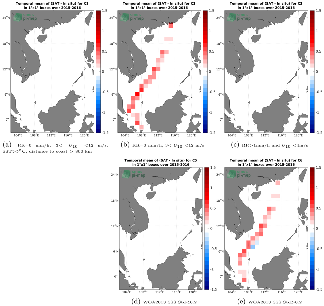
Figure 12: Temporal mean gridded over spatial boxes of size 1°×1° of \Delta SSS (SMAP SSS L3 v5.0 - 8-Day running (JPL) - TSG (LEGOS-DM)) for 5 different subdatasets corresponding to:RR=0 mm/h, 3 < U_{10} < 12 m/s, SST>5°C, distance to coast > 800 km (a), RR=0 mm/h, 3 < U_{10} < 12 m/s (b), RR>1mm/h and U_{10} < 4 m/s (c), WOA2013 SSS Std<0.2 (d), WOA2013 SSS Std>0.2 (e).
