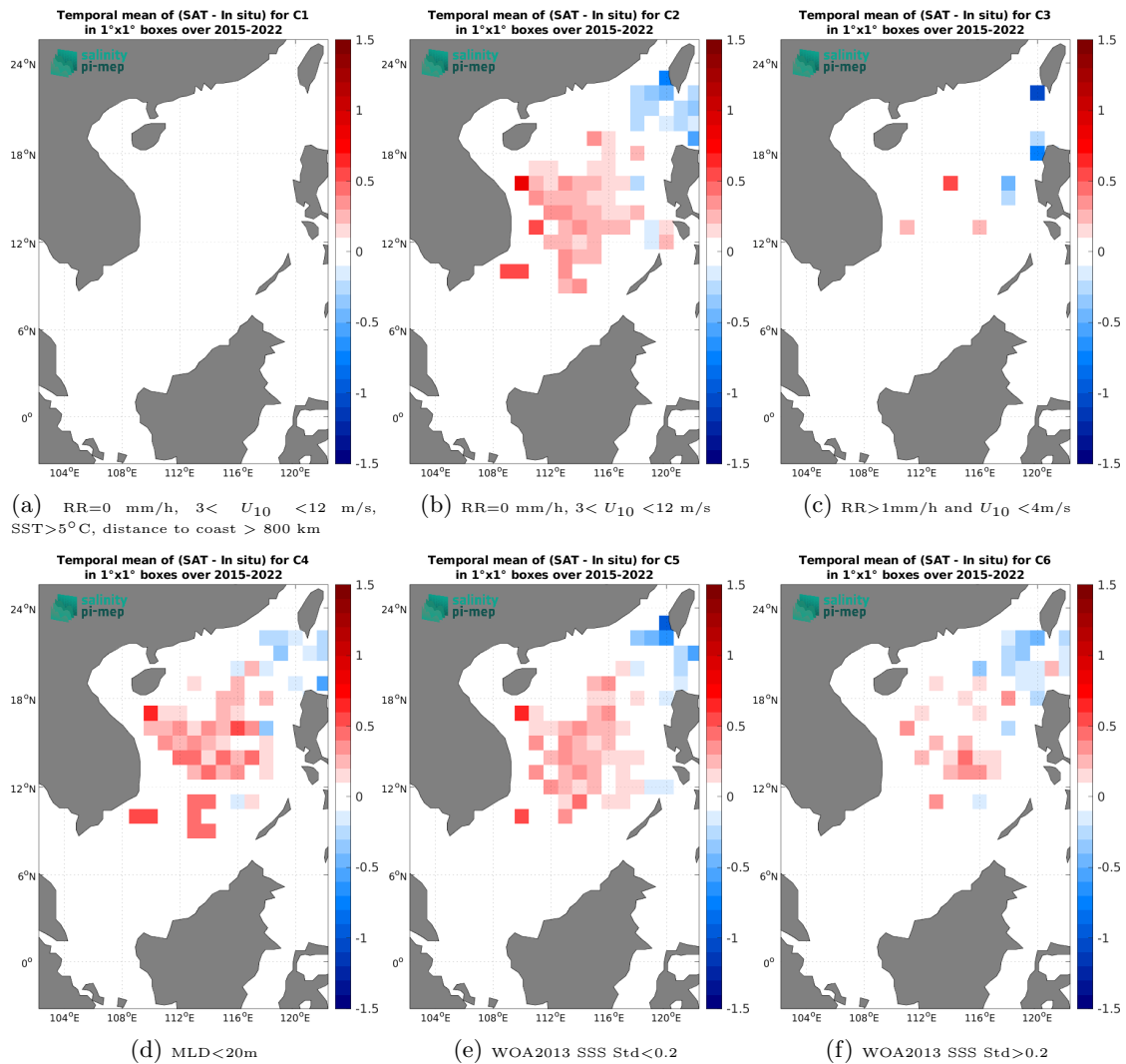
Figure 14: Temporal mean gridded over spatial boxes of size 1^\circ \times 1^\circ of \Delta\text{SSS} (SMAP SSS L3 v5.0 - 8-Day running (JPL) - Argo) for 6 different subdatasets corresponding to: RR=0 mm/h, 3 < U_{10} < 12 m/s, SST > 5^\circ\text{C} , distance to coast > 800 km (a), RR=0 mm/h, 3 < U_{10} < 12 m/s (b), RR > 1\text{mm/h} and U_{10} < 4\text{m/s} (c), MLD < 20\text{m} (d), WOA2013 SSS Std < 0.2 (e), WOA2013 SSS Std > 0.2 (f).
