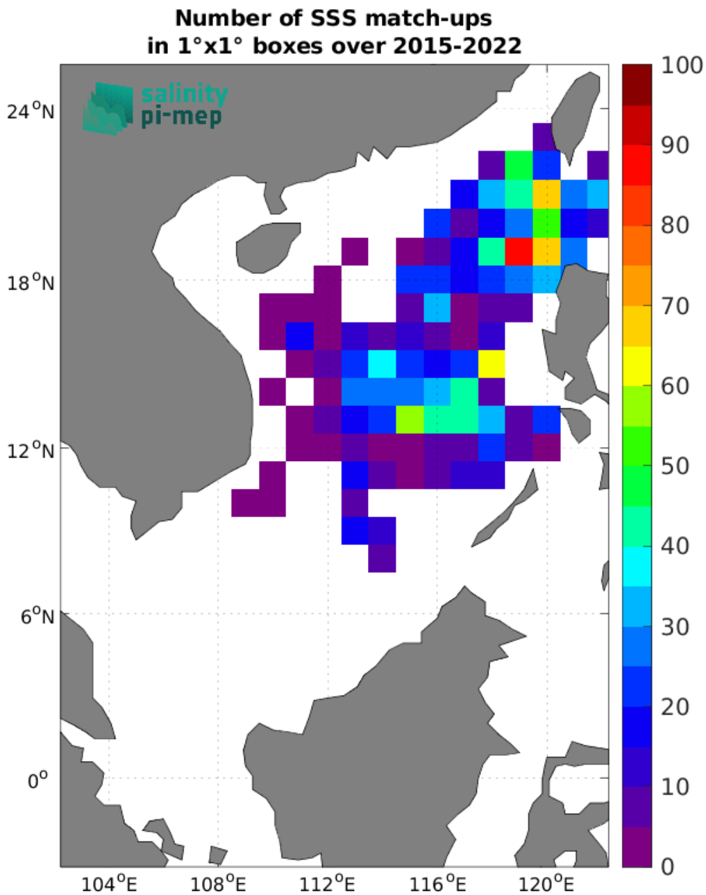
Figure 5: Number of SSS match-ups between Argo SSS and the SMAP SSS L3 v5.0 - 8-Day running (JPL) SSS product for the South China Sea Pi-MEP region over 1^\circ \times 1^\circ boxes and for the full satellite product period.
