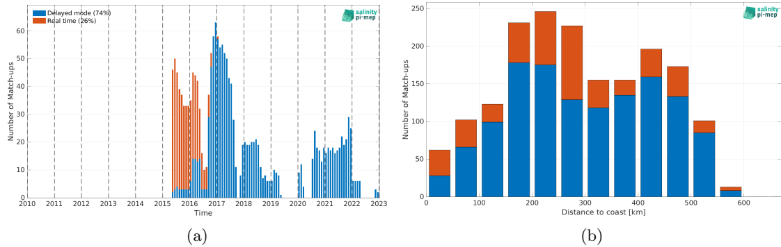
Figure 2: Number of match-ups between Argo and SMAP SSS L3 v5.0 - 8-Day running (JPL) SSS as a function of time (a) and as function of the distance to coast (b) over the South China Sea Pi-MEP region and for the full satellite product period.
