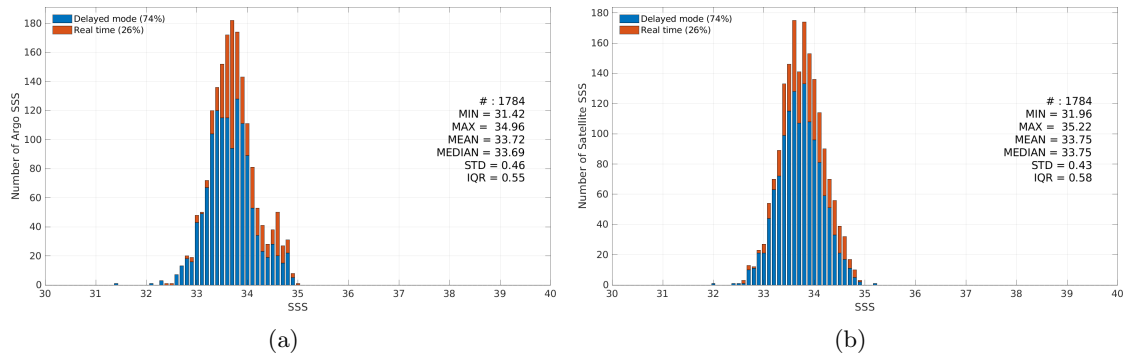
Figure 3: Histograms of SSS from Argo (a) and SMAP SSS L3 v5.0 - 8-Day running (JPL) (b) considering all match-up pairs per bins of 0.1 over the South China Sea Pi-MEP region and for the full satellite product period.
