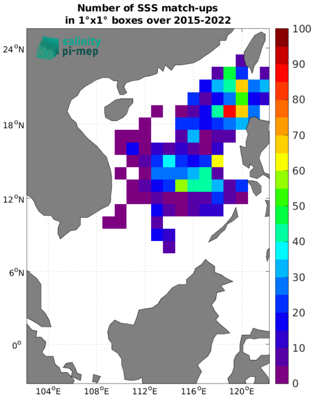
Figure 4: Number of SSS match-ups between Argo SSS and the SMAP SSS L3 v5.0 - 8-Day running (JPL) SSS product for the South China Sea Pi-MEP region over 1^{\circ} \times 1^{\circ} boxes and for the full satellite product period.
