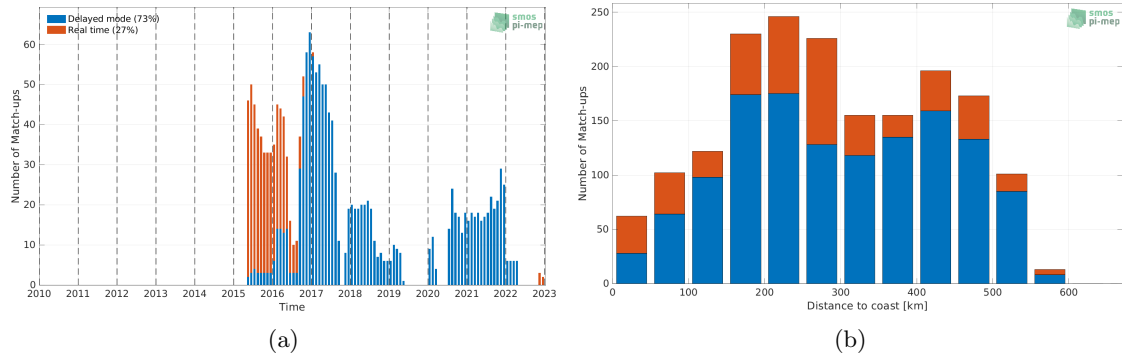
Figure 1: Number of match-ups between Argo and SMAP SSS L3 v5.0 - 8-Day running (JPL) SSS as a function of time (a) and as function of the distance to coast (b) over the South China Sea Pi-MEP region and for the full satellite product period.
