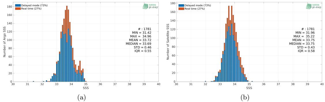
Figure 2: Histograms of SSS from Argo (a) and SMAP SSS L3 v5.0 - 8-Day running (JPL) (b) considering all match-up pairs per bins of 0.1 over the South China Sea Pi-MEP region and for the full satellite product period.
