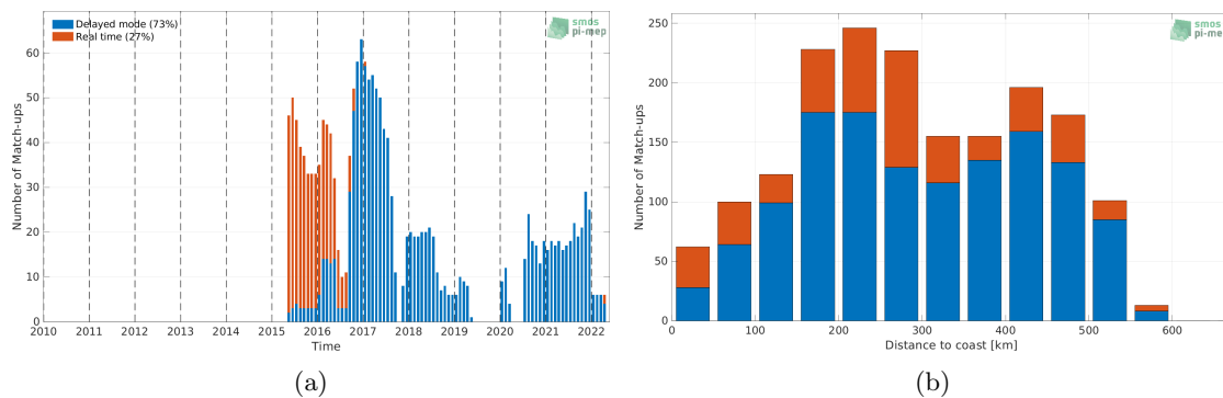
Figure 1: Number of match-ups between Argo and SMAP SSS L3 v5.0 - 8-Day running (JPL) SSS as a function of time (a) and as function of the distance to coast (b) over the South China Sea Pi-MEP region and for the full satellite product period.
