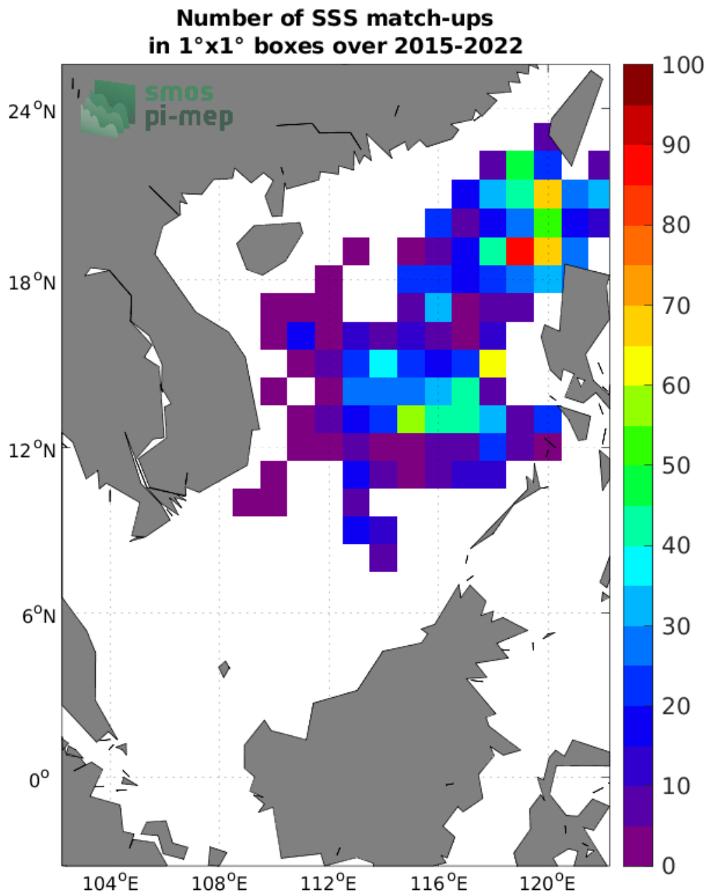
Figure 4: Number of SSS match-ups between Argo SSS and the SMAP SSS L3 v5.0 - 8-Day running (JPL) SSS product for the South China Sea Pi-MEP region over 1°x1° boxes and for the full satellite product period.
