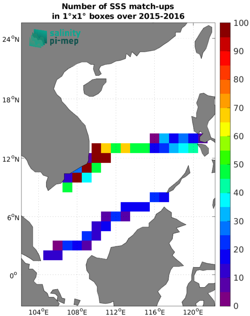
Figure 5: Number of SSS match-ups between TSG (SAMOS) SSS and the SMAP SSS L3 v5.0 - Monthly (JPL) SSS product for the South China Sea Pi-MEP region over 1^{\circ} \times 1^{\circ} boxes and for the full satellite product period.
