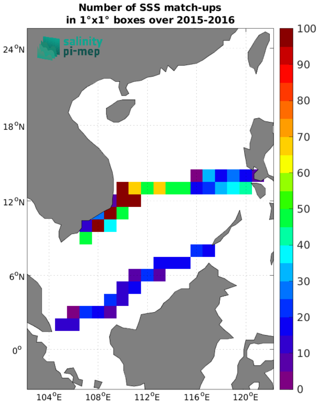
Figure 5: Number of SSS match-ups between TSG (SAMOS) SSS and the SMAP SSS L3 v5.0 - Monthly (JPL) SSS product for the South China Sea Pi-MEP region over 1^\circ \times 1^\circ boxes and for the full satellite product period.
