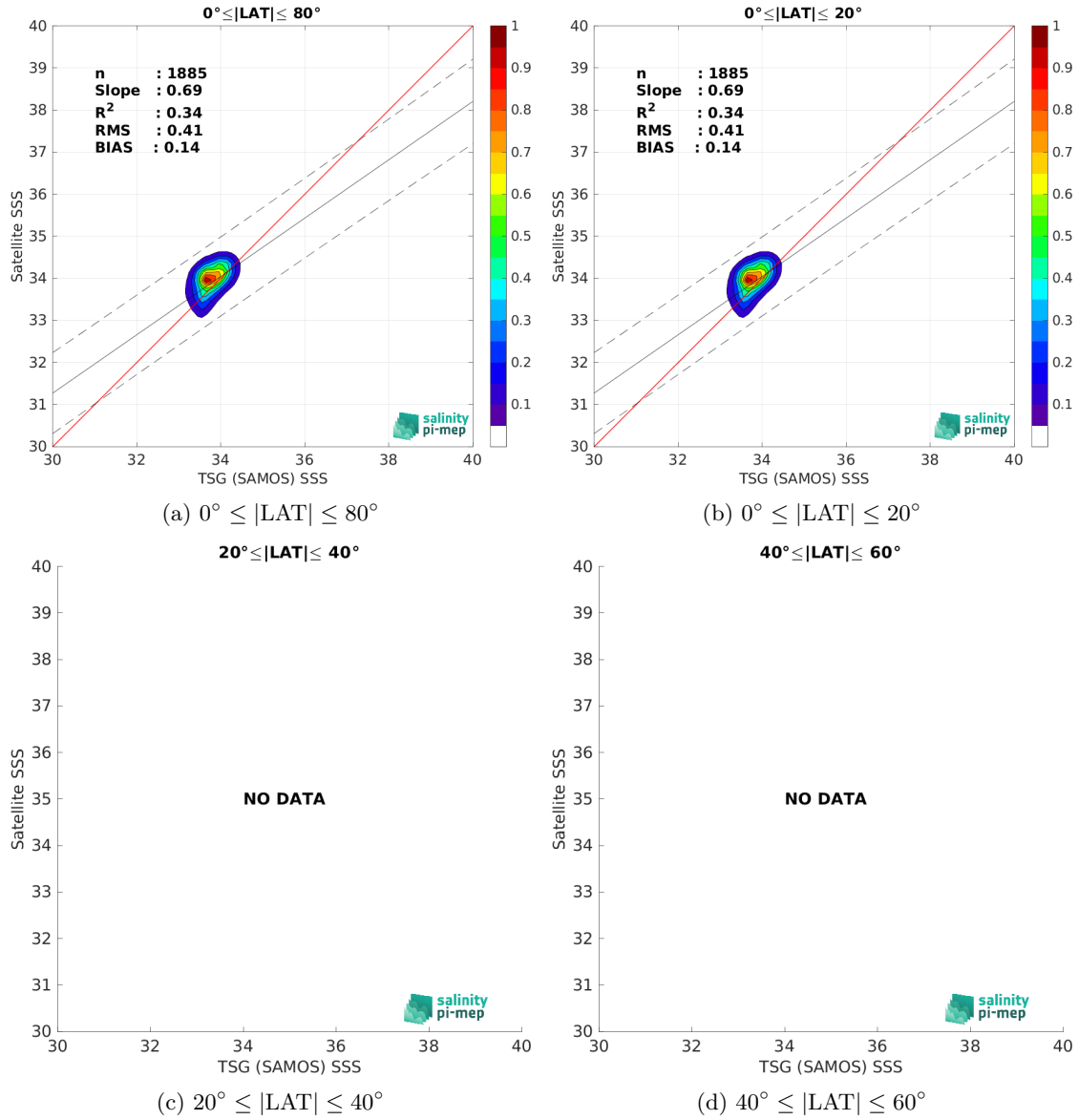
Figure 10: Contour maps of the concentration of SMAP SSS L3 v5.0 - Monthly (JPL) SSS (y-axis) versus TSG (SAMOS) SSS (x-axis) at match-up pairs for different latitude bands. For each plot, the red line shows x=y . The black thin and dashed lines indicate a linear fit through the data cloud and the \pm 95\% confidence levels, respectively. The number match-up pairs n , the slope and R^2 coefficient of the linear fit, the root mean square (RMS) and the mean bias between satellite and in situ data are indicated for each latitude band in each plots.
