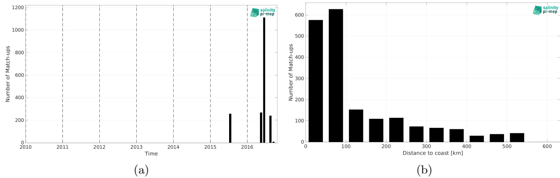
Figure 2: Number of match-ups between TSG (SAMOS) and SMAP SSS L3 v5.0 - Monthly (JPL) SSS as a function of time (a) and as function of the distance to coast (b) over the South China Sea Pi-MEP region and for the full satellite product period.
