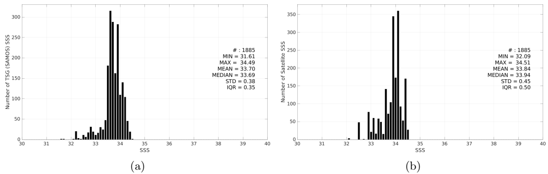
Figure 3: Histograms of SSS from TSG (SAMOS) (a) and SMAP SSS L3 v5.0 - Monthly (JPL) (b) considering all match-up pairs per bins of 0.1 over the South China Sea Pi-MEP region and for the full satellite product period.
