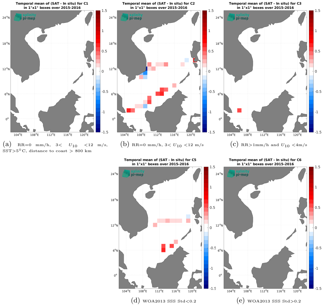
Figure 14: Temporal mean gridded over spatial boxes of size 1^\circ \times 1^\circ of \Delta SSS (SMAP SSS L3 v5.0 - Monthly (JPL) - TSG (SAMOS)) for 5 different subdatasets corresponding to: RR=0 mm/h, 3 < U_{10} < 12 m/s, SST>5°C, distance to coast > 800 km (a), RR=0 mm/h, 3 < U_{10} < 12 m/s (b), RR>1mm/h and U_{10} < 4 m/s (c), WOA2013 SSS Std<0.2 (d), WOA2013 SSS Std>0.2 (e).
