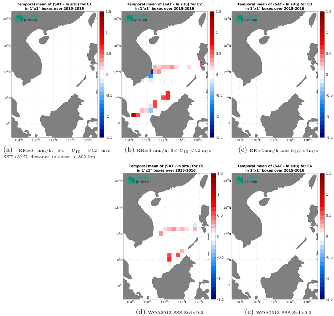
Figure 12: Temporal mean gridded over spatial boxes of size 1^\circ \times 1^\circ of \Delta\text{SSS} (SMAP SSS L3 v5.0 - Monthly (JPL) - TSG (SAMOS)) for 5 different subdatasets corresponding to:RR=0 mm/h, 3 < U_{10} < 12 m/s, SST >5^\circ\text{C} , distance to coast > 800 km (a), RR=0 mm/h, 3 < U_{10} < 12 m/s (b), RR >1 mm/h and U_{10} < 4 m/s (c), WOA2013 SSS Std <0.2 (d), WOA2013 SSS Std >0.2 (e).
