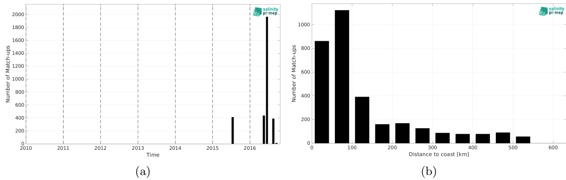
Figure 1: Number of match-ups between TSG (SAMOS) and SMAP SSS L3 v5.0 - Monthly (JPL) SSS as a function of time (a) and as function of the distance to coast (b) over the South China Sea Pi-MEP region and for the full satellite product period.
