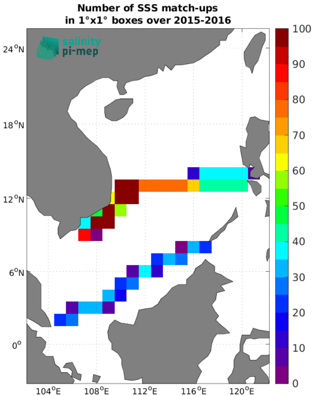
Figure 4: Number of SSS match-ups between TSG (SAMOS) SSS and the SMAP SSS L3 v5.0 - Monthly (JPL) SSS product for the South China Sea Pi-MEP region over 1^{\circ} \times 1^{\circ} boxes and for the full satellite product period.
