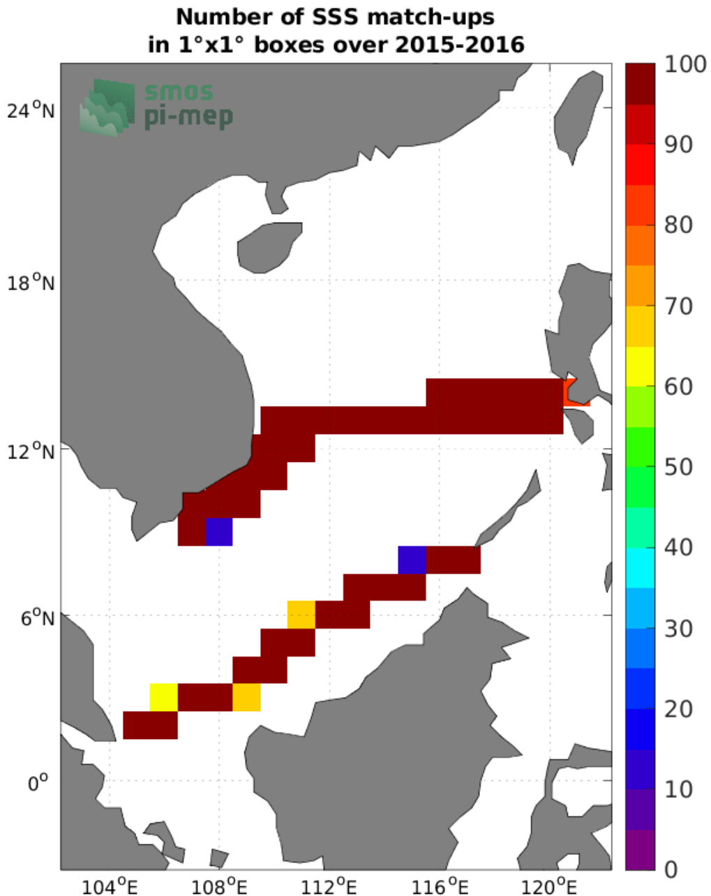
Figure 4: Number of SSS match-ups between TSG (SAMOS) SSS and the SMAP SSS L3 v5.0 - Monthly (JPL) SSS product for the South China Sea Pi-MEP region over 1°x1° boxes and for the full satellite product period.
