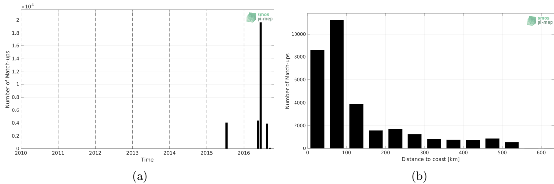
Figure 1: Number of match-ups between TSG (SAMOS) and SMAP SSS L3 v5.0 - Monthly (JPL) SSS as a function of time (a) and as function of the distance to coast (b) over the South China Sea Pi-MEP region and for the full satellite product period.
