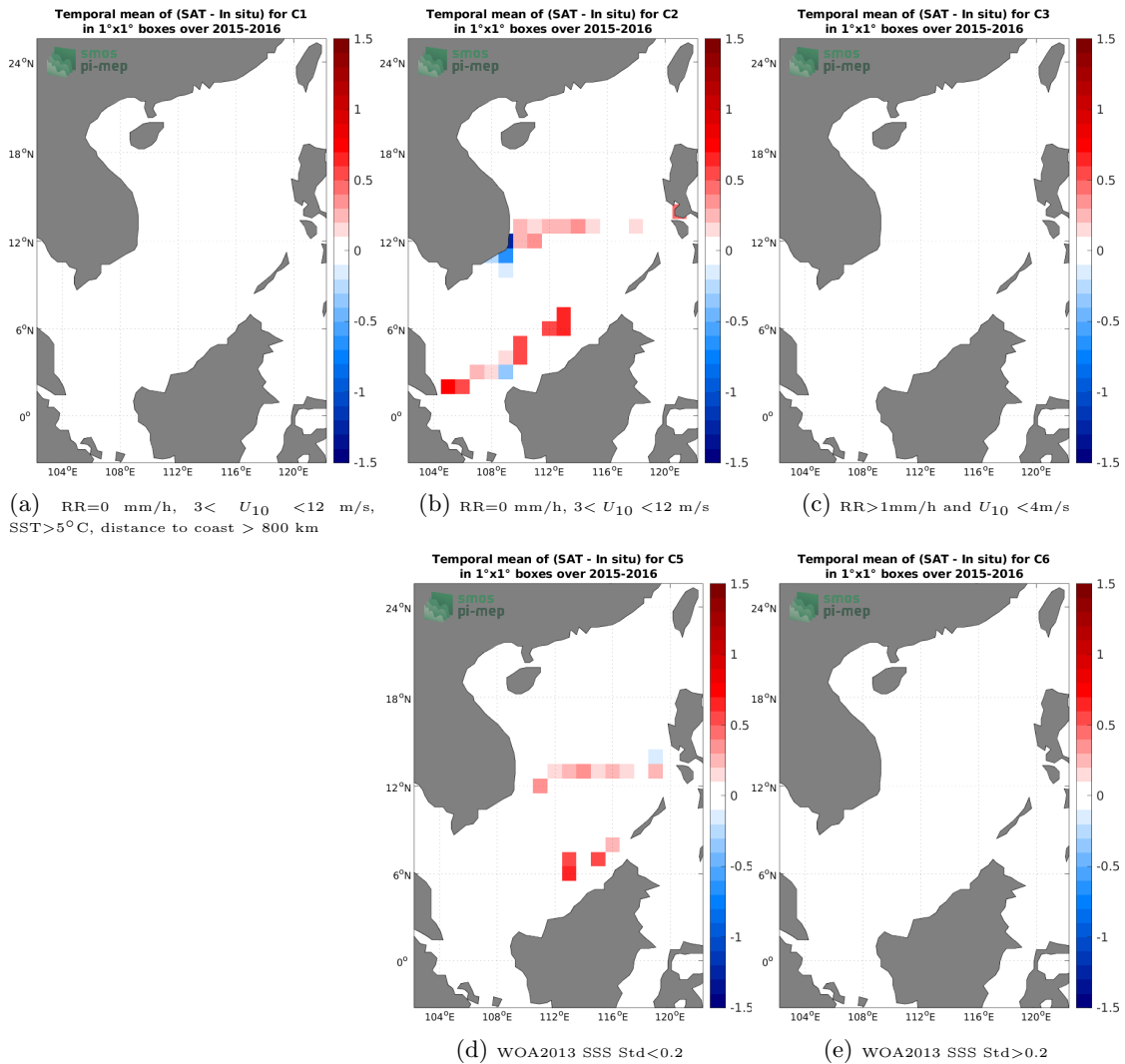
Figure 12: Temporal mean gridded over spatial boxes of size 1^\circ \times 1^\circ of \Delta SSS (SMAP SSS L3 v5.0 - Monthly (JPL) - TSG (SAMOS)) for 5 different subdatasets corresponding to:RR=0 mm/h, 3 < U_{10} < 12 m/s, SST>5°C, distance to coast > 800 km (a), RR=0 mm/h, 3 < U_{10} < 12 m/s (b), RR>1mm/h and U_{10} < 4 m/s (c), WOA2013 SSS Std<0.2 (d), WOA2013 SSS Std>0.2 (e).
