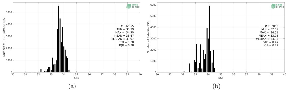
Figure 2: Histograms of SSS from TSG (SAMOS) (a) and SMAP SSS L3 v5.0 - Monthly (JPL) (b) considering all match-up pairs per bins of 0.1 over the South China Sea Pi-MEP region and for the full satellite product period.
