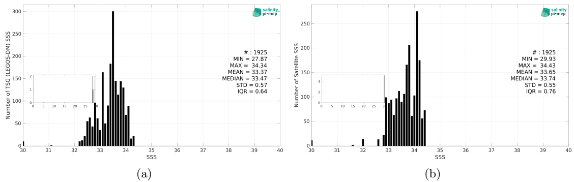
Figure 3: Histograms of SSS from TSG (LEGOS-DM) (a) and SMAP SSS L3 v5.0 - Monthly (JPL) (b) considering all match-up pairs per bins of 0.1 over the South China Sea Pi-MEP region and for the full satellite product period.
