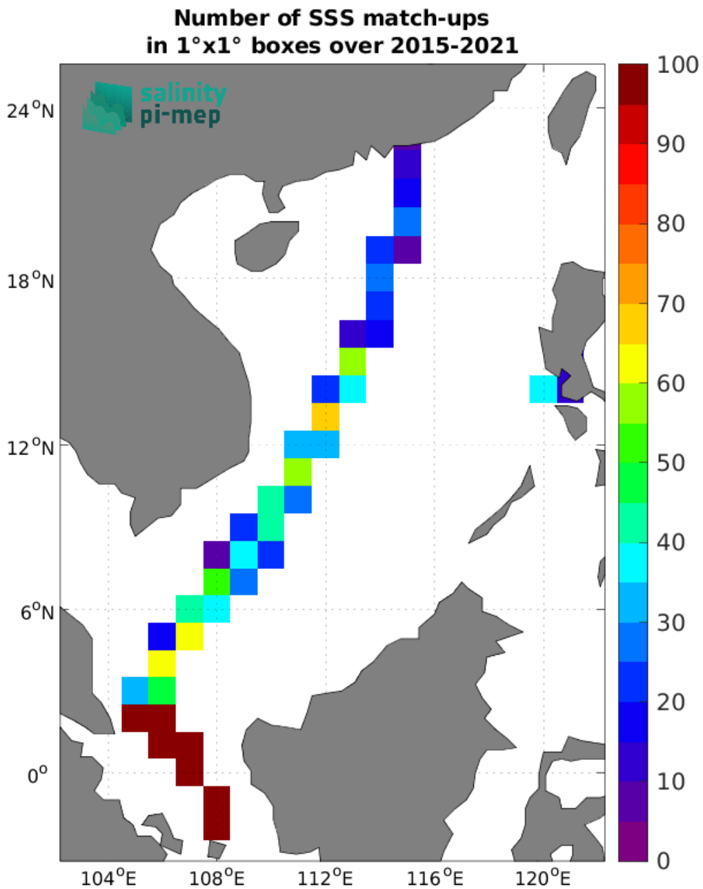
Figure 5: Number of SSS match-ups between TSG (LEGOS-DM) SSS and the SMAP SSS L3 v5.0 - Monthly (JPL) SSS product for the South China Sea Pi-MEP region over 1°x1° boxes and for the full satellite product period.
