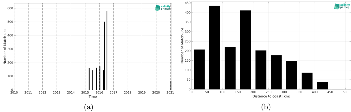
Figure 2: Number of match-ups between TSG (LEGOS-DM) and SMAP SSS L3 v5.0 - Monthly (JPL) SSS as a function of time (a) and as function of the distance to coast (b) over the South China Sea Pi-MEP region and for the full satellite product period.
