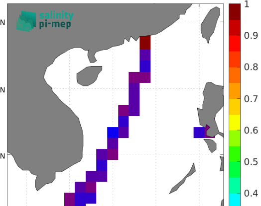
Temporal STD of (Sat - TSG (LEGOS-DM)) in 1°x1° boxes over 2015-2021
