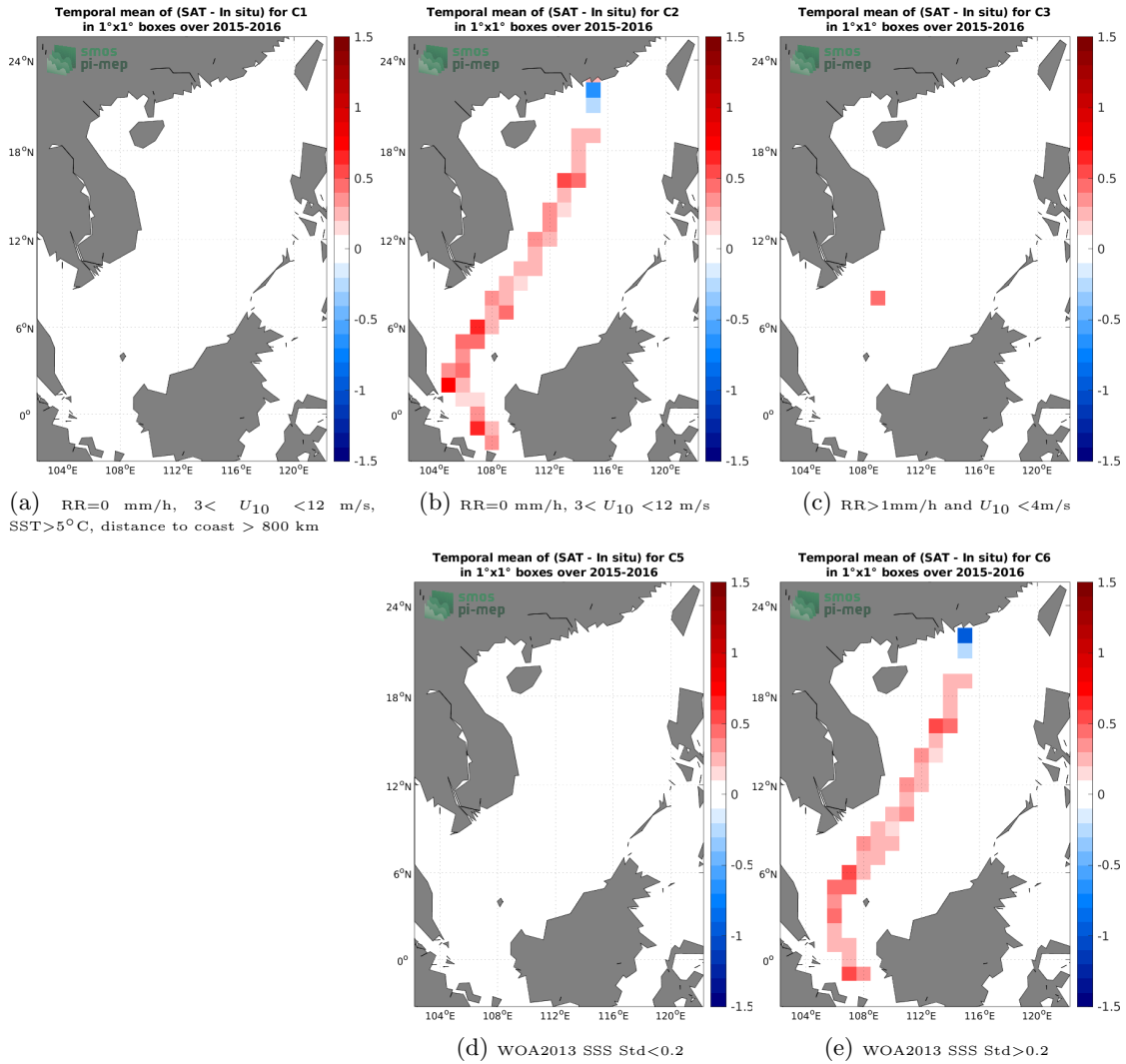
Figure 12: Temporal mean gridded over spatial boxes of size 1^\circ \times 1^\circ of \Delta SSS (SMAP SSS L3 v5.0 - Monthly (JPL) - TSG (LEGOS-DM)) for 5 different subdatasets corresponding to: RR=0 mm/h, 3 < U_{10} < 12 m/s, SST>5°C, distance to coast > 800 km (a), RR=0 mm/h, 3 < U_{10} < 12 m/s (b), RR>1mm/h and U_{10} < 4 m/s (c), WOA2013 SSS Std<0.2 (d), WOA2013 SSS Std>0.2 (e).
