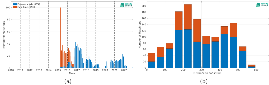
Figure 2: Number of match-ups between Argo and SMAP SSS L3 v5.0 - Monthly (JPL) SSS as a function of time (a) and as function of the distance to coast (b) over the South China Sea Pi-MEP region and for the full satellite product period.
