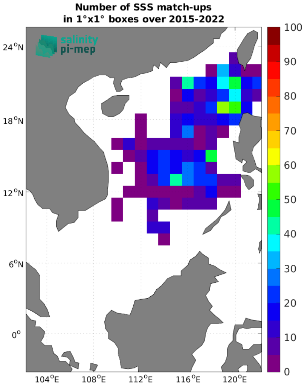
Figure 5: Number of SSS match-ups between Argo SSS and the SMAP SSS L3 v5.0 - Monthly (JPL) SSS product for the South China Sea Pi-MEP region over 1^{\circ} \times 1^{\circ} boxes and for the full satellite product period.
