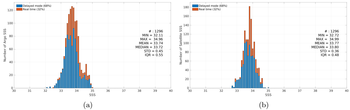
Figure 3: Histograms of SSS from Argo (a) and SMAP SSS L3 v5.0 - Monthly (JPL) (b) considering all match-up pairs per bins of 0.1 over the South China Sea Pi-MEP region and for the full satellite product period.
