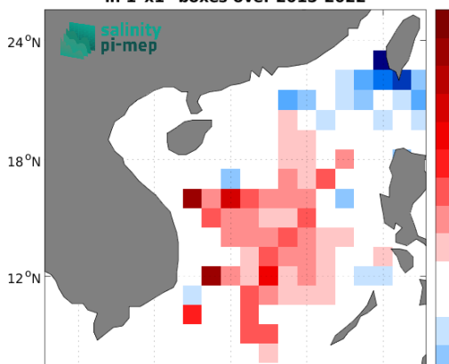
Temporal mean of (Sat - Argo) in 1°x1° boxes over 2015-2022
