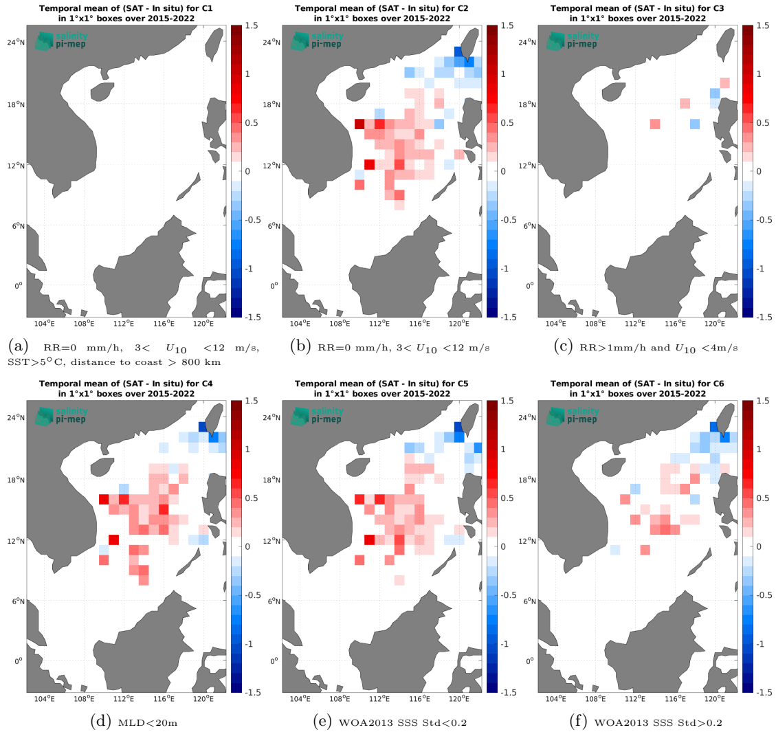
Figure 14: Temporal mean gridded over spatial boxes of size 1^\circ \times 1^\circ of \Delta\text{SSS} (SMAP SSS L3 v5.0 - Monthly (JPL) - Argo) for 6 different subdatasets corresponding to: RR=0 mm/h, 3 < U_{10} < 12 m/s, SST > 5^\circ\text{C} , distance to coast > 800 km (a), RR=0 mm/h, 3 < U_{10} < 12 m/s (b), RR > 1 mm/h and U_{10} < 4 m/s (c), MLD < 20 m (d), WOA2013 SSS Std < 0.2 (e), WOA2013 SSS Std > 0.2 (f).
