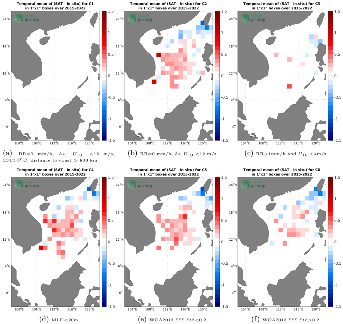
Figure 12: Temporal mean gridded over spatial boxes of size 1^\circ \times 1^\circ of \Delta SSS (SMAP SSS L3 v5.0 - Monthly (JPL) - Argo) for 6 different subdatasets corresponding to:RR=0 mm/h, 3 < U_{10} < 12 m/s, SST>5°C, distance to coast > 800 km (a), RR=0 mm/h, 3 < U_{10} < 12 m/s (b), RR>1mm/h and U_{10} < 4 m/s (c),MLD<20m (d),WOA2013 SSS Std<0.2 (e),WOA2013 SSS Std>0.2 (f).
