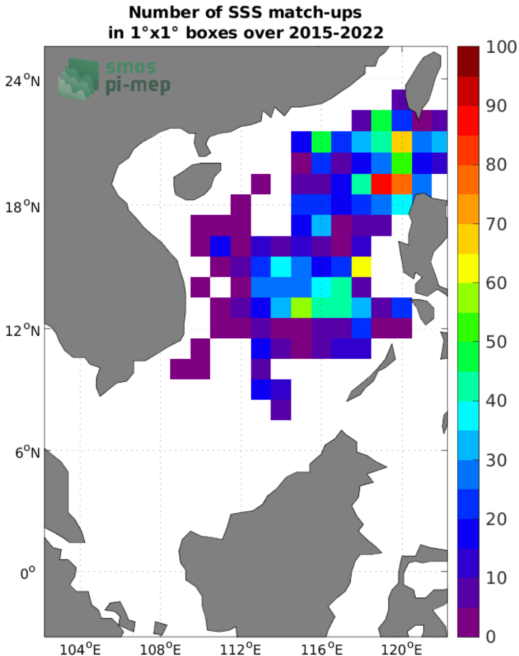
Figure 4: Number of SSS match-ups between Argo SSS and the SMAP SSS L3 v5.0 - Monthly (JPL) SSS product for the South China Sea Pi-MEP region over 1°×1° boxes and for the full satellite product period.
