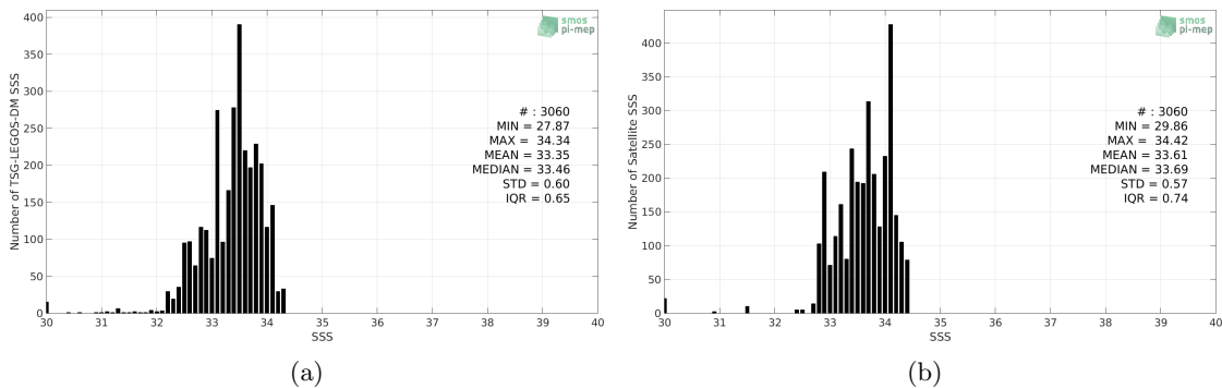
Figure 2: Histograms of SSS from TSG-LEGOS-DM (a) and SMAP-L3-JPL-V4.3-MONTHLY-60KM (b) considering all match-up pairs per bins of 0.1 over the South China Sea Pi-MEP region and for the full satellite product period.
