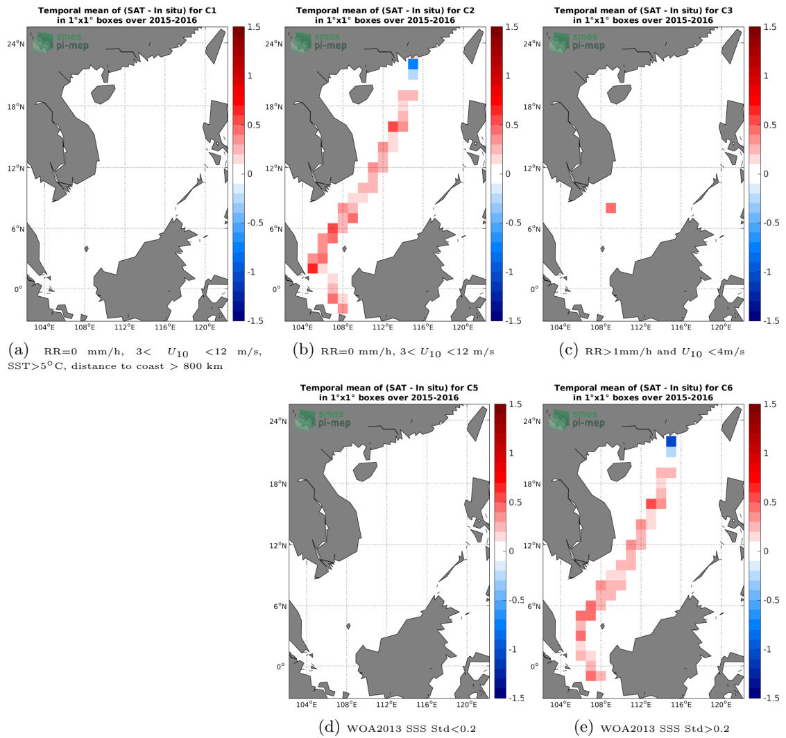
Figure 12: Temporal mean gridded over spatial boxes of size 1°x1° of \Delta SSS (SMAP-L3-JPL-V4.3-MONTHLY-60KM - TSG-LEGOS-DM) for 5 different subdatasets corresponding to:RR=0 mm/h, 3 < U_{10} < 12 m/s, SST>5°C, distance to coast > 800 km (a), RR=0 mm/h, 3 < U_{10} < 12 m/s (b), RR>1mm/h and U_{10} < 4 m/s (c), WOA2013 SSS Std<0.2 (d), WOA2013 SSS Std>0.2 (e).
