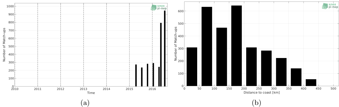
Figure 1: Number of match-ups between TSG-LEGOS-DM and SMAP-L3-JPL-V4.3-MONTHLY-60KM SSS as a function of time (a) and as function of the distance to coast (b) over the South China Sea Pi-MEP region and for the full satellite product period.
