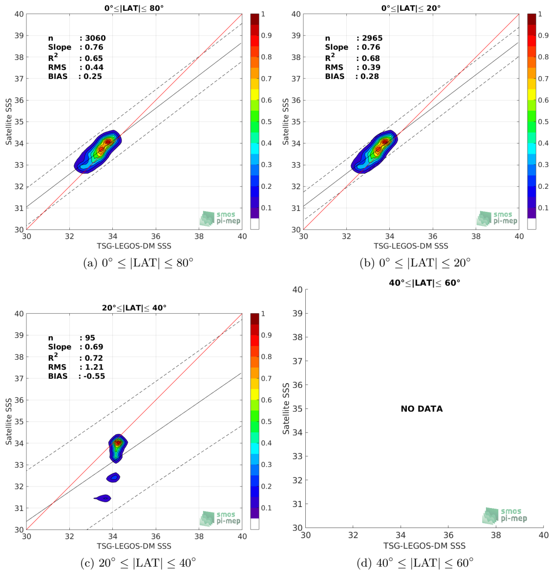
Figure 9: Contour maps of the concentration of SMAP-L3-JPL-V4.3-MONTHLY-60KM SSS (y-axis) versus TSG-LEGOS-DM SSS (x-axis) at match-up pairs for different latitudinal bands. For each plot, the red line shows x=y . The black thin and dashed lines indicate a linear fit through the data cloud and the \pm 95\% confidence levels, respectively. The number match-up pairs n , the slope and R^2 coefficient of the linear fit, the root mean square (RMS) and the mean bias between satellite and in situ data are indicated for each latitude band in each plots.
