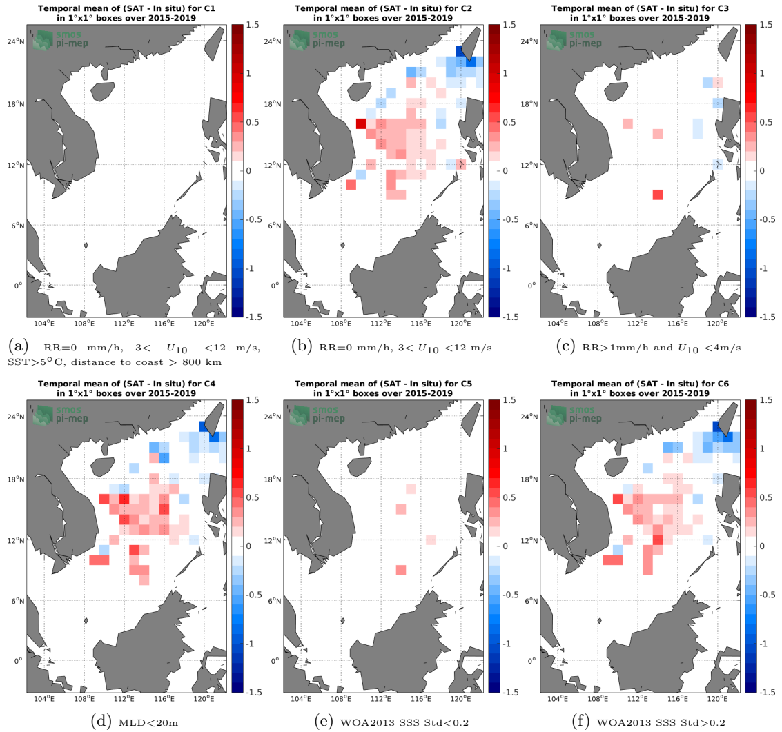
Figure 12: Temporal mean gridded over spatial boxes of size 1^\circ \times 1^\circ of \Delta SSS (SMAP-L3-JPL-V4.3-MONTHLY-60KM - Argo) for 6 different subdatasets corresponding to:RR=0 mm/h, 3 < U_{10} < 12 m/s, SST>5°C, distance to coast > 800 km (a), RR=0 mm/h, 3 < U_{10} < 12 m/s (b), RR>1mm/h and U_{10} < 4 m/s (c),MLD<20m (d),WOA2013 SSS Std<0.2 (e),WOA2013 SSS Std>0.2 (f).
