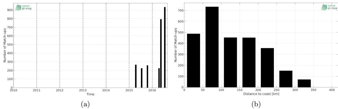
Figure 1: Number of match-ups between TSG-LEGOS-DM and SMAP-L3-JPL-V4-8DAY-RUNNING-60KM SSS as a function of time (a) and as function of the distance to coast (b) over the South China Sea Pi-MEP region and for the full satellite product period.
