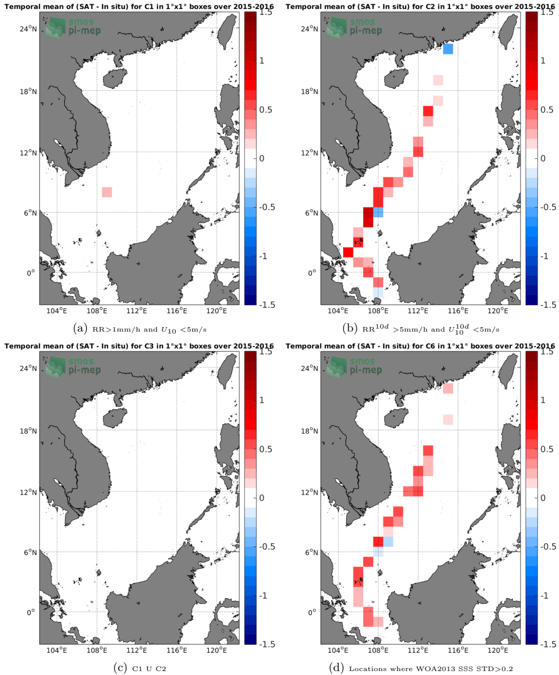
Figure 12: Temporal mean gridded over spatial boxes of size 1°x1° of \Delta\text{SSS} (SMAP-L3-JPL-V4-8DAY-RUNNING-60KM - TSG-LEGOS-DM) for 4 different subdatasets corresponding to: RR > 1\text{mm/h} and U_{10} < 5\text{m/s} (a), RR^{10d} > 5\text{mm/h} and U_{10}^{10d} < 5\text{m/s} (b), C1 U C2 (c), Locations where WOA2013 SSS STD > 0.2 (d).
