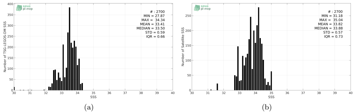
Figure 2: Histograms of SSS from TSG-LEGOS-DM (a) and SMAP-L3-JPL-V4-8DAY-RUNNING-60KM (b) considering all match-up pairs per bins of 0.1 over the South China Sea Pi-MEP region and for the full satellite product period.
