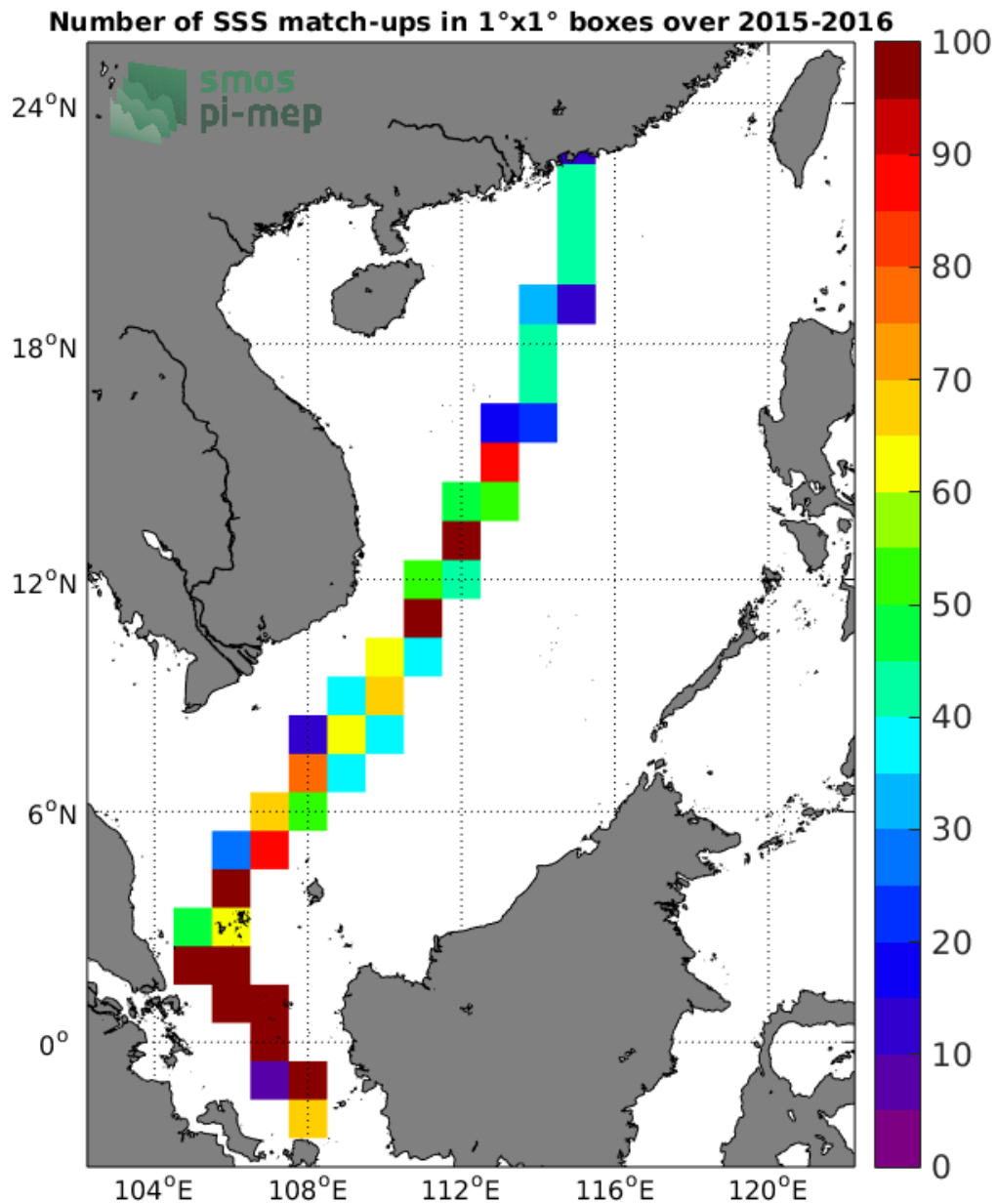
Figure 4: Number of SSS match-ups between TSG-LEGOS-DM SSS and the SMAP-L3-JPL-V4-8DAY-RUNNING-60KM SSS product for the South China Sea Pi-MEP region over 1°x1° boxes and for the full satellite product period.
