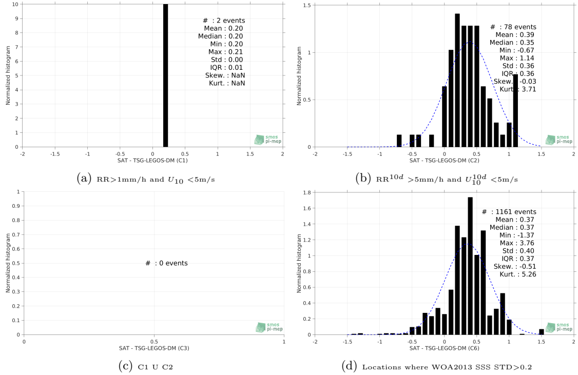
Figure 13: Normalized histogram of \Delta\text{SSS} (SMAP-L3-JPL-V4-8DAY-RUNNING-60KM - TSG-LEGOS-DM) for 6 different subdatasets corresponding to: RR > 1mm/h and U_{10} < 5\text{m/s} (a), RR^{10d} > 5\text{mm/h} and U_{10}^{10d} < 5\text{m/s} (b), C1 U C2 (c), Locations where WOA2013 SSS STD > 0.2 (d).
