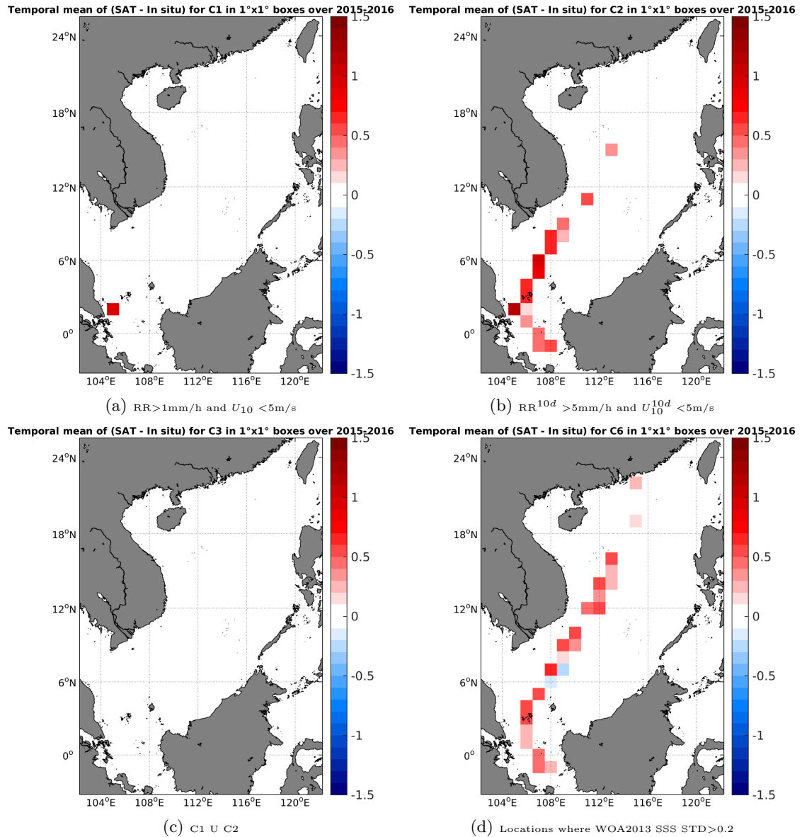
Figure 12: Temporal mean gridded over spatial boxes of size 1^\circ \times 1^\circ of \Delta SSS (SMAP-L3-JPL-V4-8DAY-RUNNING-60KM - TSG-LEGOS-DM) for 4 different subdatasets corresponding to: RR > 1 mm/h and U_{10} < 5 m/s (a), RR 10d > 5 mm/h and U_{10}^{10d} < 5 m/s (b), C1 U C2 (c), Locations where WOA2013 SSS STD > 0.2 (d).
