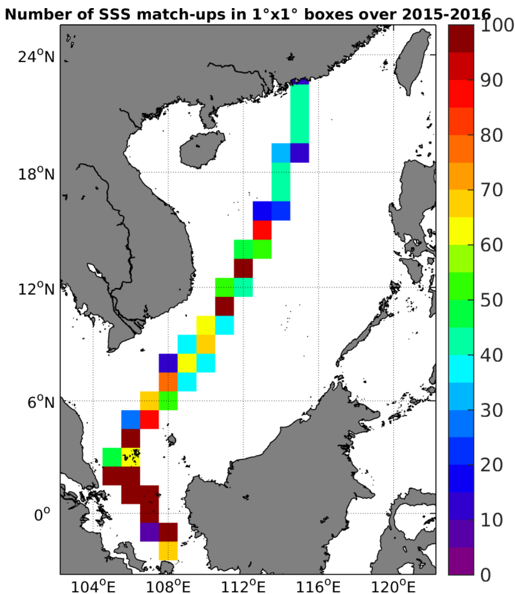
Figure 4: Number of SSS match-ups between TSG-LEGOS-DM SSS and the SMAP-L3-JPL-V4-8DAY-RUNNING-60KM SSS product for the South China Sea Pi-MEP region over 1°x1° boxes and for the full satellite product period.
