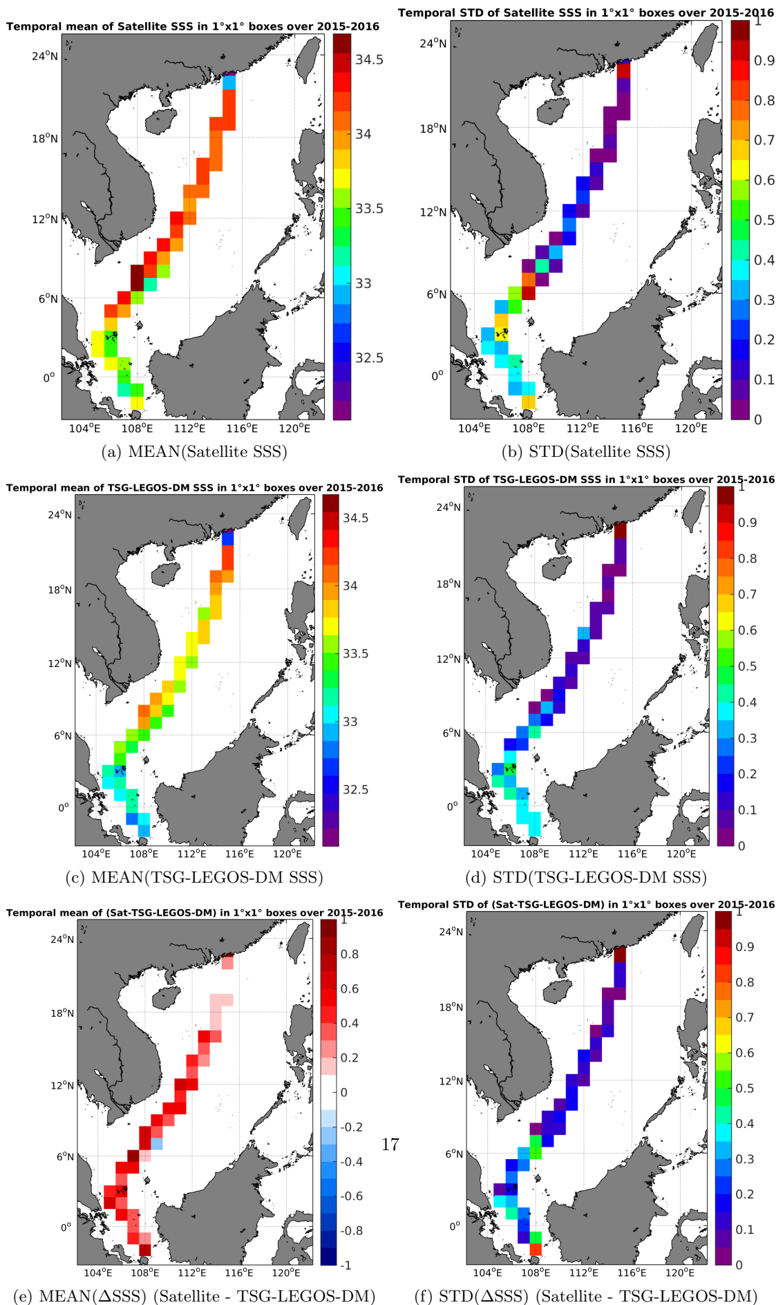
Figure 6: Temporal mean (left) and STD (right) of SSS from SMAP-L3-JPL-V4-8DAY-RUNNING-60KM (top), TSG-LEGOS-DM (middle), and of \Delta SSS (Satellite - TSG-LEGOS-DM). Only match-up pairs are used to generate these maps.
