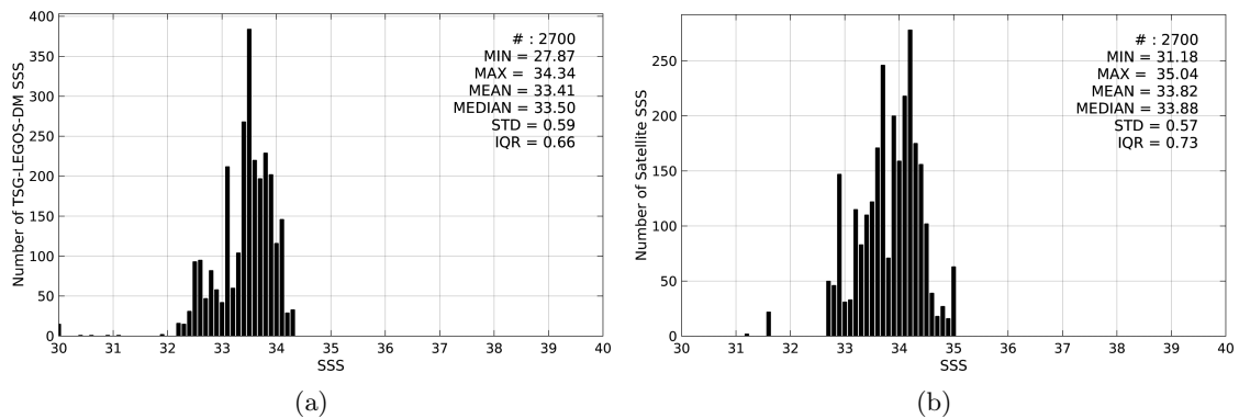
Figure 2: Histograms of SSS from TSG-LEGOS-DM (a) and SMAP-L3-JPL-V4-8DAY-RUNNING-60KM (b) considering all match-up pairs per bins of 0.1 over the South China Sea Pi-MEP region and for the full satellite product period.
