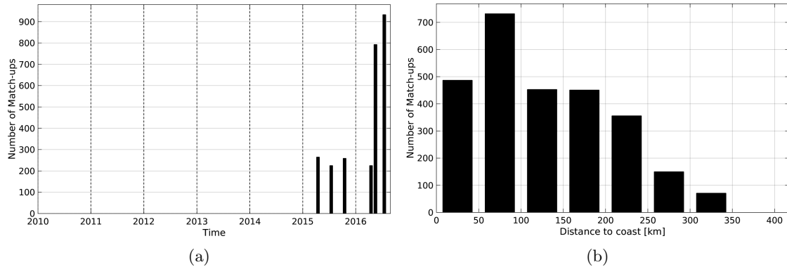
Figure 1: Number of match-ups between TSG-LEGOS-DM and SMAP-L3-JPL-V4-8DAY-RUNNING-60KM SSS as a function of time (a) and as function of the distance to coast (b) over the South China Sea Pi-MEP region and for the full satellite product period.
