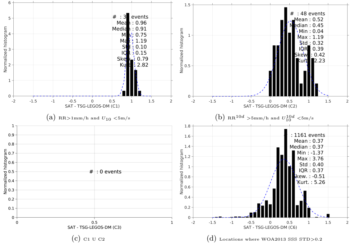
Figure 13: Normalized histogram of \Delta SSS (SMAP-L3-JPL-V4-8DAY-RUNNING-60KM - TSG-LEGOS-DM) for 6 different subdatasets corresponding to: RR > 1mm/h and U_{10} < 5 m/s (a), RR^{10d} > 5 mm/h and U_{10}^{10d} < 5 m/s (b), C1 U C2 (c), Locations where WOA2013 SSS STD > 0.2 (d).
