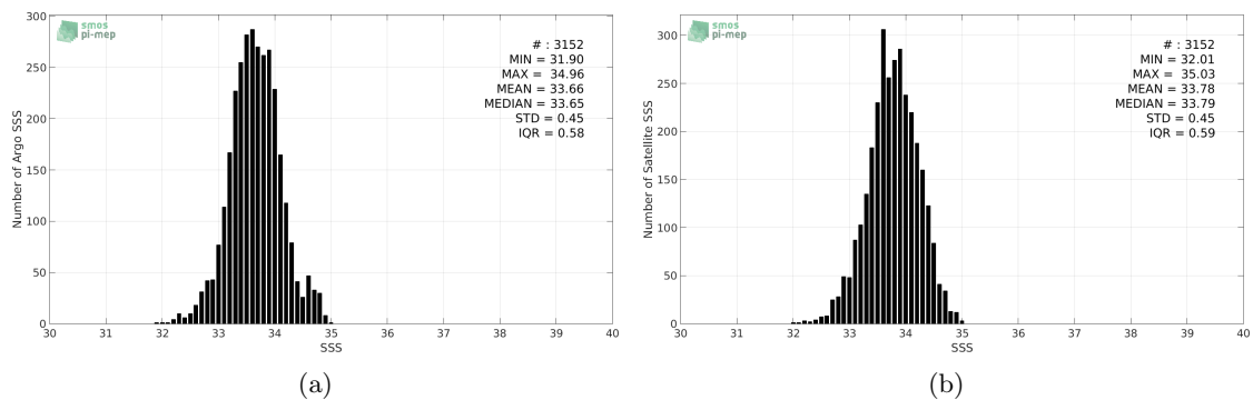
Figure 2: Histograms of SSS from Argo (a) and SMAP-L3-JPL-V4-8DAY-RUNNING-60KM (b) considering all match-up pairs per bins of 0.1 over the South China Sea Pi-MEP region and for the full satellite product period.
