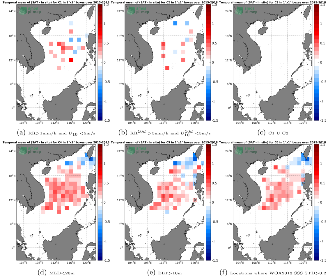
Figure 12: Temporal mean gridded over spatial boxes of size 1°x1° of \Delta SSS (SMAP-L3-JPL-V4-8DAY-RUNNING-60KM - Argo) for 6 different subdatasets corresponding to: RR > 1\text{mm/h} and U_{10} < 5\text{m/s} (a), RR^{10d} > 5\text{mm/h} and U_{10}^{10d} < 5\text{m/s} (b), C1 U C2 (c), MLD < 20\text{m} (d), BLT > 10\text{m} (e), Locations where WOA2013 SSS STD > 0.2 (f).
