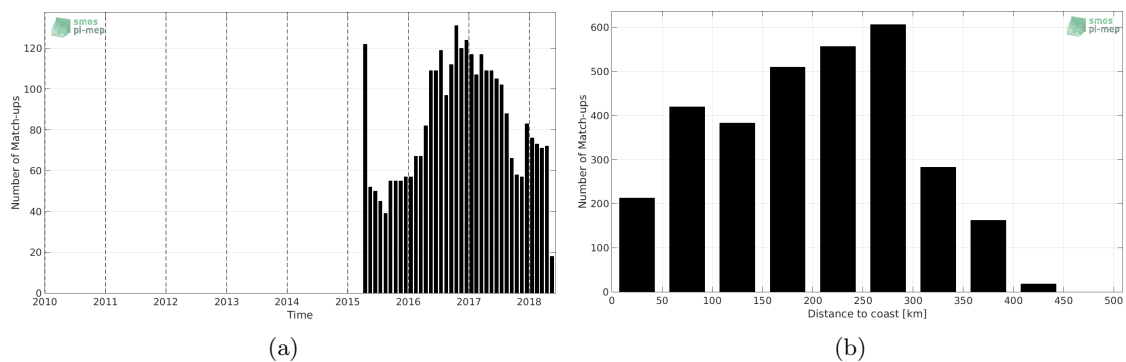
Figure 1: Number of match-ups between Argo and SMAP-L3-JPL-V4-8DAY-RUNNING-60KM SSS as a function of time (a) and as function of the distance to coast (b) over the South China Sea Pi-MEP region and for the full satellite product period.
