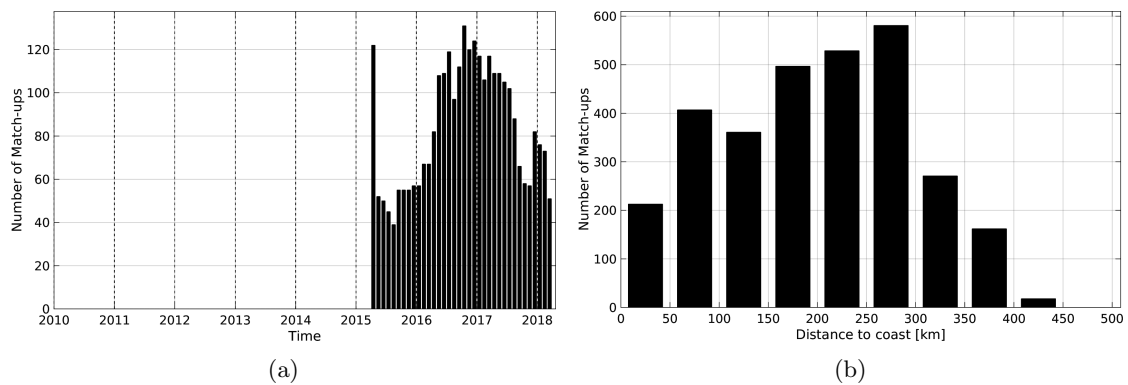
Figure 1: Number of match-ups between Argo and SMAP-L3-JPL-V4-8DAY-RUNNING-60KM SSS as a function of time (a) and as function of the distance to coast (b) over the South China Sea Pi-MEP region and for the full satellite product period.
