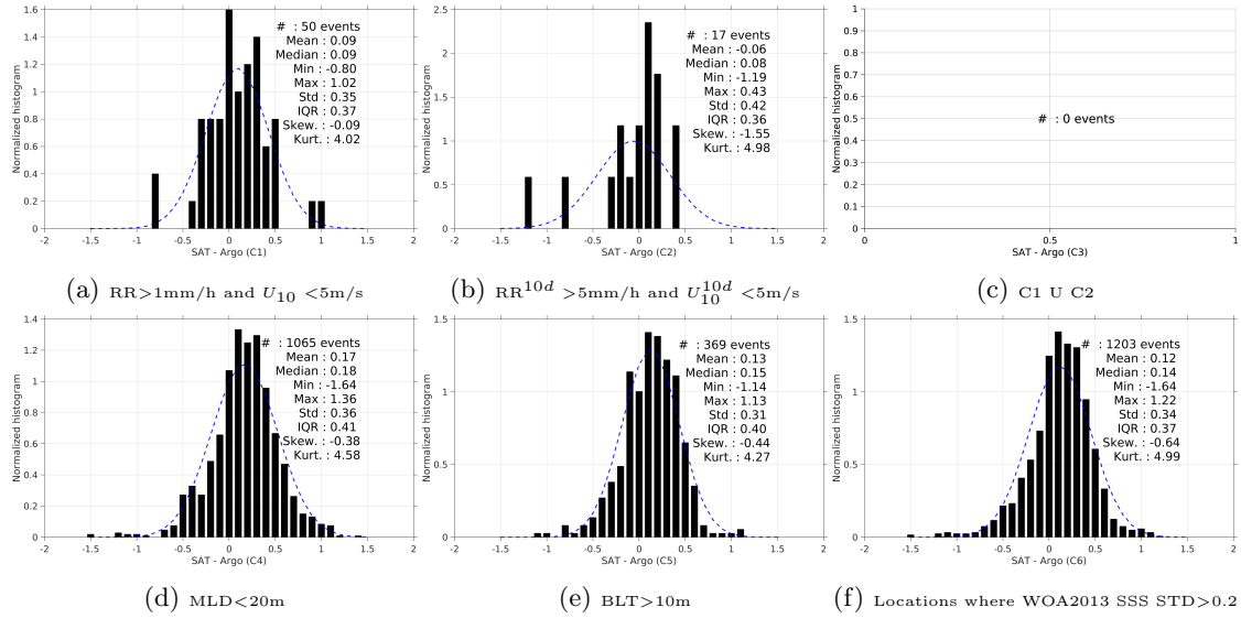
Figure 13: Normalized histogram of \Delta SSS (SMAP-L3-JPL-V4-8DAY-RUNNING-60KM - Argo) for 6 different subdatasets corresponding to: RR > 1mm/h and U_{10} < 5 m/s (a), RR^{10d} > 5 mm/h and U_{10}^{10d} < 5 m/s (b), C1 U C2 (c), MLD < 20m (d), BLT > 10m (e), Locations where WOA2013 SSS STD > 0.2 (f).
