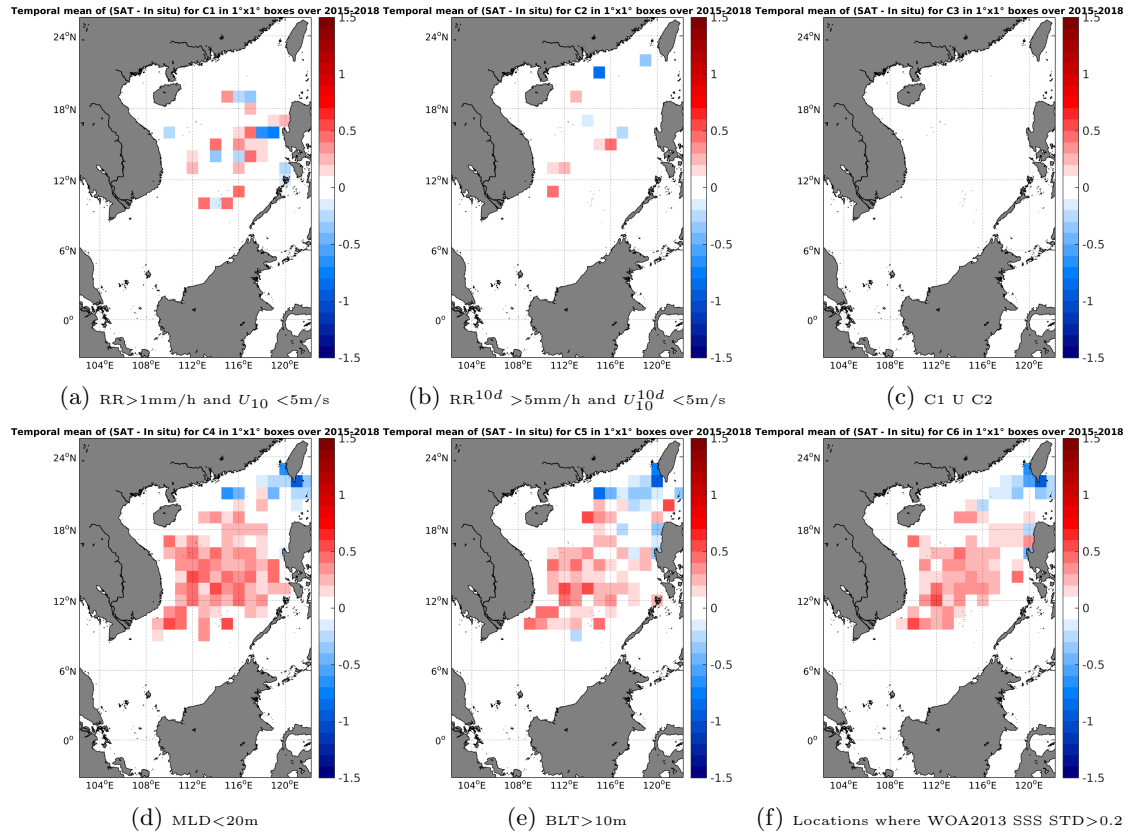
Figure 12: Temporal mean gridded over spatial boxes of size 1^\circ \times 1^\circ of \Delta SSS (SMAP-L3-JPL-V4-8DAY-RUNNING-60KM - Argo) for 6 different subdatasets corresponding to: RR > 1\text{mm/h} and U_{10} < 5\text{m/s} (a), RR^{10d} > 5\text{mm/h} and U_{10}^{10d} < 5\text{m/s} (b), C1 U C2 (c), MLD < 20\text{m} (d), BLT > 10\text{m} (e), Locations where WOA2013 SSS STD > 0.2 (f).
