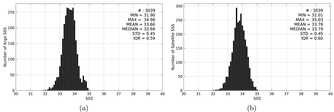
Figure 2: Histograms of SSS from Argo (a) and SMAP-L3-JPL-V4-8DAY-RUNNING-60KM (b) considering all match-up pairs per bins of 0.1 over the South China Sea Pi-MEP region and for the full satellite product period.
