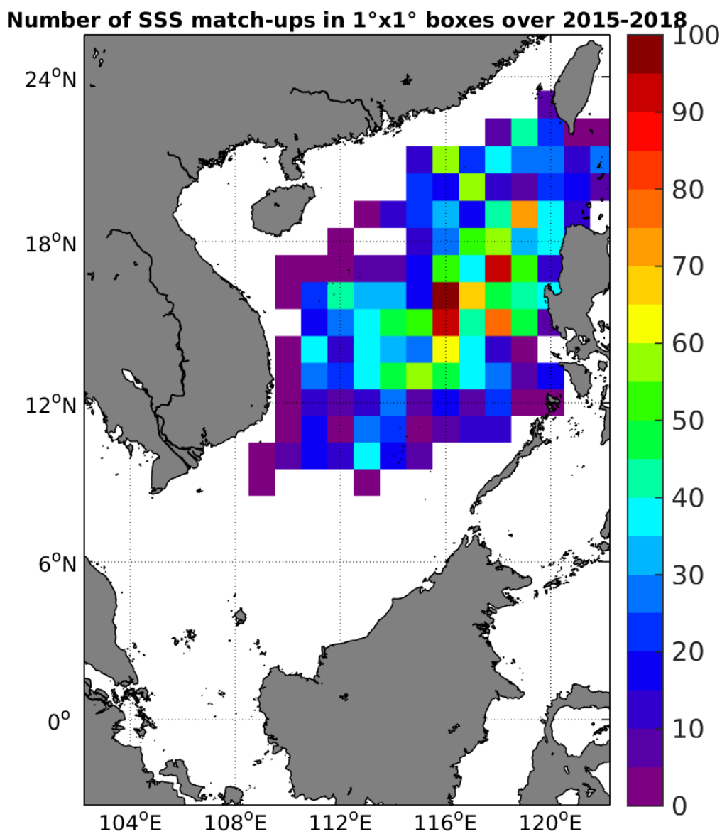
Figure 4: Number of SSS match-ups between Argo SSS and the SMAP-L3-JPL-V4-8DAY-RUNNING-60KM SSS product for the South China Sea Pi-MEP region over 1°x1° boxes and for the full satellite product period.
