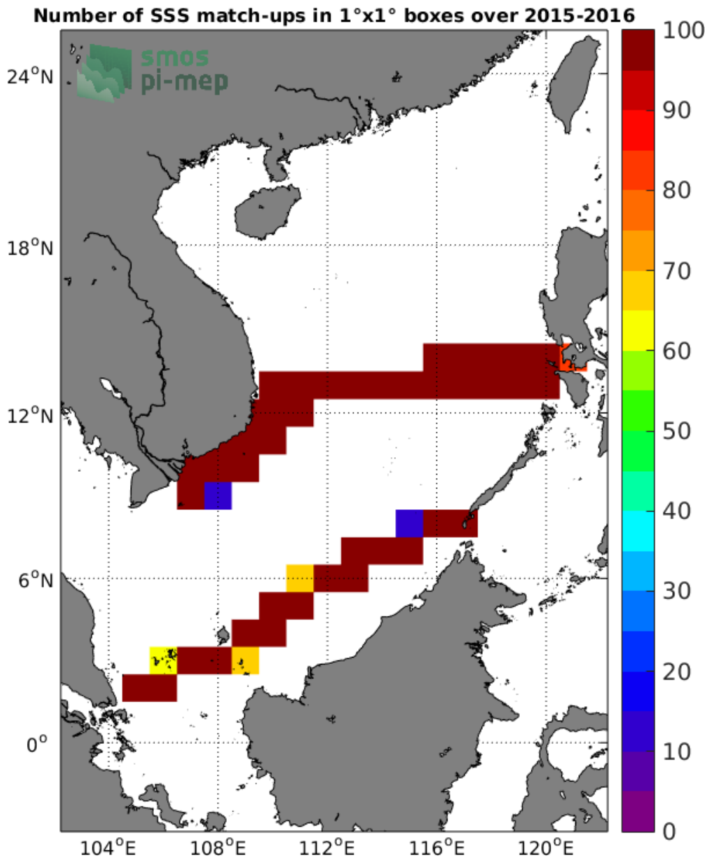
Figure 4: Number of SSS match-ups between TSG-SAMOS SSS and the SMAP-L3-JPL-V4-MONTHLY-60KM SSS product for the South China Sea Pi-MEP region over 1°x1° boxes and for the full satellite product period.
