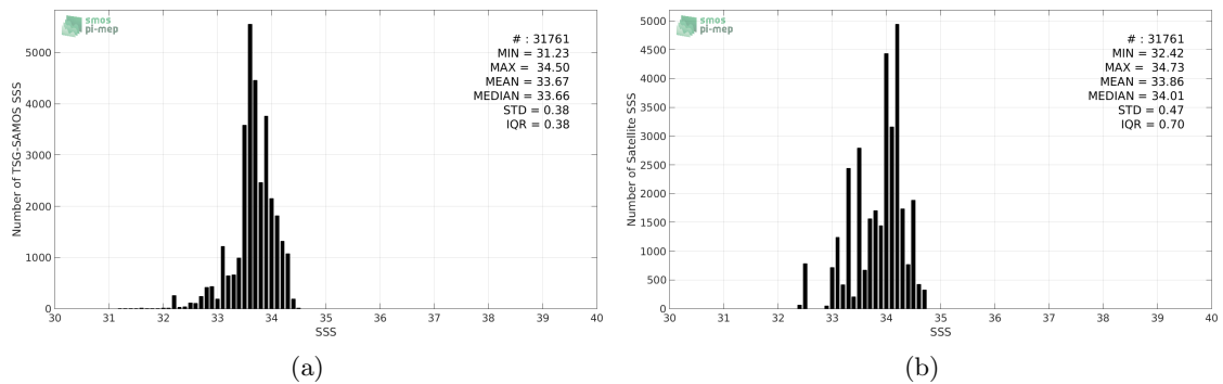
Figure 2: Histograms of SSS from TSG-SAMOS (a) and SMAP-L3-JPL-V4-MONTHLY-60KM (b) considering all match-up pairs per bins of 0.1 over the South China Sea Pi-MEP region and for the full satellite product period.
