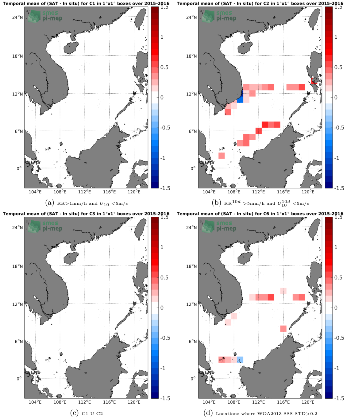
Figure 12: Temporal mean gridded over spatial boxes of size 1°x1° of \Delta\text{SSS} (SMAP-L3-JPL-V4-MONTHLY-60KM - TSG-SAMOS) for 4 different subdatasets corresponding to: RR > 1\text{mm/h} and U_{10} < 5\text{m/s} (a), RR^{10d} > 5\text{mm/h} and U_{10}^{10d} < 5\text{m/s} (b), C1 U C2 (c), Locations where WOA2013 SSS STD > 0.2 (d).
