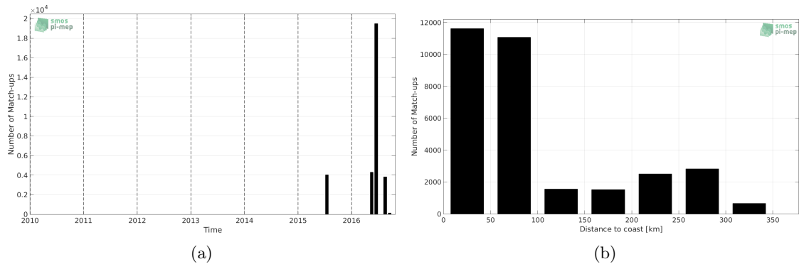
Figure 1: Number of match-ups between TSG-SAMOS and SMAP-L3-JPL-V4-MONTHLY-60KM SSS as a function of time (a) and as function of the distance to coast (b) over the South China Sea Pi-MEP region and for the full satellite product period.
