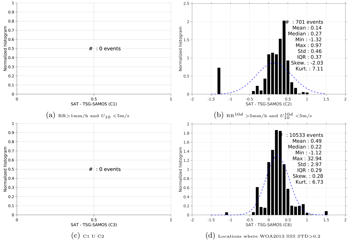
Figure 13: Normalized histogram of \Delta\text{SSS} (SMAP-L3-JPL-V4-MONTHLY-60KM - TSG-SAMOS) for 6 different subdatasets corresponding to: RR > 1\text{mm/h} and U_{10} < 5\text{m/s} (a), RR^{10d} > 5\text{mm/h} and U_{10}^{10d} < 5\text{m/s} (b), C1 \cup C2 (c), Locations where WOA2013 SSS STD > 0.2 (d).
