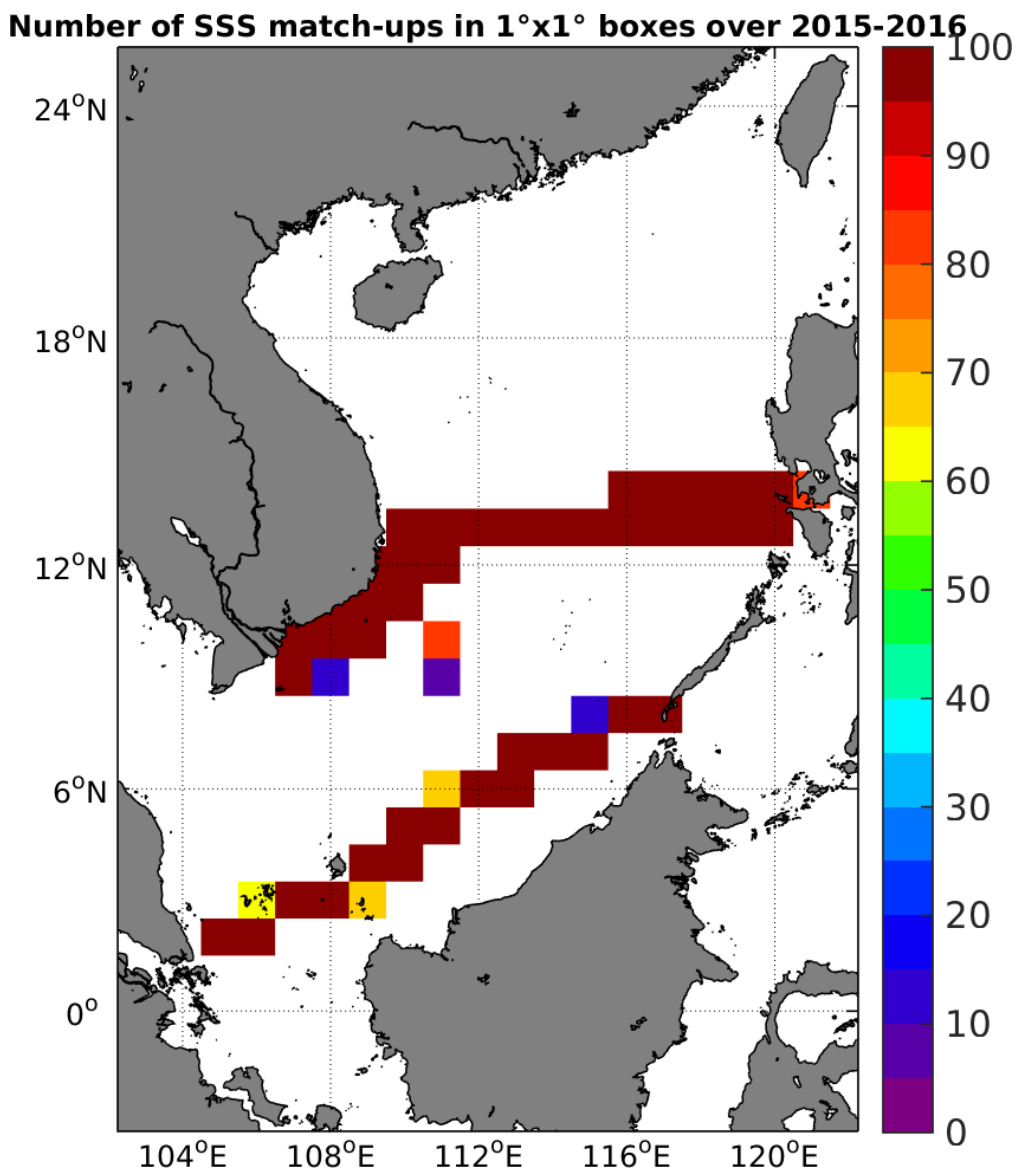
Figure 4: Number of SSS match-ups between TSG-SAMOS SSS and the SMAP-L3-JPL-V4-MONTHLY-60KM SSS product for the South China Sea Pi-MEP region over 1°x1° boxes and for the full satellite product period.
