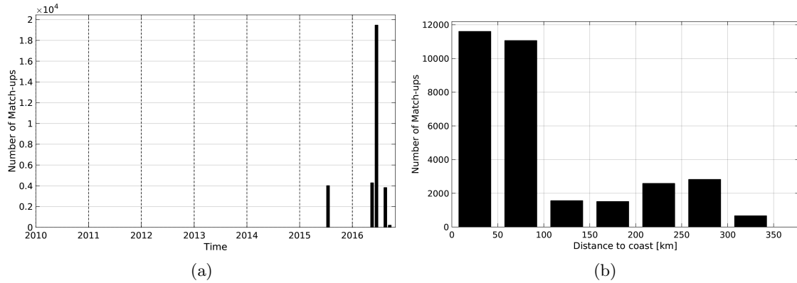
Figure 1: Number of match-ups between TSG-SAMOS and SMAP-L3-JPL-V4-MONTHLY-60KM SSS as a function of time (a) and as function of the distance to coast (b) over the South China Sea Pi-MEP region and for the full satellite product period.
