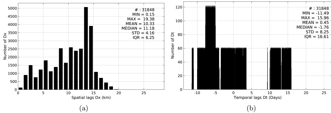
Figure 5: Histograms of the spatial (a) and temporal (b) lags between the time of the TSG-SAMOS measurements and the date of the corresponding SMAP-L3-JPL-V4-MONTHLY-60KM SSS product.
