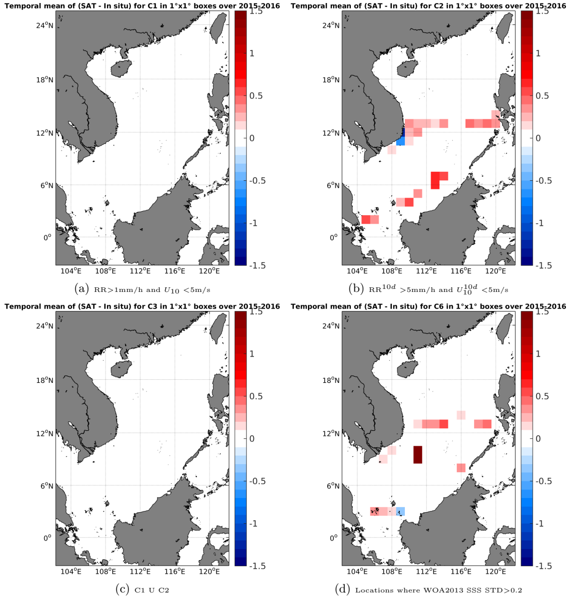
Figure 12: Temporal mean gridded over spatial boxes of size 1°x1° of ΔSSS (SMAP-L3-JPL-V4-MONTHLY-60KM - TSG-SAMOS) for 4 different subdatasets corresponding to: RR > 1\text{mm/h} and U_{10} < 5\text{m/s} (a), RR^{10d} > 5\text{mm/h} and U_{10}^{10d} < 5\text{m/s} (b), C1 U C2 (c), Locations where WOA2013 SSS STD > 0.2 (d).
