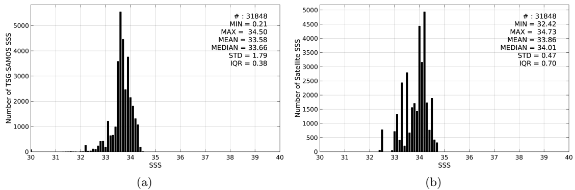
Figure 2: Histograms of SSS from TSG-SAMOS (a) and SMAP-L3-JPL-V4-MONTHLY-60KM (b) considering all match-up pairs per bins of 0.1 over the South China Sea Pi-MEP region and for the full satellite product period.
