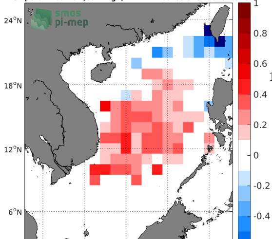
Temporal mean of (Sat-Argo) in 1°x1° boxes over 2015-2018
