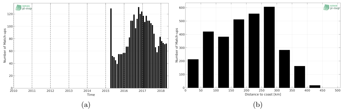
Figure 1: Number of match-ups between Argo and SMAP-L3-JPL-V4-MONTHLY-60KM SSS as a function of time (a) and as function of the distance to coast (b) over the South China Sea Pi-MEP region and for the full satellite product period.
