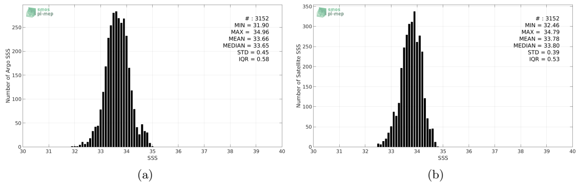
Figure 2: Histograms of SSS from Argo (a) and SMAP-L3-JPL-V4-MONTHLY-60KM (b) considering all match-up pairs per bins of 0.1 over the South China Sea Pi-MEP region and for the full satellite product period.
