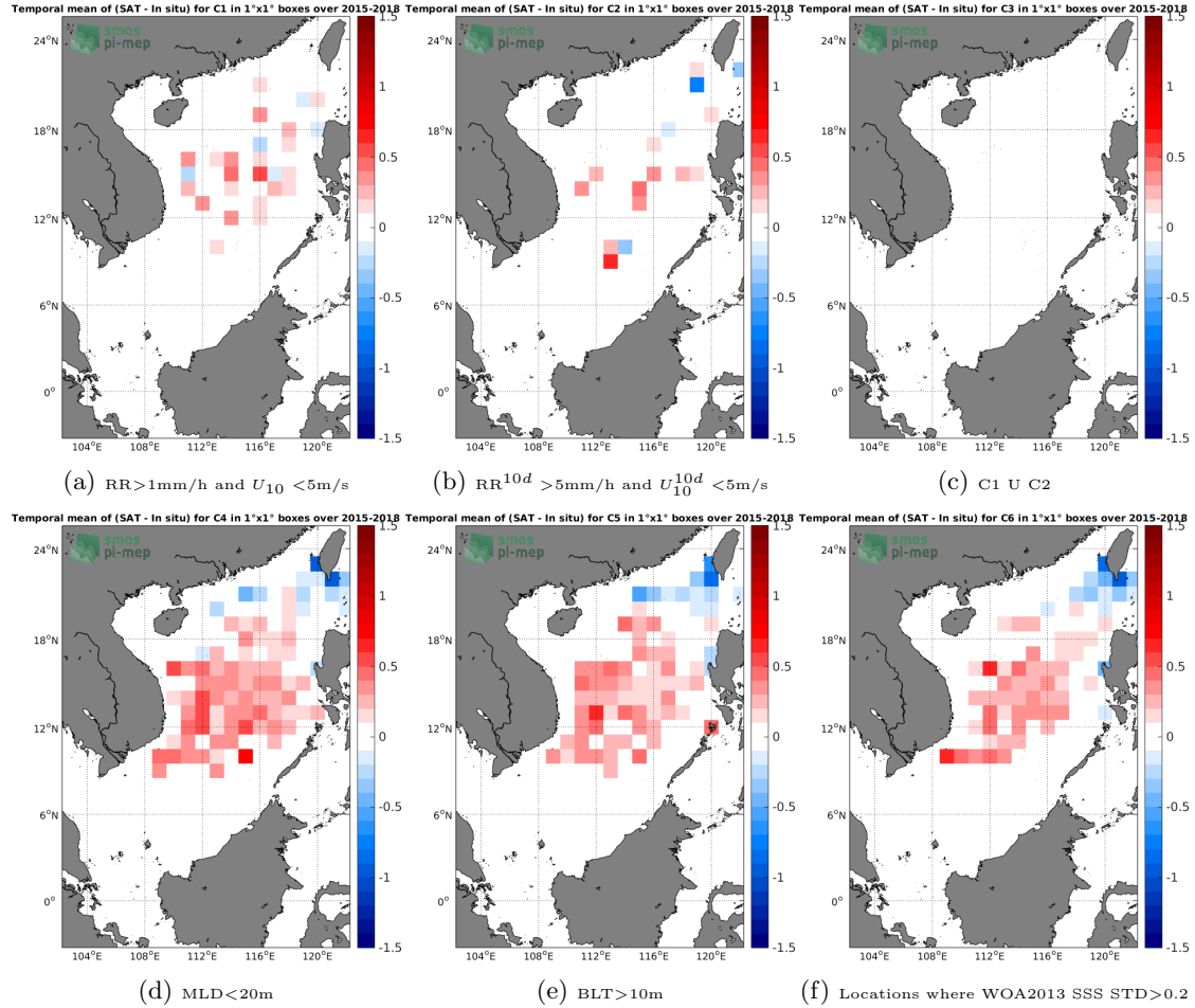
Figure 12: Temporal mean gridded over spatial boxes of size 1^\circ \times 1^\circ of \Delta SSS (SMAP-L3-JPL-V4-MONTHLY-60KM - Argo) for 6 different subdatasets corresponding to: RR > 1\text{mm/h} and U_{10} < 5\text{m/s} (a), RR^{10d} > 5\text{mm/h} and U_{10}^{10d} < 5\text{m/s} (b), C1 U C2 (c), MLD < 20\text{m} (d), BLT > 10\text{m} (e), Locations where WOA2013 SSS STD > 0.2 (f).
