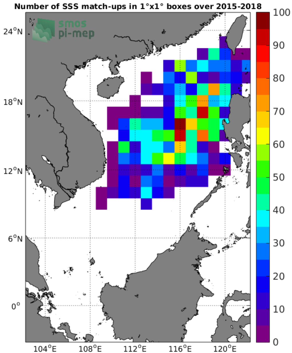
Figure 4: Number of SSS match-ups between Argo SSS and the SMAP-L3-JPL-V4-MONTHLY-60KM SSS product for the South China Sea Pi-MEP region over 1°x1° boxes and for the full satellite product period.
