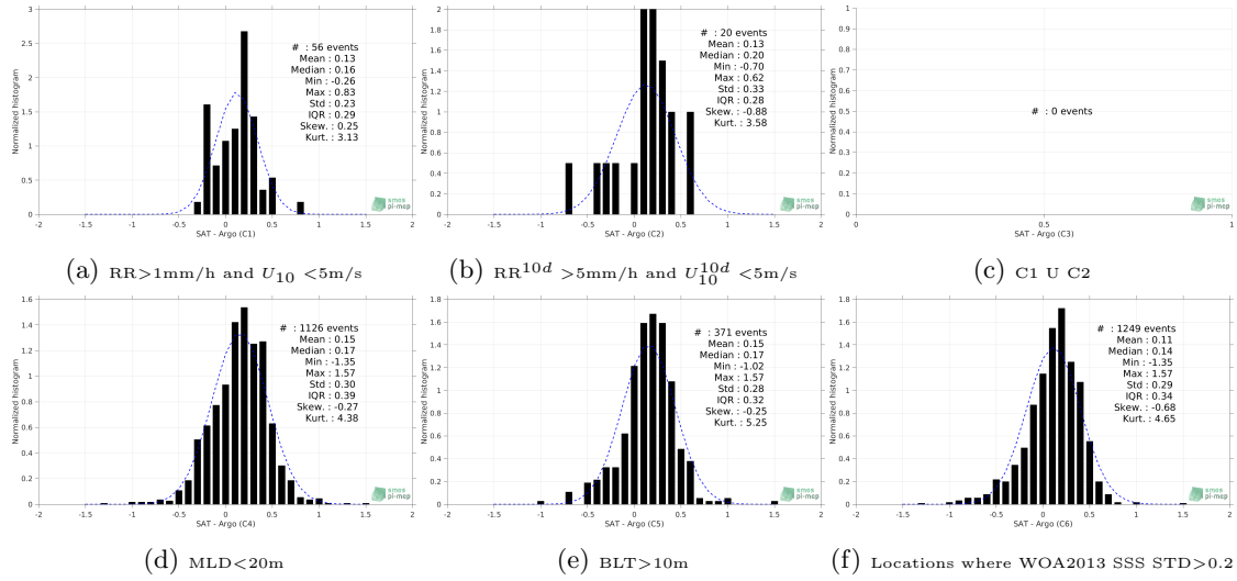
Figure 13: Normalized histogram of \Delta SSS (SMAP-L3-JPL-V4-MONTHLY-60KM - Argo) for 6 different subdatasets corresponding to: RR > 1mm/h and U_{10} < 5 m/s (a), RR 10d > 5mm/h and U_{10}^{10d} < 5 m/s (b), C1 U C2 (c), MLD < 20m (d), BLT > 10m (e), Locations where WOA2013 SSS STD > 0.2 (f).
