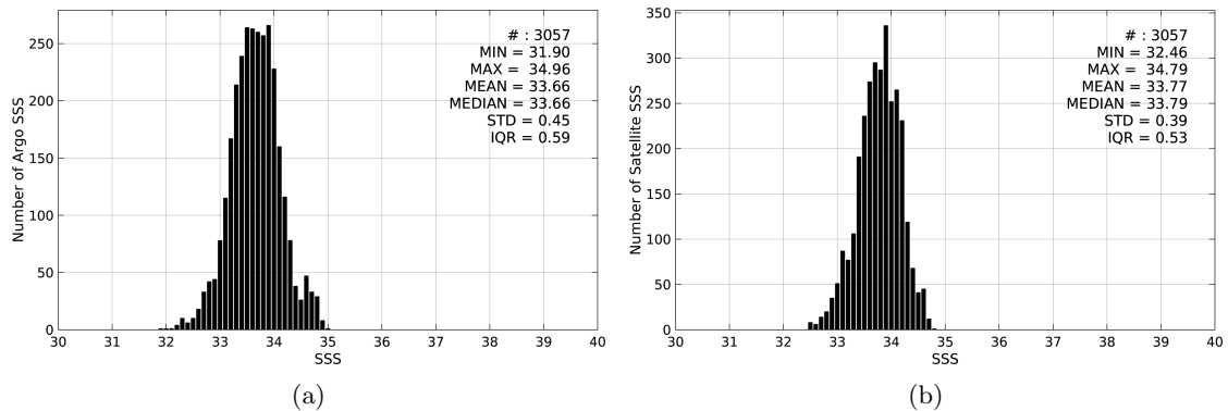
Figure 2: Histograms of SSS from Argo (a) and SMAP-L3-JPL-V4-MONTHLY-60KM (b) considering all match-up pairs per bins of 0.1 over the South China Sea Pi-MEP region and for the full satellite product period.
