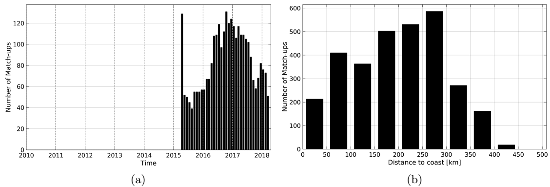
Figure 1: Number of match-ups between Argo and SMAP-L3-JPL-V4-MONTHLY-60KM SSS as a function of time (a) and as function of the distance to coast (b) over the South China Sea Pi-MEP region and for the full satellite product period.
