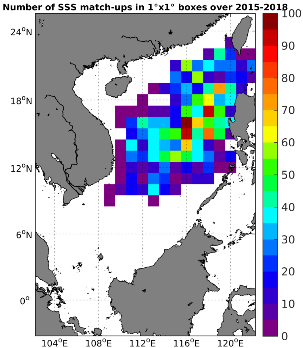
Figure 4: Number of SSS match-ups between Argo SSS and the SMAP-L3-JPL-V4-MONTHLY-60KM SSS product for the South China Sea Pi-MEP region over 1°x1° boxes and for the full satellite product period.
