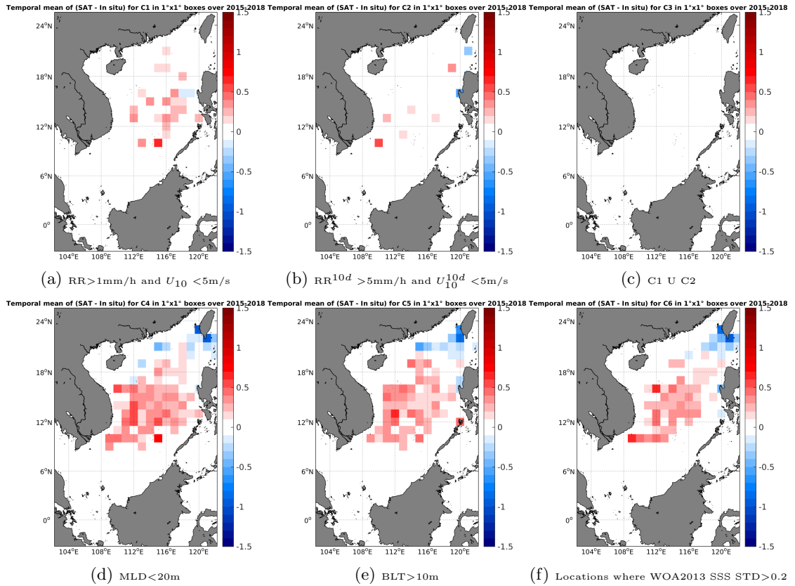
Figure 12: Temporal mean gridded over spatial boxes of size 1^\circ \times 1^\circ of \Delta SSS (SMAP-L3-JPL-V4-MONTHLY-60KM - Argo) for 6 different subdatasets corresponding to: RR > 1\text{mm/h} and U_{10} < 5\text{m/s} (a), RR^{10d} > 5\text{mm/h} and U_{10}^{10d} < 5\text{m/s} (b), C1 U C2 (c), MLD < 20\text{m} (d), BLT > 10\text{m} (e), Locations where WOA2013 SSS STD > 0.2 (f).
