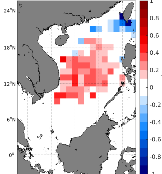
Temporal mean of (Sat-Argo) in 1°x1° boxes over 2015-2018
