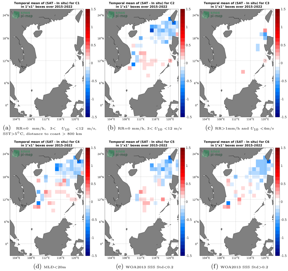
Figure 12: Temporal mean gridded over spatial boxes of size 1^\circ \times 1^\circ of \Delta SSS (SMAP SSS L2-AVERAGED v5 (RSS) - Argo) for 6 different subdatasets corresponding to:RR=0 mm/h, 3 < U_{10} < 12 m/s, SST > 5°C, distance to coast > 800 km (a), RR=0 mm/h, 3 < U_{10} < 12 m/s (b), RR > 1mm/h and U_{10} < 4 m/s (c),MLD < 20m (d),WOA2013 SSS Std < 0.2 (e),WOA2013 SSS Std > 0.2 (f).
