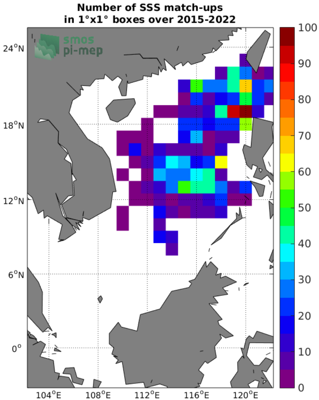
Figure 4: Number of SSS match-ups between Argo SSS and the SMAP SSS L2-AVERAGED v5 (RSS) SSS product for the South China Sea Pi-MEP region over 1°x1° boxes and for the full satellite product period.
