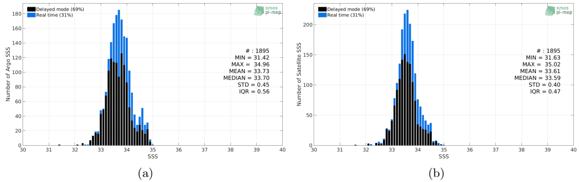
Figure 2: Histograms of SSS from Argo (a) and SMAP SSS L2-AVERAGED v5 (RSS) (b) considering all match-up pairs per bins of 0.1 over the South China Sea Pi-MEP region and for the full satellite product period.
