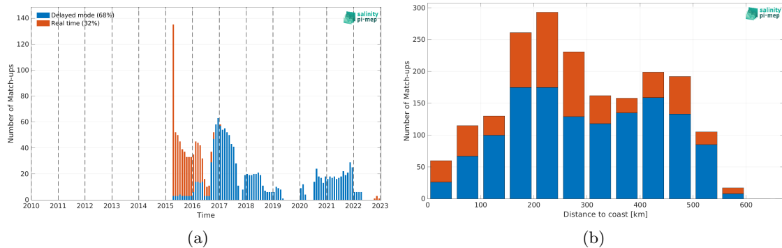
Figure 1: Number of match-ups between Argo and SMAP SSS L2-AVERAGED v5.0 (JPL) SSS as a function of time (a) and as function of the distance to coast (b) over the South China Sea Pi-MEP region and for the full satellite product period.
