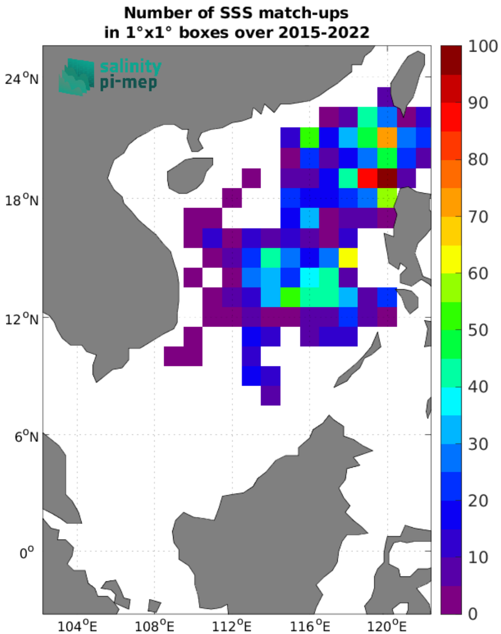
Figure 3: Number of SSS match-ups between Argo SSS and the SMAP SSS L2-AVERAGED v5.0 (JPL) SSS product for the South China Sea Pi-MEP region over 1^{\circ} \times 1^{\circ} boxes and for the full satellite product period.
