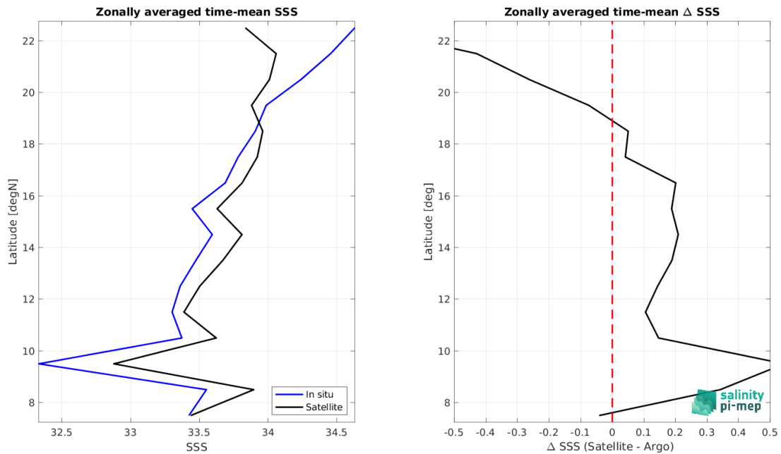
Figure 7: Left panel: Zonal mean SSS from SMAP SSS L2-AVERAGED v5.0 (JPL) satellite product (black) and from Argo (blue). Right panel: Zonal mean of \Delta SSS (Satellite - Argo) for all the collected Pi-MEP match-up pairs estimated over the full satellite product period.
