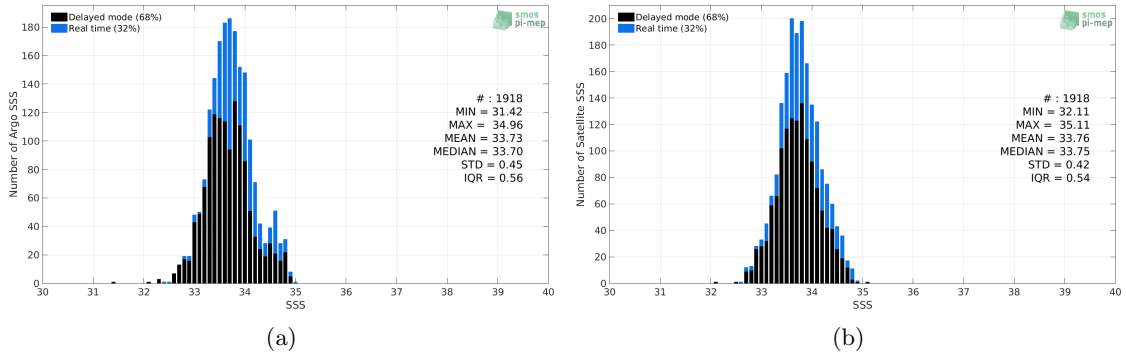
Figure 2: Histograms of SSS from Argo (a) and SMAP SSS L2-AVERAGED v5.0 (JPL) (b) considering all match-up pairs per bins of 0.1 over the South China Sea Pi-MEP region and for the full satellite product period.
