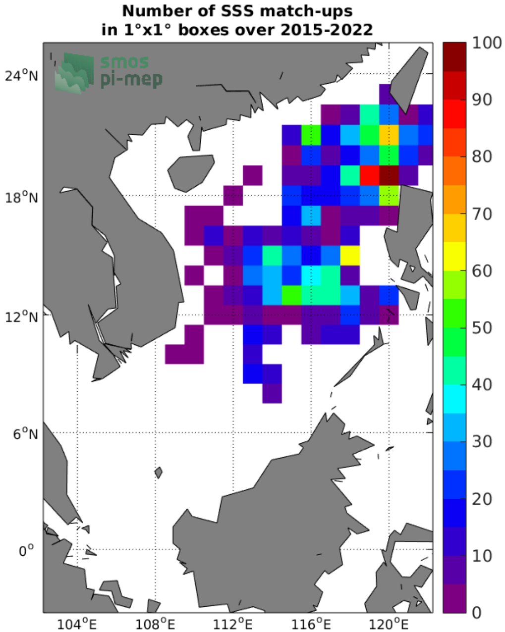
Figure 4: Number of SSS match-ups between Argo SSS and the SMAP SSS L2-AVERAGED v5.0 (JPL) SSS product for the South China Sea Pi-MEP region over 1^\circ \times 1^\circ boxes and for the full satellite product period.
