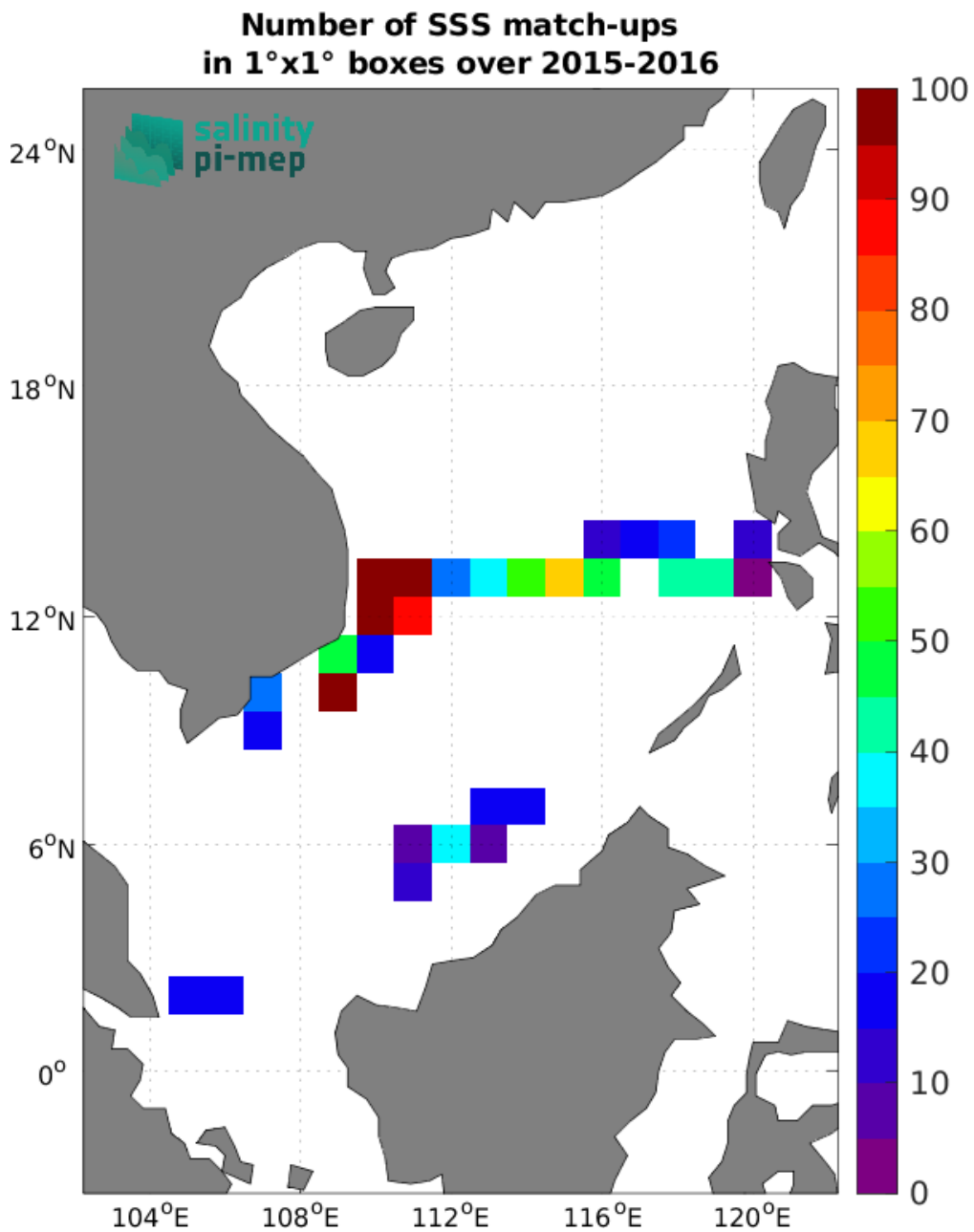
Figure 5: Number of SSS match-ups between TSG (SAMOS) SSS and the SMAP SSS L2 v6 - 40 km (RSS) SSS product for the South China Sea Pi-MEP region over 1°x1° boxes and for the full satellite product period.
