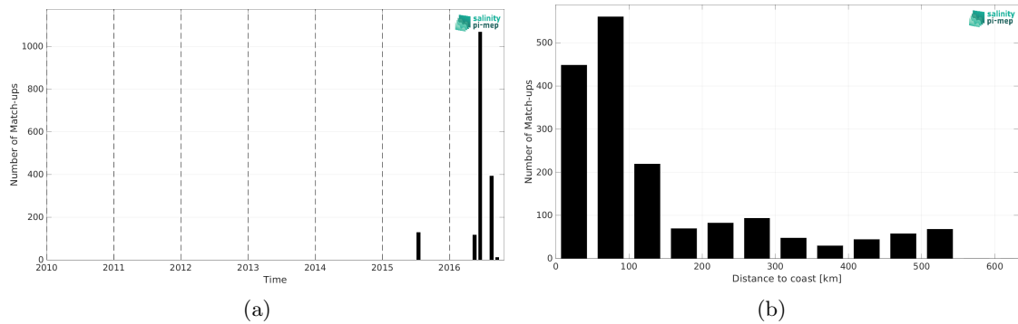
Figure 2: Number of match-ups between TSG (SAMOS) and SMAP SSS L2 v6 - 40 km (RSS) SSS as a function of time (a) and as function of the distance to coast (b) over the South China Sea Pi-MEP region and for the full satellite product period.
