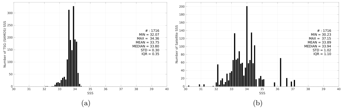
Figure 3: Histograms of SSS from TSG (SAMOS) (a) and SMAP SSS L2 v6 - 40 km (RSS) (b) considering all match-up pairs per bins of 0.1 over the South China Sea Pi-MEP region and for the full satellite product period.
