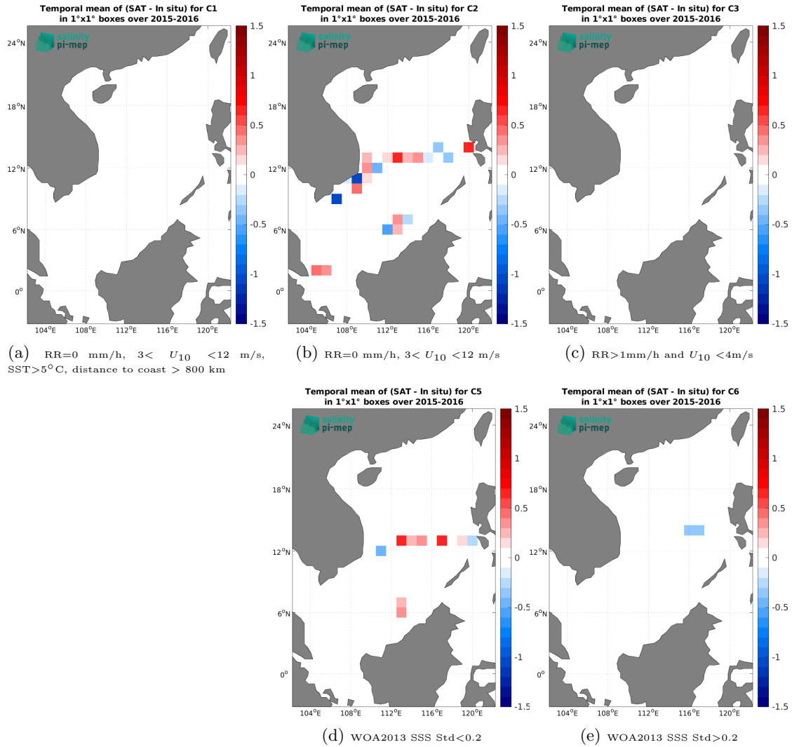
Figure 14: Temporal mean gridded over spatial boxes of size 1^\circ \times 1^\circ of \Delta\text{SSS} (SMAP SSS L2 v6 - 40 km (RSS) - TSG (SAMOS)) for 5 different subdatasets corresponding to: RR=0 mm/h, 3 < U_{10} < 12 m/s, SST > 5^\circ\text{C} , distance to coast > 800 km (a), RR=0 mm/h, 3 < U_{10} < 12 m/s (b), RR > 1 mm/h and U_{10} < 4 m/s (c), WOA2013 SSS Std < 0.2 (d), WOA2013 SSS Std > 0.2 (e).
