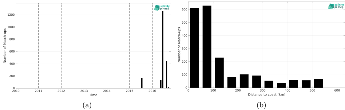
Figure 1: Number of match-ups between TSG (SAMOS) and SMAP SSS L2 v5 (RSS) SSS as a function of time (a) and as function of the distance to coast (b) over the South China Sea Pi-MEP region and for the full satellite product period.
