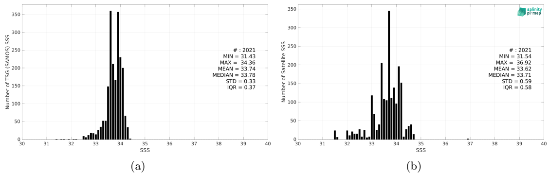
Figure 2: Histograms of SSS from TSG (SAMOS) (a) and SMAP SSS L2 v5 (RSS) (b) considering all match-up pairs per bins of 0.1 over the South China Sea Pi-MEP region and for the full satellite product period.
