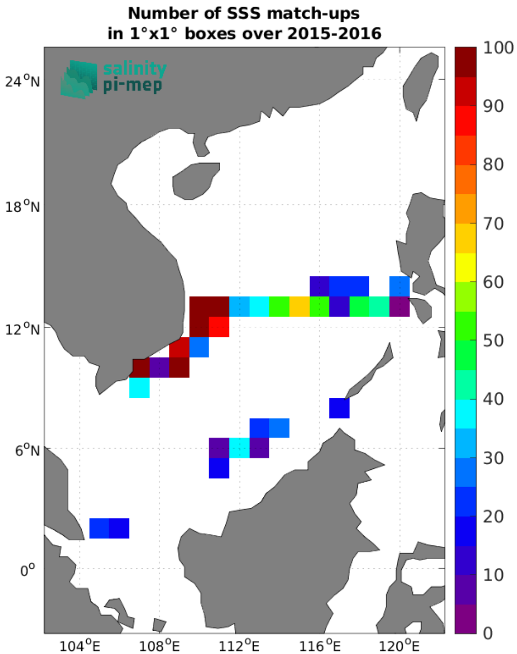
Figure 4: Number of SSS match-ups between TSG (SAMOS) SSS and the SMAP SSS L2 v5 (RSS) SSS product for the South China Sea Pi-MEP region over 1^{\circ} \times 1^{\circ} boxes and for the full satellite product period.
