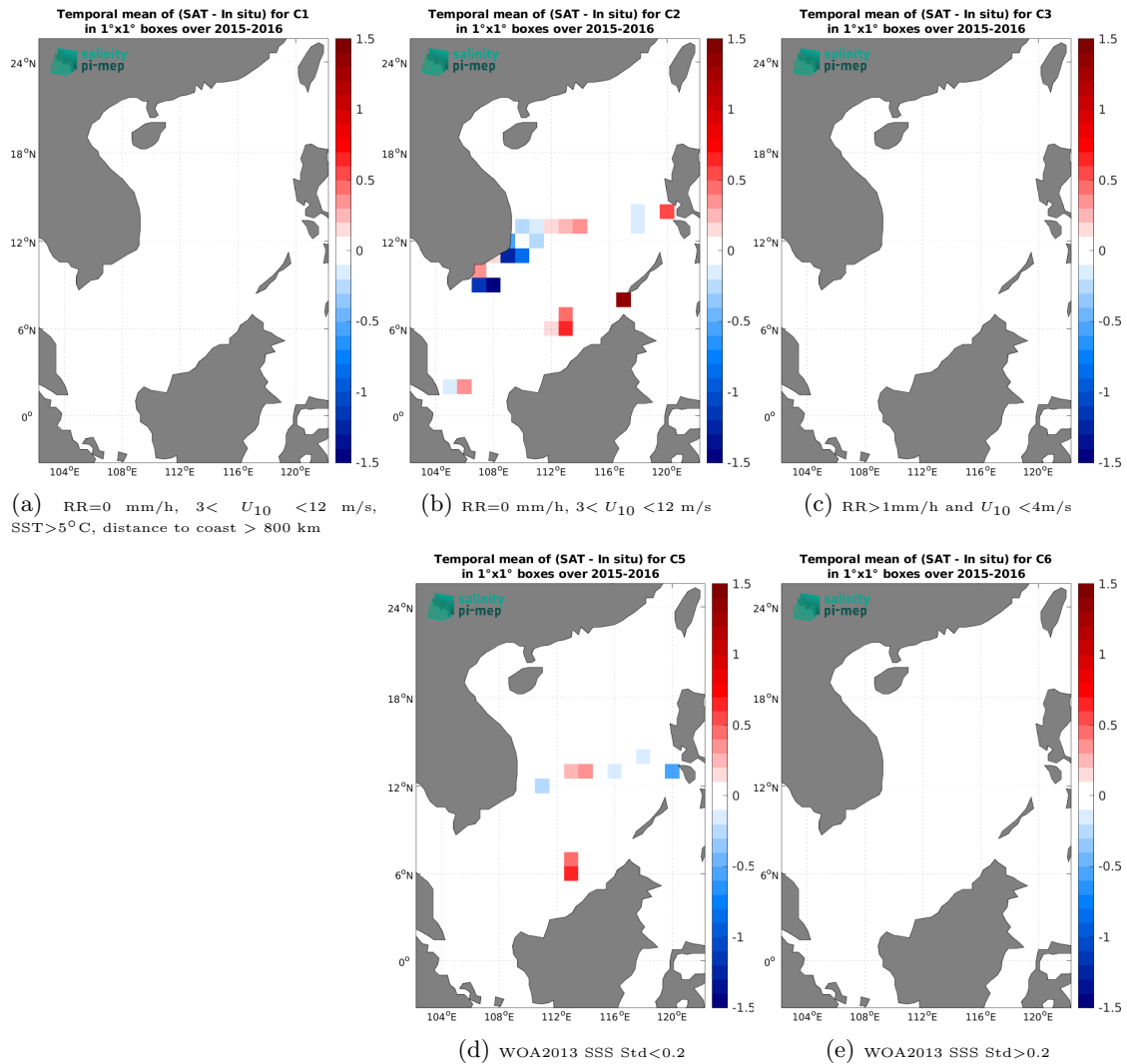
Figure 12: Temporal mean gridded over spatial boxes of size 1^\circ \times 1^\circ of \Delta\text{SSS} (SMAP SSS L2 v5 (RSS) - TSG (SAMOS)) for 5 different subdatasets corresponding to:RR=0 mm/h, 3 < U_{10} < 12 m/s, SST >5^\circ\text{C} , distance to coast > 800 km (a), RR=0 mm/h, 3 < U_{10} < 12 m/s (b), RR >1 mm/h and U_{10} < 4 m/s (c), WOA2013 SSS Std <0.2 (d), WOA2013 SSS Std >0.2 (e).
