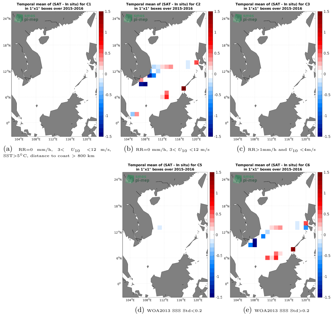
Figure 12: Temporal mean gridded over spatial boxes of size 1^\circ \times 1^\circ of \Delta SSS (SMAP SSS L2 v5 (RSS) - TSG (SAMOS)) for 5 different subdatasets corresponding to:RR=0 mm/h, 3 < U_{10} < 12 m/s, SST>5°C, distance to coast > 800 km (a), RR=0 mm/h, 3 < U_{10} < 12 m/s (b), RR>1mm/h and U_{10} < 4 m/s (c), WOA2013 SSS Std<0.2 (d), WOA2013 SSS Std>0.2 (e).
