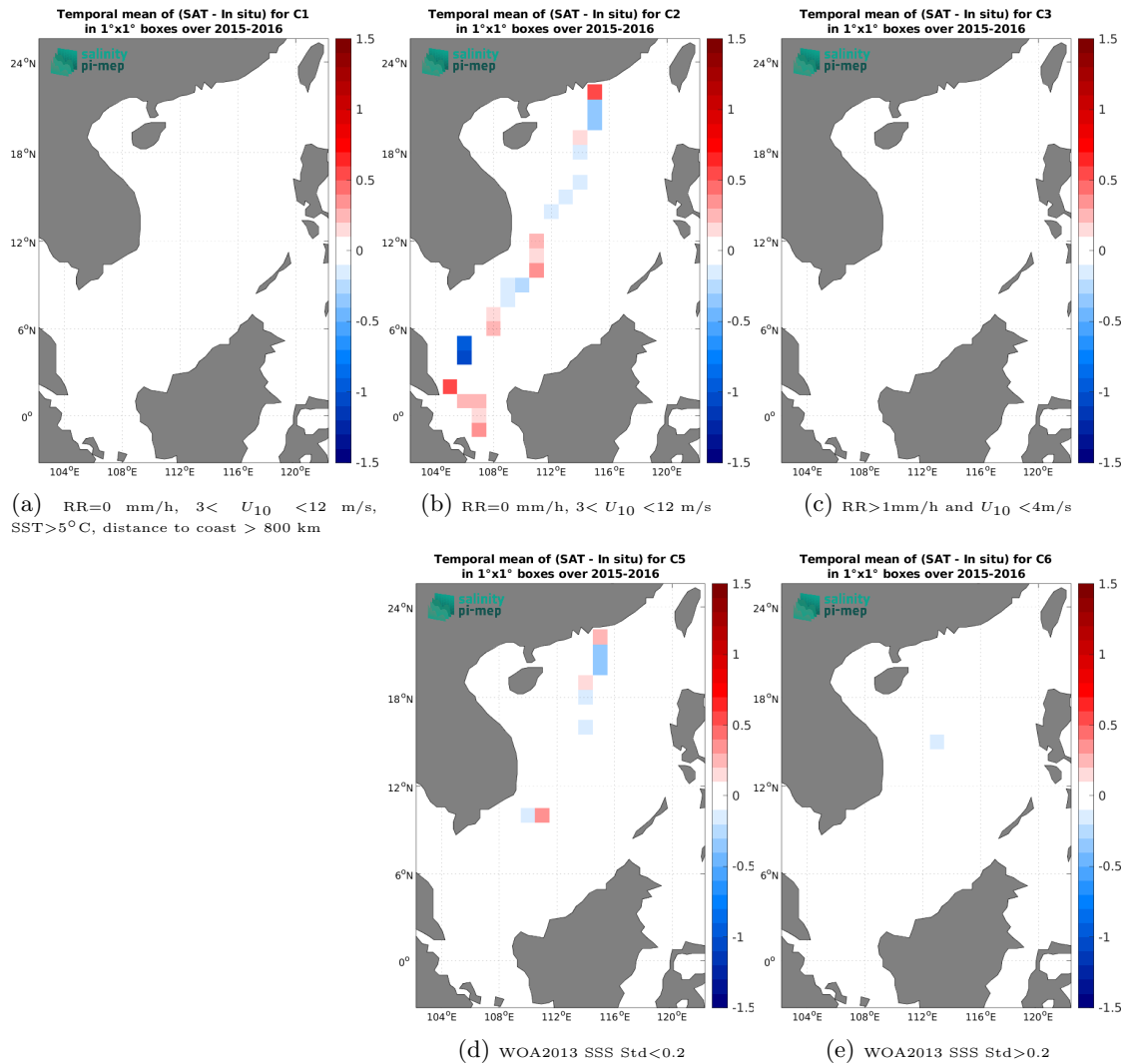
Figure 12: Temporal mean gridded over spatial boxes of size 1^\circ \times 1^\circ of \Delta SSS (SMAP SSS L2 v5 (RSS) - TSG (LEGOS-DM)) for 5 different subdatasets corresponding to:RR=0 mm/h, 3 < U_{10} < 12 m/s, SST >5^\circ\text{C} , distance to coast > 800 km (a), RR=0 mm/h, 3 < U_{10} < 12 m/s (b), RR >1 mm/h and U_{10} < 4 m/s (c), WOA2013 SSS Std <0.2 (d), WOA2013 SSS Std >0.2 (e).
