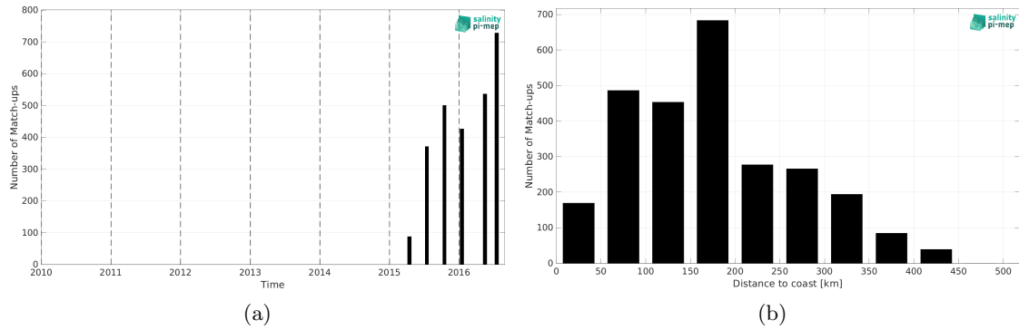
Figure 1: Number of match-ups between TSG (LEGOS-DM) and SMAP SSS L2 v5 (RSS) SSS as a function of time (a) and as function of the distance to coast (b) over the South China Sea Pi-MEP region and for the full satellite product period.
