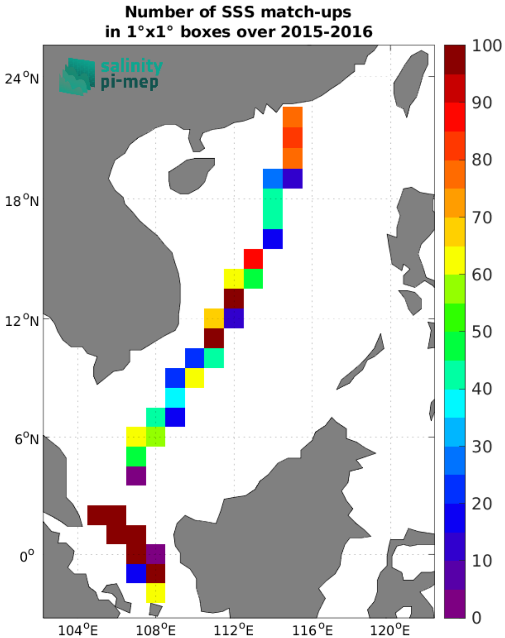
Figure 4: Number of SSS match-ups between TSG (LEGOS-DM) SSS and the SMAP SSS L2 v5 (RSS) SSS product for the South China Sea Pi-MEP region over 1°×1° boxes and for the full satellite product period.
