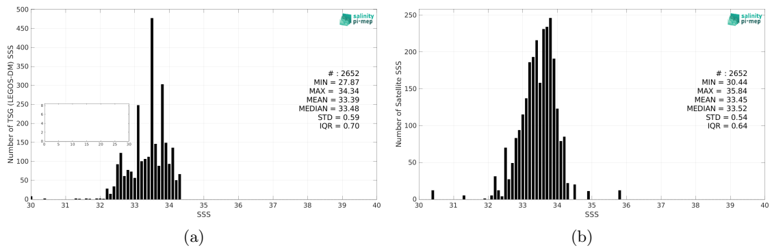
Figure 2: Histograms of SSS from TSG (LEGOS-DM) (a) and SMAP SSS L2 v5 (RSS) (b) considering all match-up pairs per bins of 0.1 over the South China Sea Pi-MEP region and for the full satellite product period.
