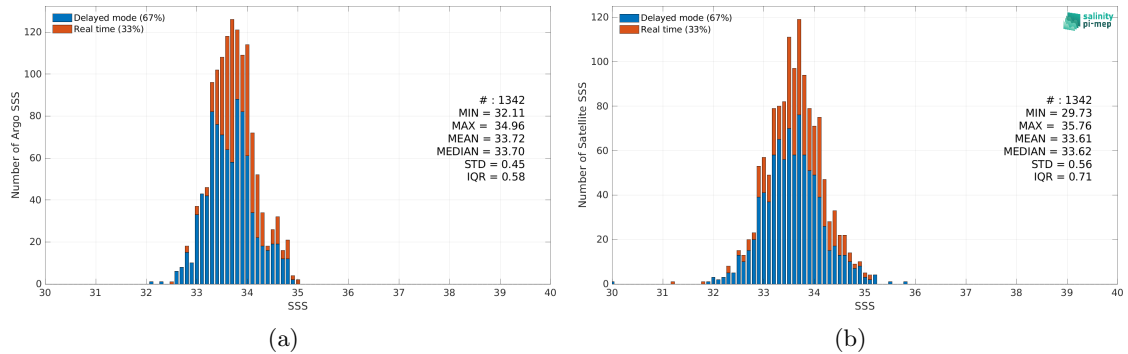
Figure 2: Histograms of SSS from Argo (a) and SMAP SSS L2 v5 (RSS) (b) considering all match-up pairs per bins of 0.1 over the South China Sea Pi-MEP region and for the full satellite product period.
