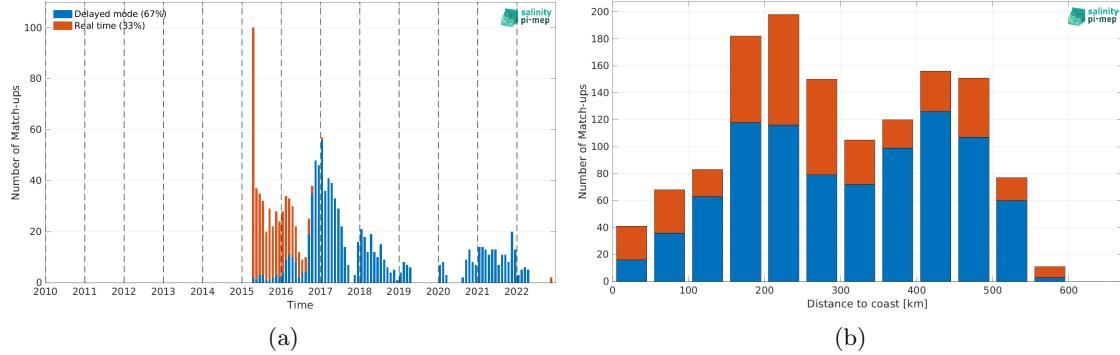
Figure 1: Number of match-ups between Argo and SMAP SSS L2 v5 (RSS) SSS as a function of time (a) and as function of the distance to coast (b) over the South China Sea Pi-MEP region and for the full satellite product period.
