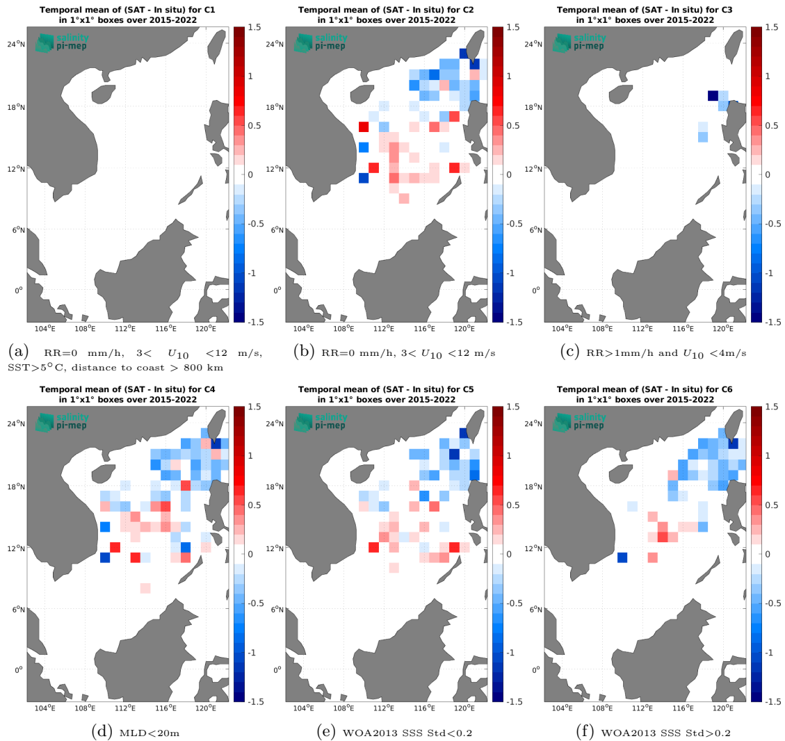
Figure 12: Temporal mean gridded over spatial boxes of size 1^\circ \times 1^\circ of \Delta SSS (SMAP SSS L2 v5 (RSS) - Argo) for 6 different subdatasets corresponding to:RR=0 mm/h, 3 < U_{10} < 12 m/s, SST > 5^\circ\text{C} , distance to coast > 800 km (a), RR=0 mm/h, 3 < U_{10} < 12 m/s (b), RR > 1 mm/h and U_{10} < 4 m/s (c),MLD < 20 m (d),WOA2013 SSS Std < 0.2 (e),WOA2013 SSS Std > 0.2 (f).
