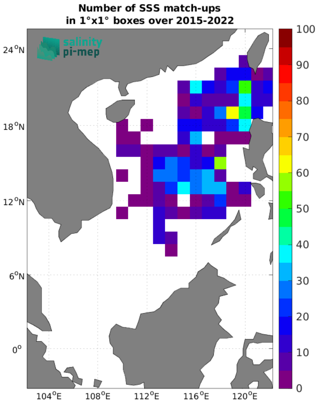
Figure 4: Number of SSS match-ups between Argo SSS and the SMAP SSS L2 v5 (RSS) SSS product for the South China Sea Pi-MEP region over 1^\circ \times 1^\circ boxes and for the full satellite product period.
