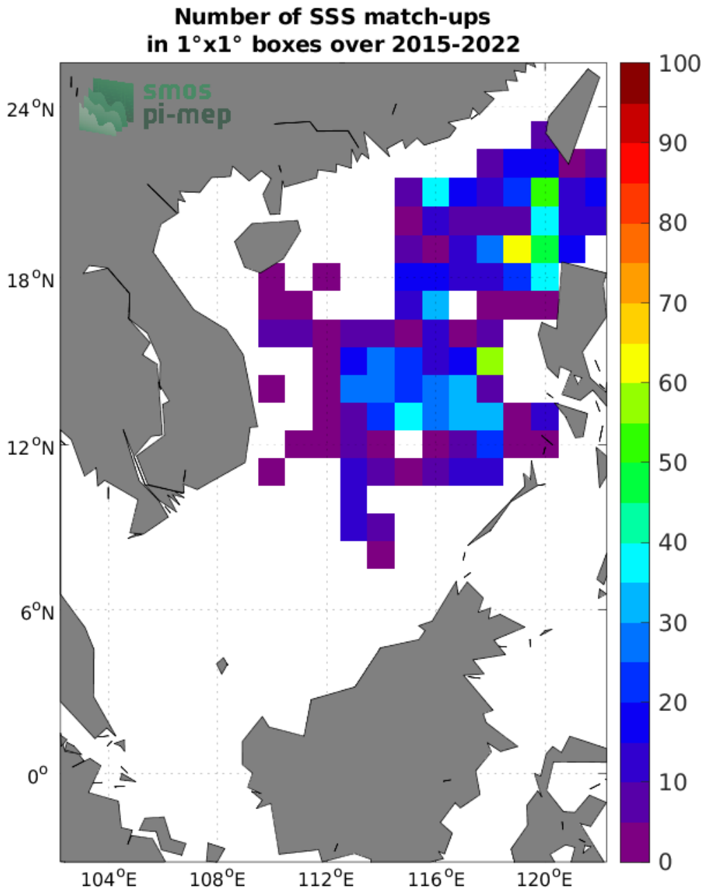
Figure 4: Number of SSS match-ups between Argo SSS and the SMAP SSS L2 v5 (RSS) SSS product for the South China Sea Pi-MEP region over 1°x1° boxes and for the full satellite product period.
