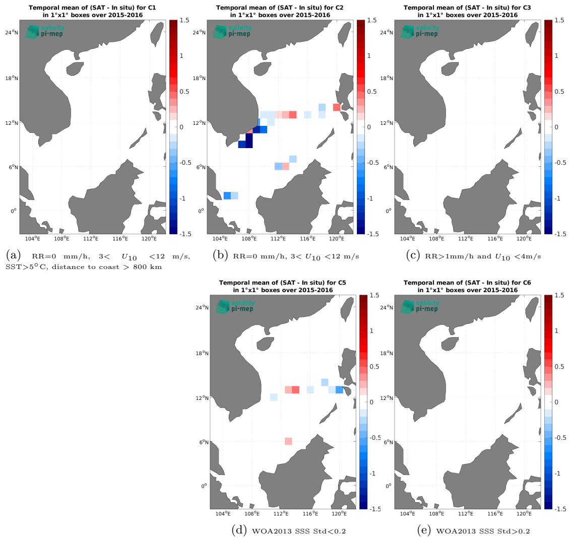
Figure 14: Temporal mean gridded over spatial boxes of size 1^\circ \times 1^\circ of \Delta\text{SSS} (SMAP SSS L2 v5.3 (RSS) - TSG (SAMOS)) for 5 different subdatasets corresponding to: RR=0 mm/h, 3 < U_{10} < 12 m/s, SST > 5^\circ\text{C} , distance to coast > 800 km (a), RR=0 mm/h, 3 < U_{10} < 12 m/s (b), RR > 1 mm/h and U_{10} < 4 m/s (c), WOA2013 SSS Std < 0.2 (d), WOA2013 SSS Std > 0.2 (e).
