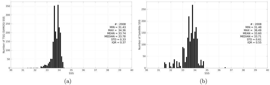
Figure 3: Histograms of SSS from TSG (SAMOS) (a) and SMAP SSS L2 v5.3 (RSS) (b) considering all match-up pairs per bins of 0.1 over the South China Sea Pi-MEP region and for the full satellite product period.
