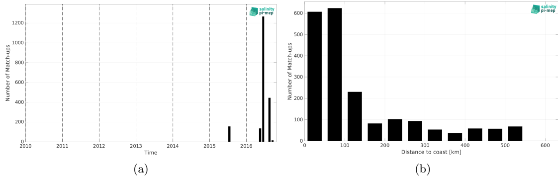
Figure 2: Number of match-ups between TSG (SAMOS) and SMAP SSS L2 v5.3 (RSS) SSS as a function of time (a) and as function of the distance to coast (b) over the South China Sea Pi-MEP region and for the full satellite product period.
