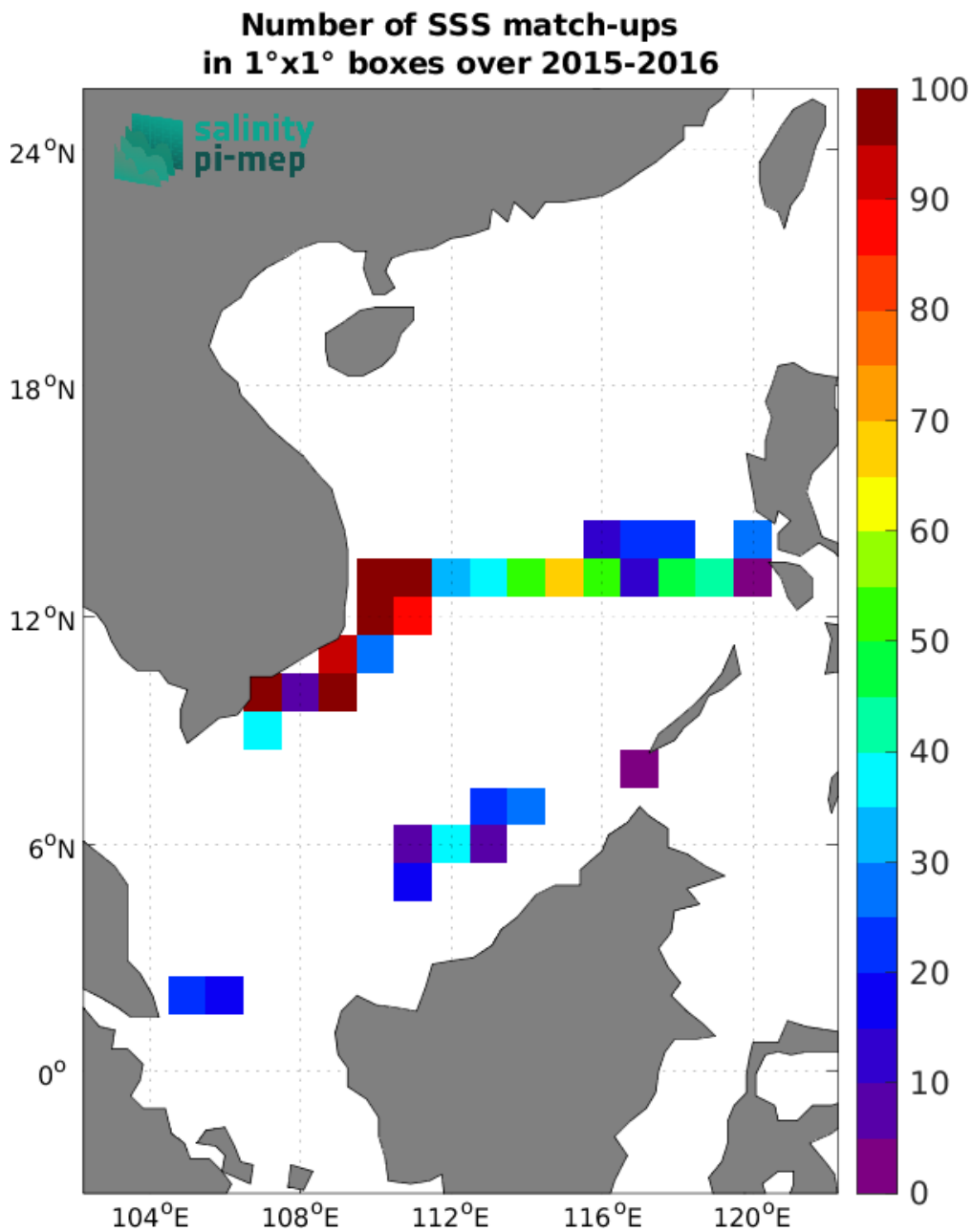
Figure 5: Number of SSS match-ups between TSG (SAMOS) SSS and the SMAP SSS L2 v5.3 (RSS) SSS product for the South China Sea Pi-MEP region over 1^\circ \times 1^\circ boxes and for the full satellite product period.
