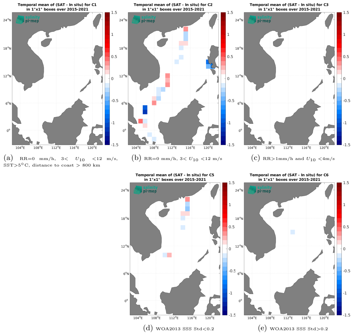
Figure 14: Temporal mean gridded over spatial boxes of size 1^\circ \times 1^\circ of \Delta\text{SSS} (SMAP SSS L2 v5.3 (RSS) - TSG (LEGOS-DM)) for 5 different subdatasets corresponding to: RR=0 mm/h, 3 < U_{10} < 12 m/s, SST > 5^\circ\text{C} , distance to coast > 800 km (a), RR=0 mm/h, 3 < U_{10} < 12 m/s (b), RR > 1 mm/h and U_{10} < 4 m/s (c), WOA2013 SSS Std < 0.2 (d), WOA2013 SSS Std > 0.2 (e).
