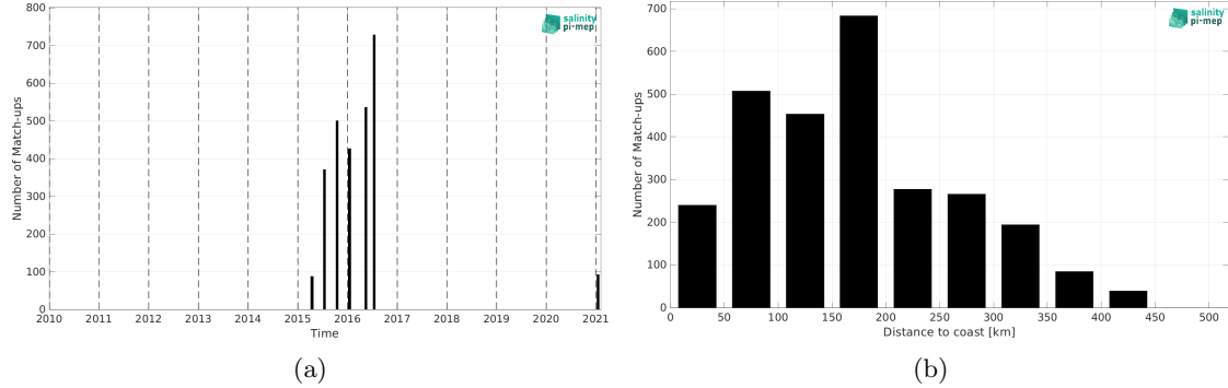
Figure 2: Number of match-ups between TSG (LEGOS-DM) and SMAP SSS L2 v5.3 (RSS) SSS as a function of time (a) and as function of the distance to coast (b) over the South China Sea Pi-MEP region and for the full satellite product period.
