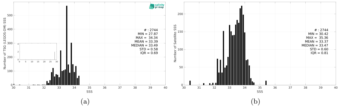
Figure 3: Histograms of SSS from TSG (LEGOS-DM) (a) and SMAP SSS L2 v5.3 (RSS) (b) considering all match-up pairs per bins of 0.1 over the South China Sea Pi-MEP region and for the full satellite product period.
