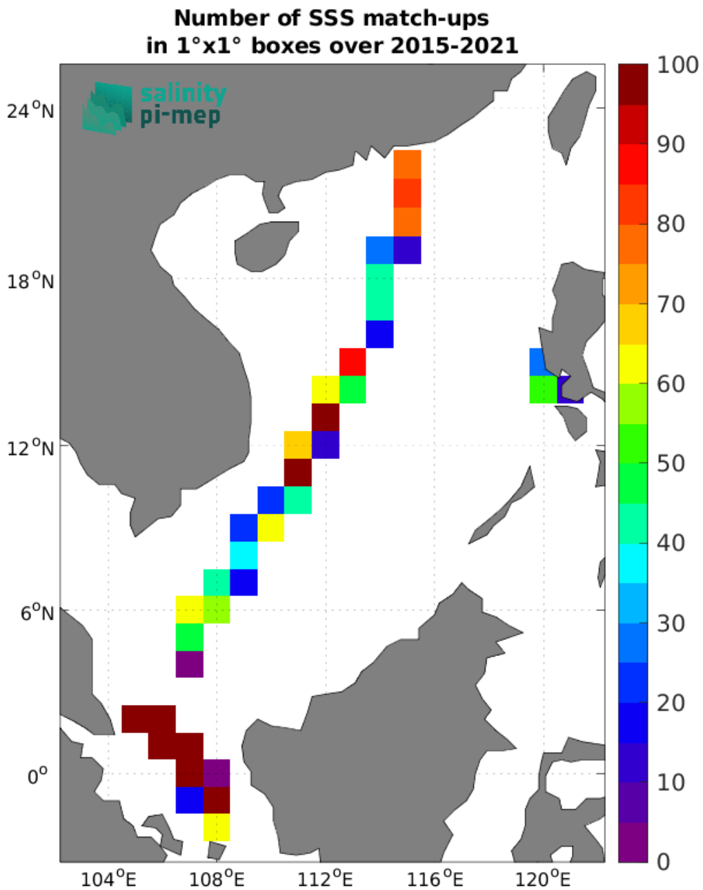
Figure 5: Number of SSS match-ups between TSG (LEGOS-DM) SSS and the SMAP SSS L2 v5.3 (RSS) SSS product for the South China Sea Pi-MEP region over 1^{\circ} \times 1^{\circ} boxes and for the full satellite product period.
