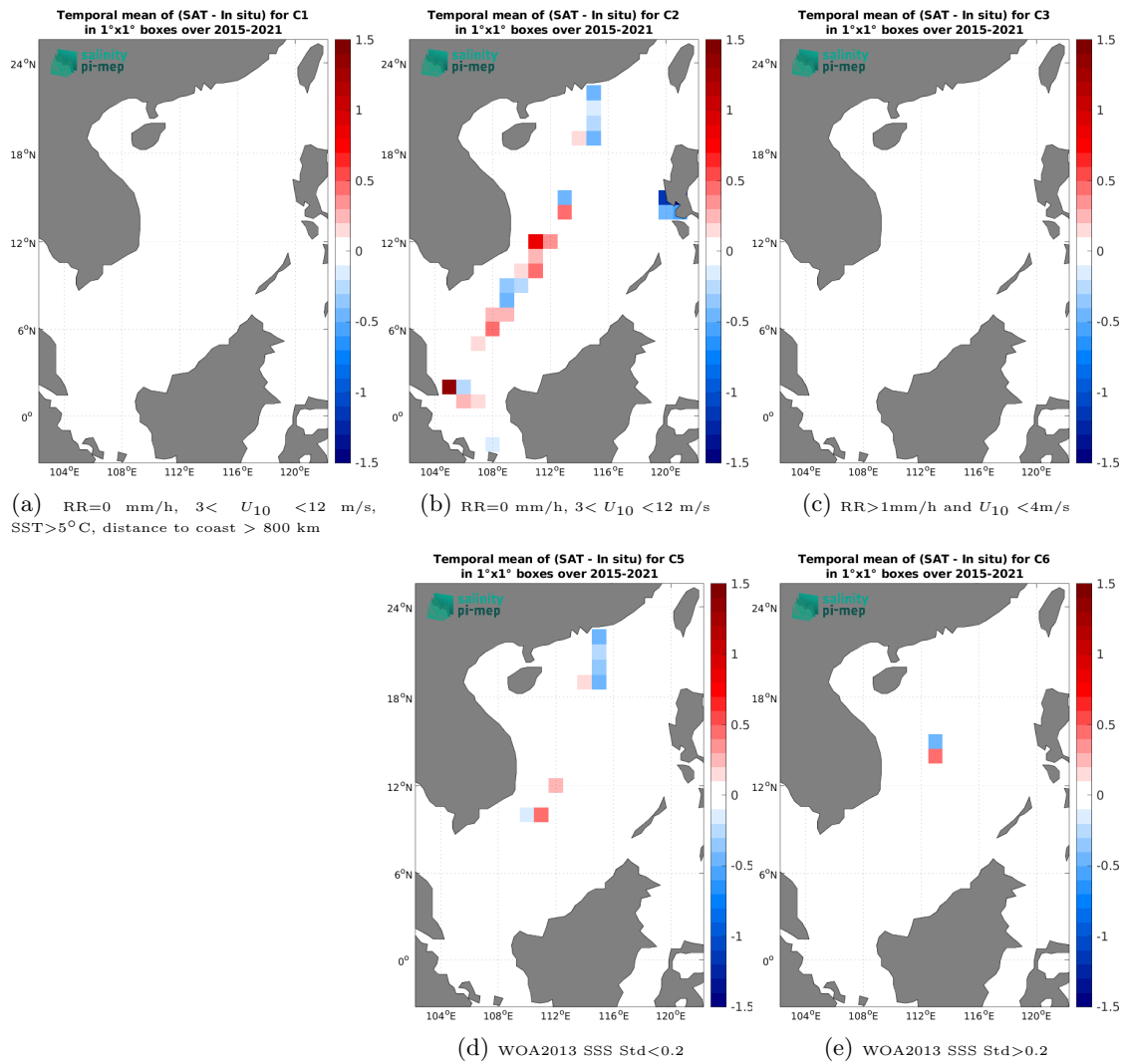
Figure 14: Temporal mean gridded over spatial boxes of size 1^{\circ} \times 1^{\circ} of \Delta SSS (SMAP SSS L2 v5.3 - 40 km (RSS) - TSG (LEGOS-DM)) for 5 different subdatasets corresponding to: RR=0 mm/h, 3 < U_{10} < 12 m/s, SST > 5^{\circ}C , distance to coast > 800 km (a), RR=0 mm/h, 3 < U_{10} < 12 m/s (b), RR > 1 mm/h and U_{10} < 4 m/s (c), WOA2013 SSS Std < 0.2 (d), WOA2013 SSS Std > 0.2 (e).
