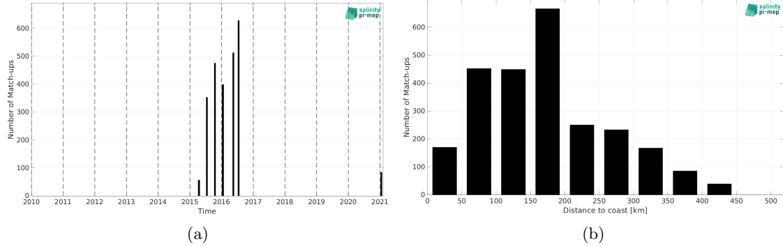
Figure 2: Number of match-ups between TSG (LEGOS-DM) and SMAP SSS L2 v5.3 - 40 km (RSS) SSS as a function of time (a) and as function of the distance to coast (b) over the South China Sea Pi-MEP region and for the full satellite product period.
