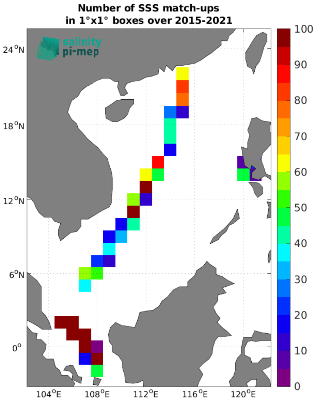
Figure 5: Number of SSS match-ups between TSG (LEGOS-DM) SSS and the SMAP SSS L2 v5.3 - 40 km (RSS) SSS product for the South China Sea Pi-MEP region over 1^{\circ}\times 1^{\circ} boxes and for the full satellite product period.
