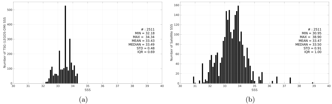
Figure 3: Histograms of SSS from TSG (LEGOS-DM) (a) and SMAP SSS L2 v5.3 - 40 km (RSS) (b) considering all match-up pairs per bins of 0.1 over the South China Sea Pi-MEP region and for the full satellite product period.
