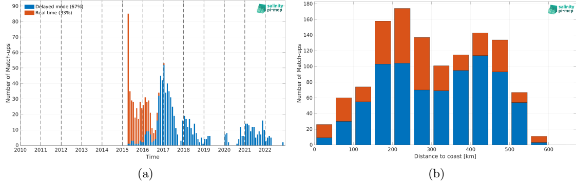
Figure 2: Number of match-ups between Argo and SMAP SSS L2 v5.3 - 40 km (RSS) SSS as a function of time (a) and as function of the distance to coast (b) over the South China Sea Pi-MEP region and for the full satellite product period.
