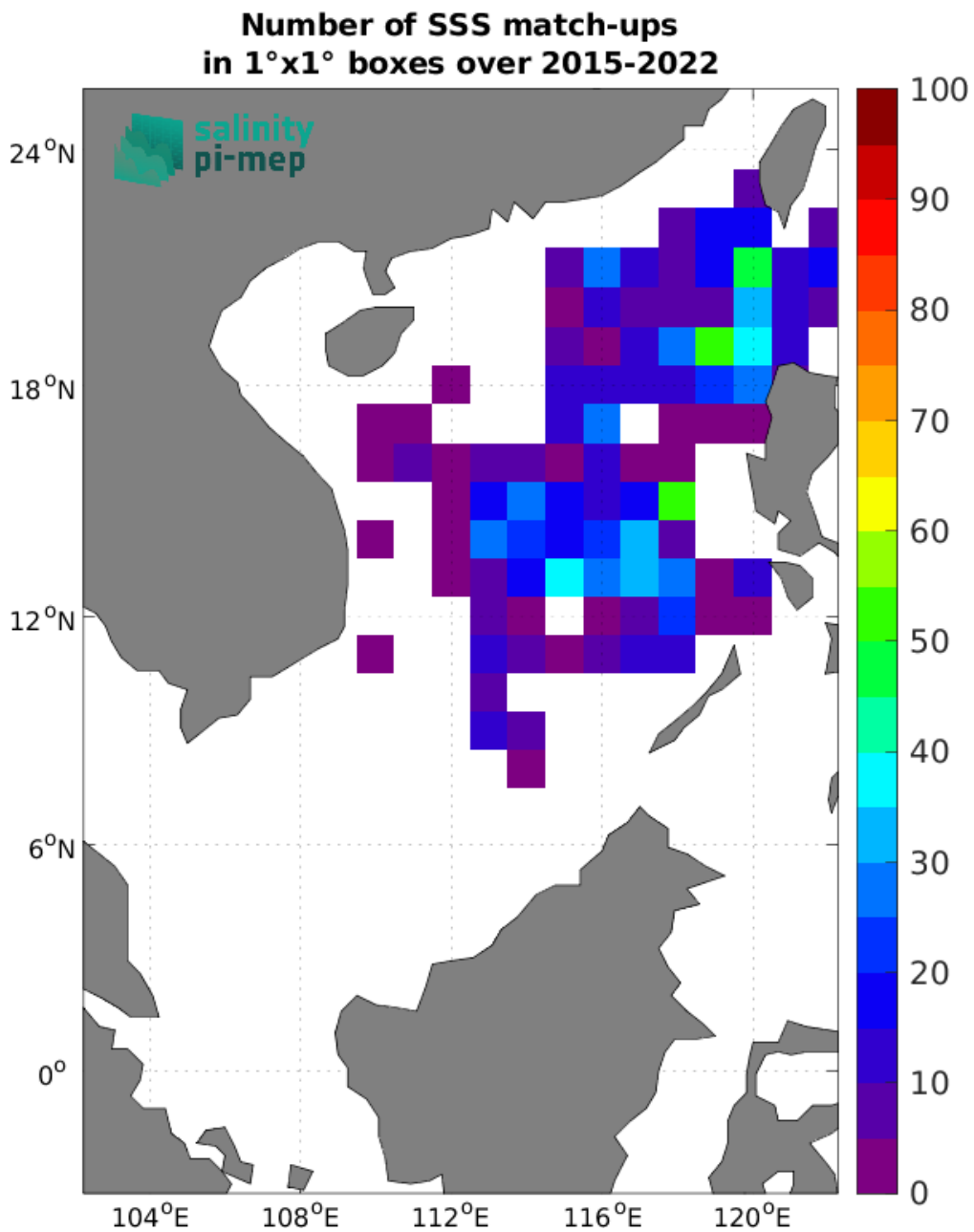
Figure 5: Number of SSS match-ups between Argo SSS and the SMAP SSS L2 v5.3 - 40 km (RSS) SSS product for the South China Sea Pi-MEP region over 1^\circ \times 1^\circ boxes and for the full satellite product period.
