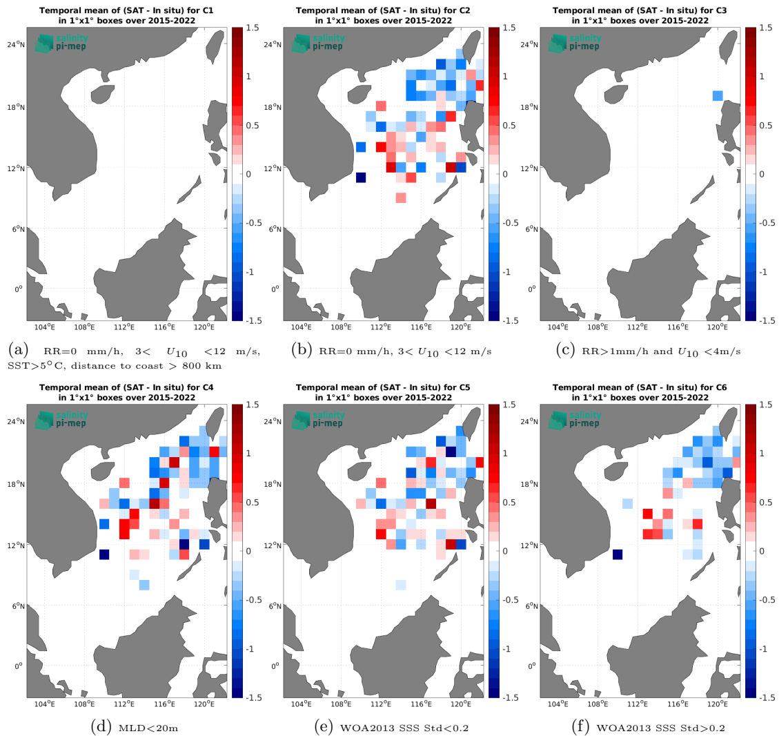
Figure 14: Temporal mean gridded over spatial boxes of size 1^\circ \times 1^\circ of \Delta\text{SSS} (SMAP SSS L2 v5.3 - 40 km (RSS) - Argo) for 6 different subdatasets corresponding to: RR=0 mm/h, 3 < U_{10} < 12 m/s, SST > 5^\circ\text{C} , distance to coast > 800 km (a), RR=0 mm/h, 3 < U_{10} < 12 m/s (b), RR > 1 mm/h and U_{10} < 4 m/s (c), MLD < 20 m (d), WOA2013 SSS Std < 0.2 (e), WOA2013 SSS Std > 0.2 (f).
