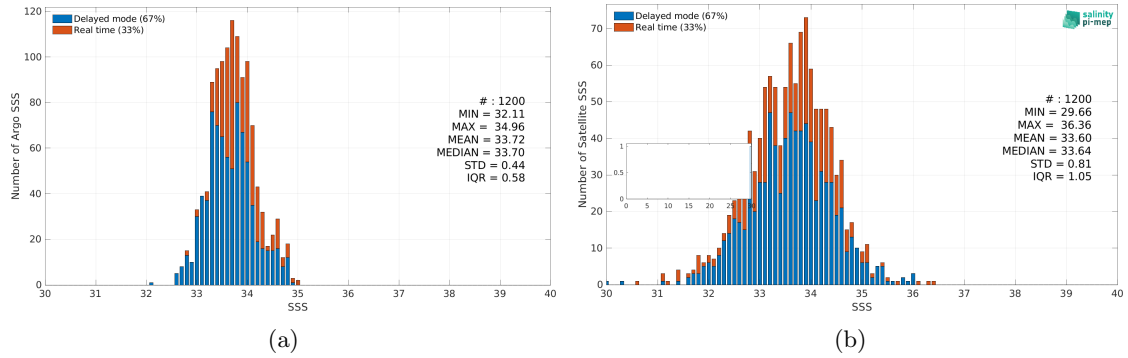
Figure 3: Histograms of SSS from Argo (a) and SMAP SSS L2 v5.3 - 40 km (RSS) (b) considering all match-up pairs per bins of 0.1 over the South China Sea Pi-MEP region and for the full satellite product period.
