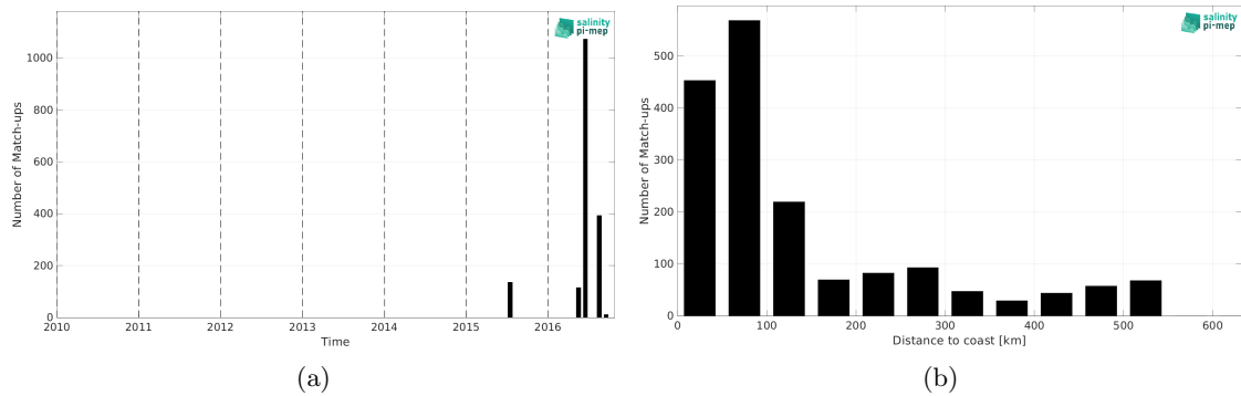
Figure 1: Number of match-ups between TSG (SAMOS) and SMAP SSS L2 v5 - 40 km (RSS) SSS as a function of time (a) and as function of the distance to coast (b) over the South China Sea Pi-MEP region and for the full satellite product period.
