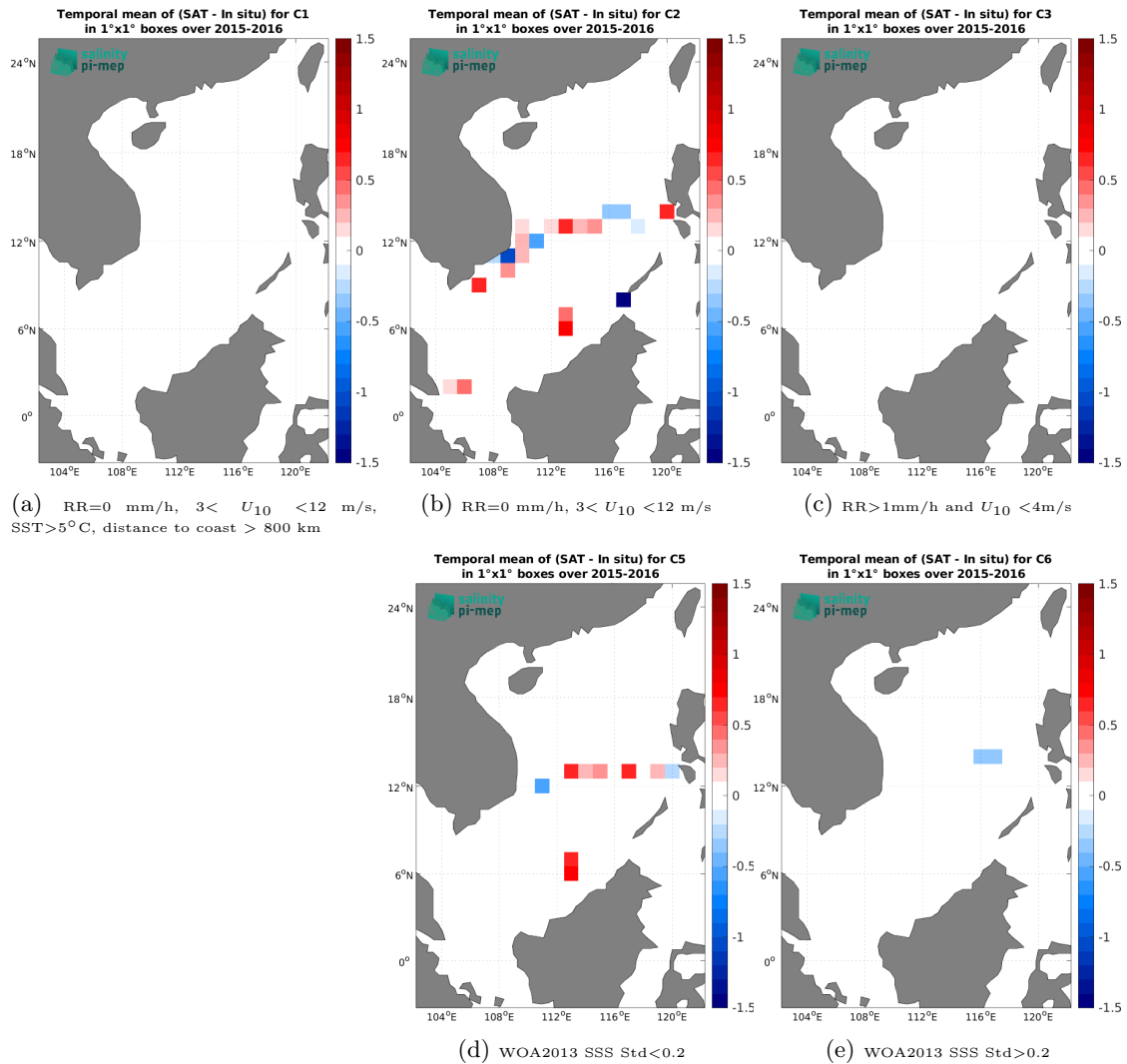
Figure 12: Temporal mean gridded over spatial boxes of size 1^\circ \times 1^\circ of \Delta SSS (SMAP SSS L2 v5 - 40 km (RSS) - TSG (SAMOS)) for 5 different subdatasets corresponding to:RR=0 mm/h, 3 < U_{10} < 12 m/s, SST >5^\circ\text{C} , distance to coast > 800 km (a), RR=0 mm/h, 3 < U_{10} < 12 m/s (b), RR >1 mm/h and U_{10} < 4 m/s (c), WOA2013 SSS Std <0.2 (d), WOA2013 SSS Std >0.2 (e).
