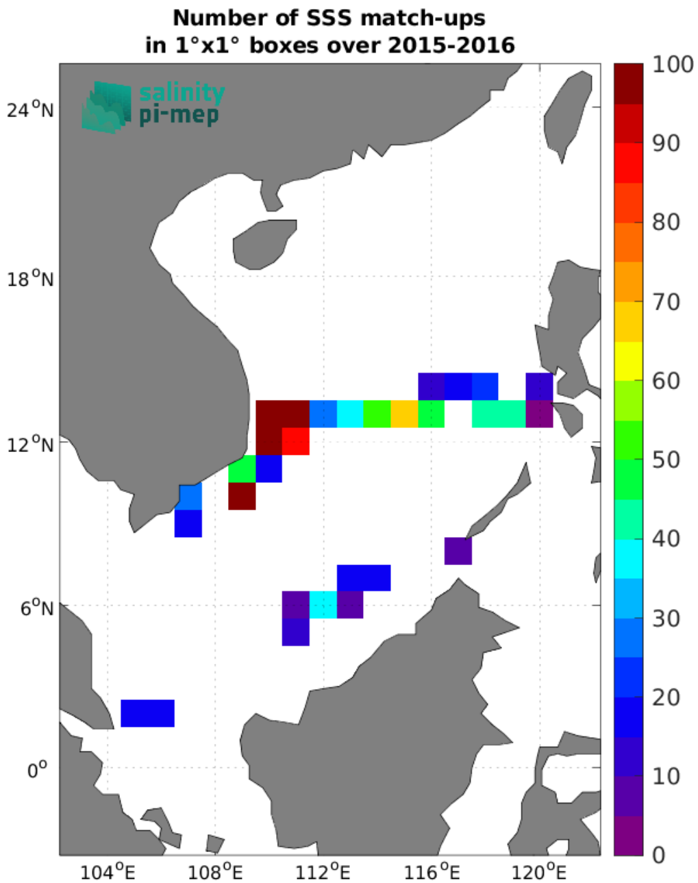
Figure 4: Number of SSS match-ups between TSG (SAMOS) SSS and the SMAP SSS L2 v5 - 40 km (RSS) SSS product for the South China Sea Pi-MEP region over 1°x1° boxes and for the full satellite product period.
