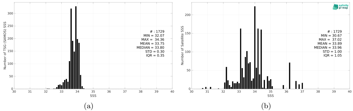
Figure 2: Histograms of SSS from TSG (SAMOS) (a) and SMAP SSS L2 v5 - 40 km (RSS) (b) considering all match-up pairs per bins of 0.1 over the South China Sea Pi-MEP region and for the full satellite product period.
