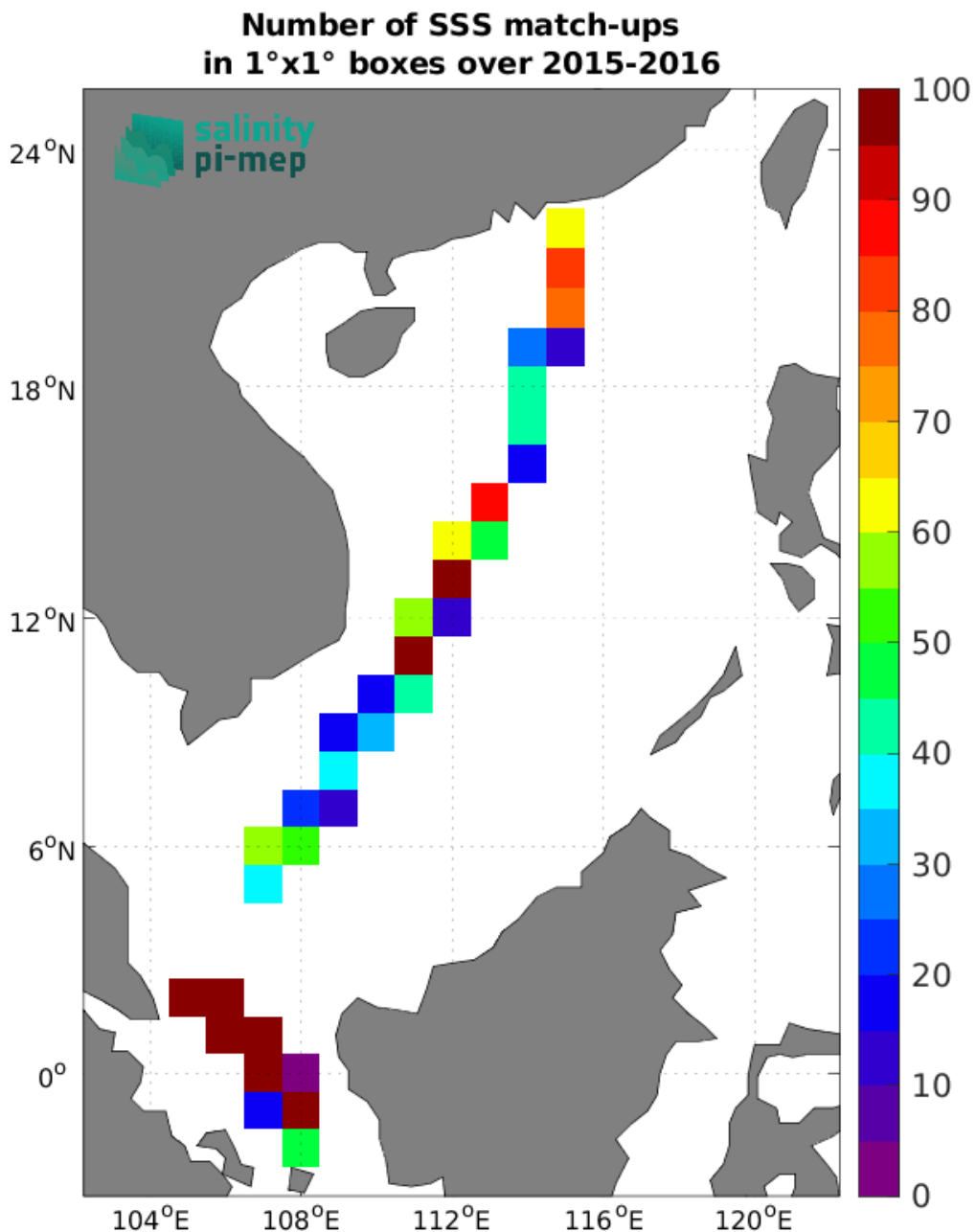
Figure 4: Number of SSS match-ups between TSG (LEGOS-DM) SSS and the SMAP SSS L2 v5 - 40 km (RSS) SSS product for the South China Sea Pi-MEP region over 1^\circ \times 1^\circ boxes and for the full satellite product period.
