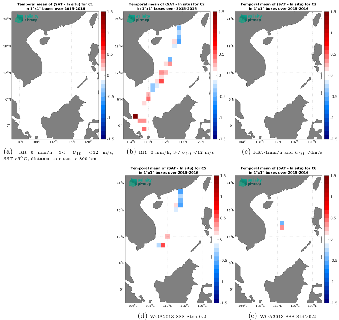
Figure 12: Temporal mean gridded over spatial boxes of size 1^\circ \times 1^\circ of \Delta\text{SSS} (SMAP SSS L2 v5 - 40 km (RSS) - TSG (LEGOS-DM)) for 5 different subdatasets corresponding to:RR=0 mm/h, 3 < U_{10} < 12 m/s, SST >5^\circ\text{C} , distance to coast > 800 km (a), RR=0 mm/h, 3 < U_{10} < 12 m/s (b), RR >1 mm/h and U_{10} < 4 m/s (c), WOA2013 SSS Std <0.2 (d), WOA2013 SSS Std >0.2 (e).
