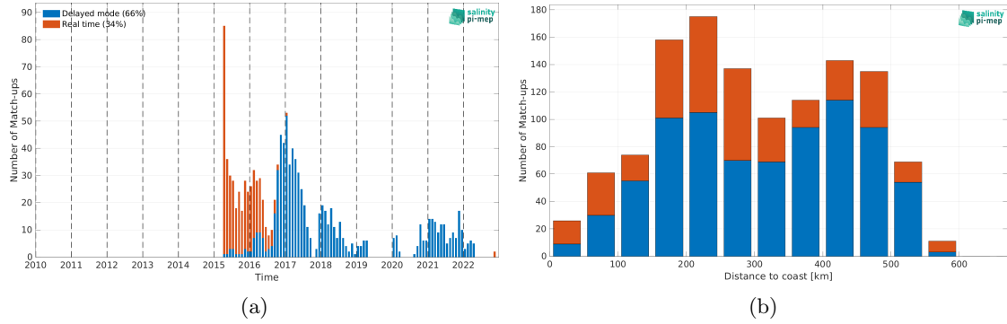
Figure 1: Number of match-ups between Argo and SMAP SSS L2 v5 - 40 km (RSS) SSS as a function of time (a) and as function of the distance to coast (b) over the South China Sea Pi-MEP region and for the full satellite product period.
