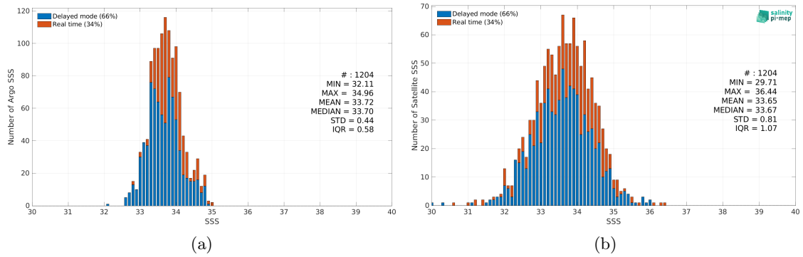
Figure 2: Histograms of SSS from Argo (a) and SMAP SSS L2 v5 - 40 km (RSS) (b) considering all match-up pairs per bins of 0.1 over the South China Sea Pi-MEP region and for the full satellite product period.
