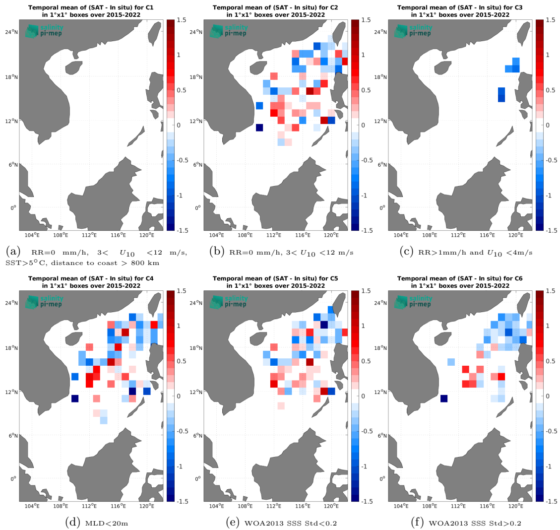
Figure 12: Temporal mean gridded over spatial boxes of size 1^\circ \times 1^\circ of \Delta SSS (SMAP SSS L2 v5 - 40 km (RSS) - Argo) for 6 different subdatasets corresponding to: RR=0 mm/h, 3 < U_{10} < 12 m/s, SST > 5°C, distance to coast > 800 km (a), RR=0 mm/h, 3 < U_{10} < 12 m/s (b), RR > 1mm/h and U_{10} < 4 m/s (c), MLD < 20m (d), WOA2013 SSS Std < 0.2 (e), WOA2013 SSS Std > 0.2 (f).
