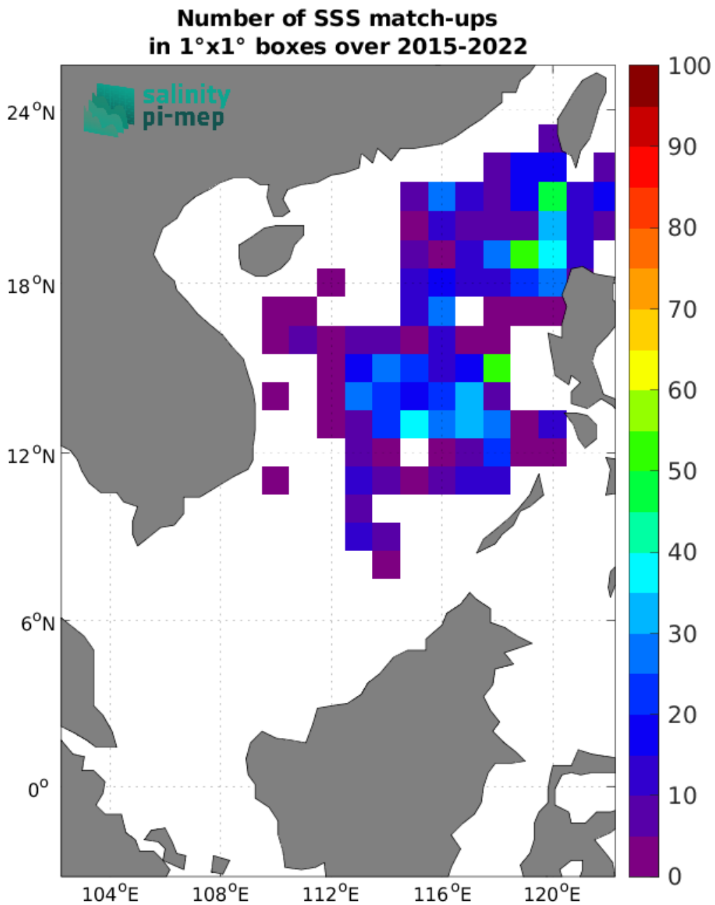
Figure 4: Number of SSS match-ups between Argo SSS and the SMAP SSS L2 v5 - 40 km (RSS) SSS product for the South China Sea Pi-MEP region over 1°×1° boxes and for the full satellite product period.
