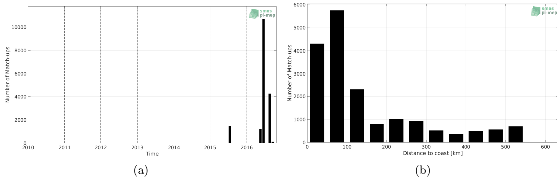
Figure 1: Number of match-ups between TSG (SAMOS) and SMAP SSS L2 v4 (RSS) SSS as a function of time (a) and as function of the distance to coast (b) over the South China Sea Pi-MEP region and for the full satellite product period.
