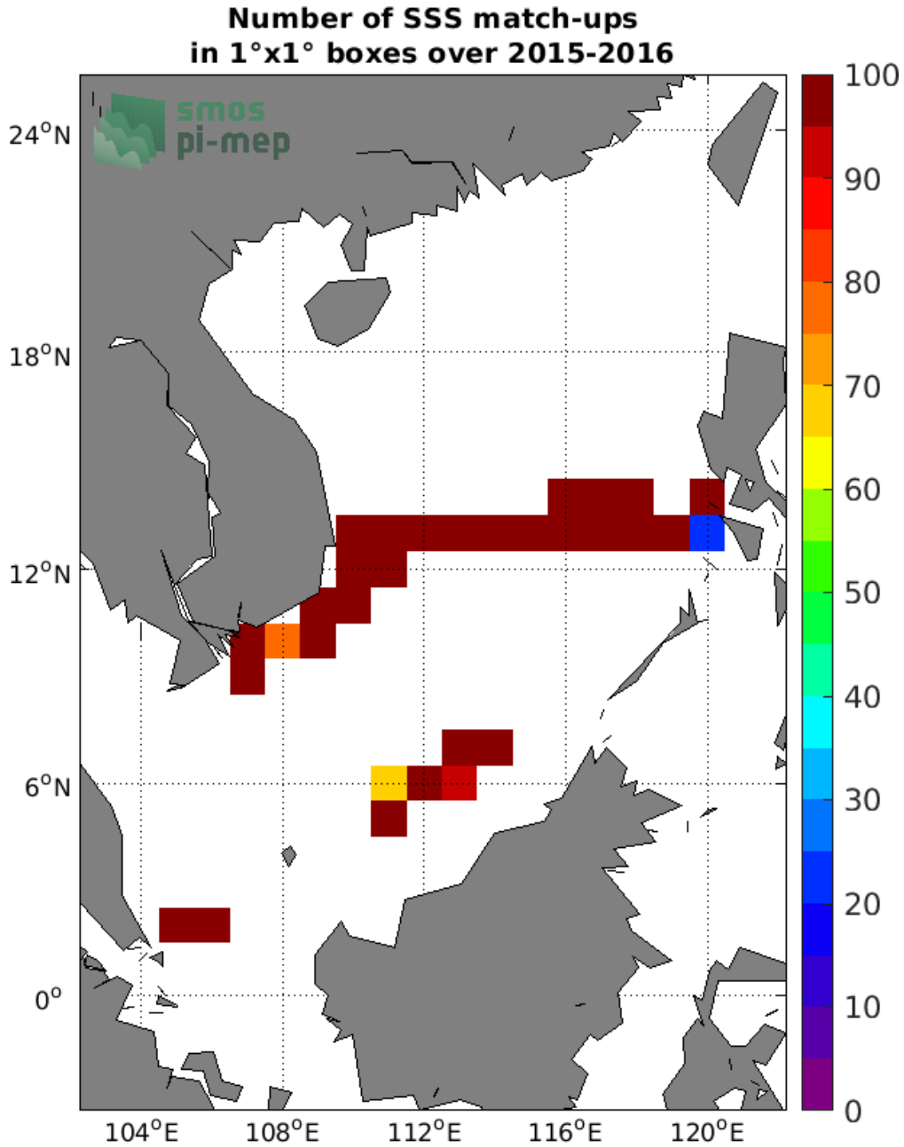
Figure 4: Number of SSS match-ups between TSG (SAMOS) SSS and the SMAP SSS L2 v4 (RSS) SSS product for the South China Sea Pi-MEP region over 1^{\circ} \times 1^{\circ} boxes and for the full satellite product period.
