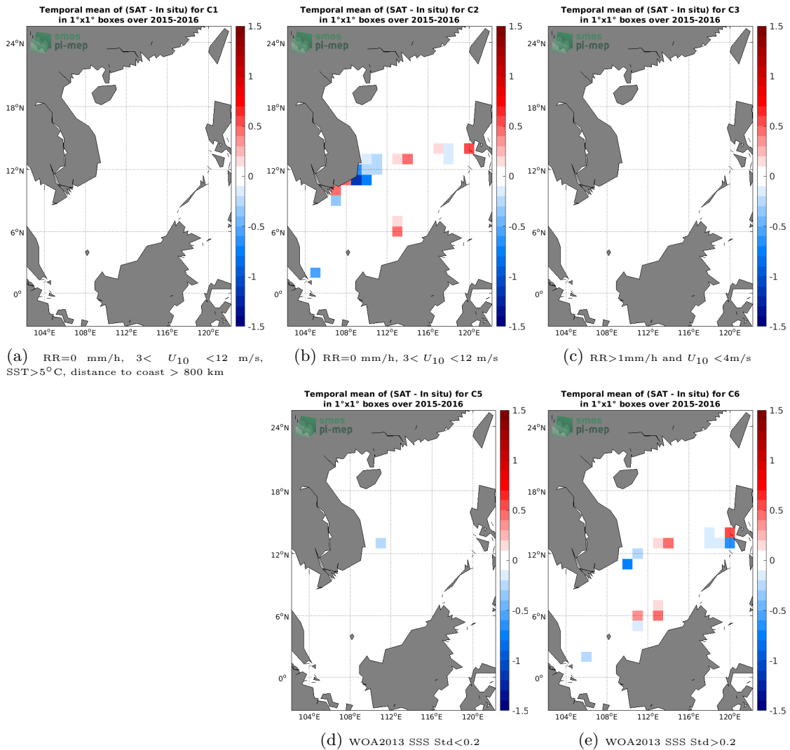
Figure 12: Temporal mean gridded over spatial boxes of size 1^\circ \times 1^\circ of \Delta SSS (SMAP SSS L2 v4 (RSS) - TSG (SAMOS)) for 5 different subdatasets corresponding to:RR=0 mm/h, 3 < U_{10} < 12 m/s, SST > 5°C, distance to coast > 800 km (a), RR=0 mm/h, 3 < U_{10} < 12 m/s (b), RR > 1mm/h and U_{10} < 4 m/s (c), WOA2013 SSS Std < 0.2 (d), WOA2013 SSS Std > 0.2 (e).
