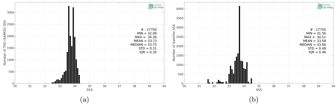
Figure 2: Histograms of SSS from TSG (SAMOS) (a) and SMAP SSS L2 v4 (RSS) (b) considering all match-up pairs per bins of 0.1 over the South China Sea Pi-MEP region and for the full satellite product period.
