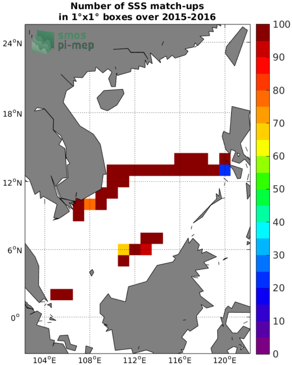
Figure 4: Number of SSS match-ups between TSG (SAMOS) SSS and the SMAP SSS L2 v4 (RSS) SSS product for the South China Sea Pi-MEP region over 1°x1° boxes and for the full satellite product period.
