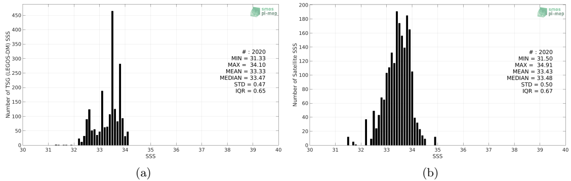
Figure 2: Histograms of SSS from TSG (LEGOS-DM) (a) and SMAP SSS L2 v4 (RSS) (b) considering all match-up pairs per bins of 0.1 over the South China Sea Pi-MEP region and for the full satellite product period.
