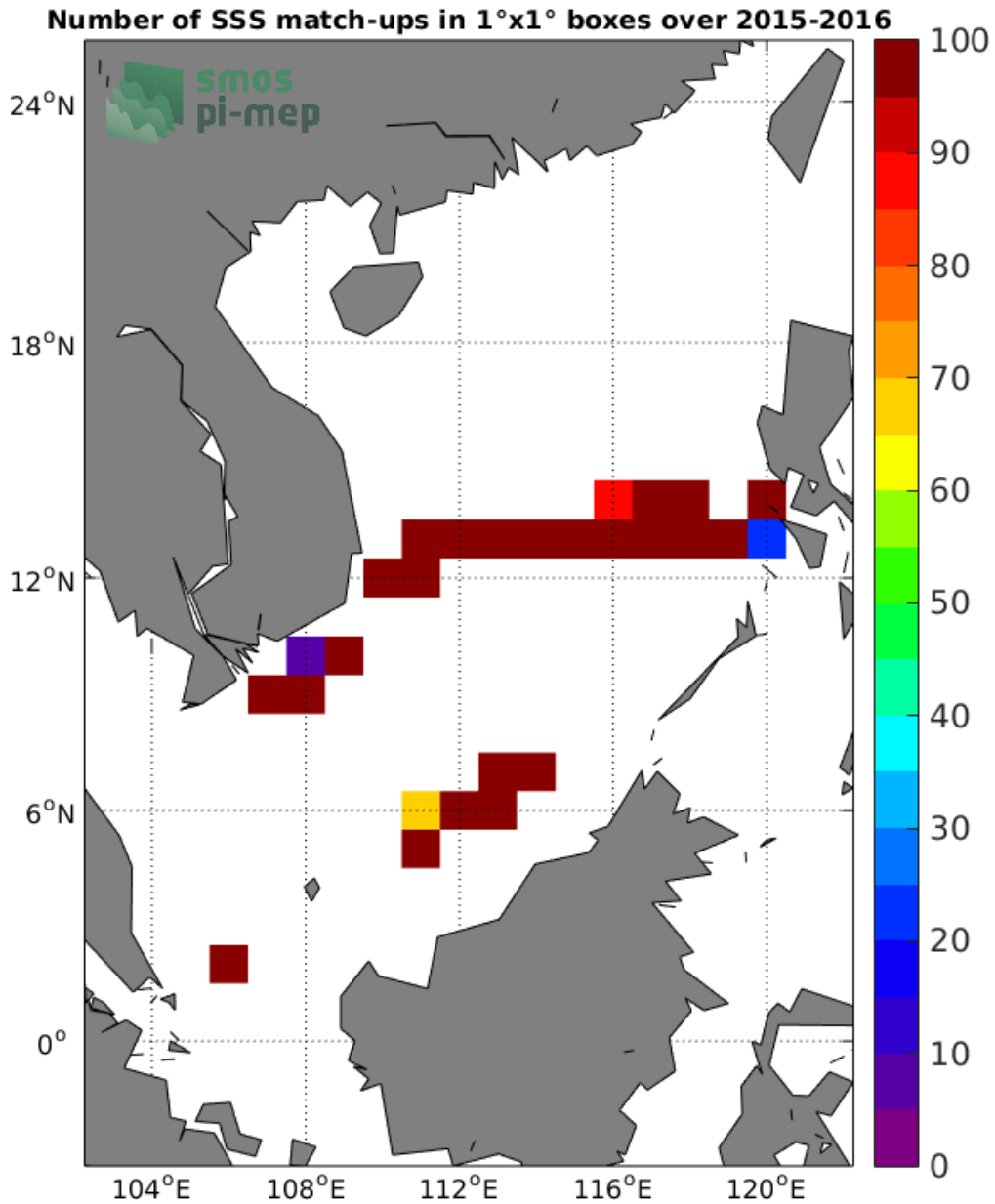
Figure 4: Number of SSS match-ups between TSG-SAMOS SSS and the SMAP-L2-RSS-V3-70KM SSS product for the South China Sea Pi-MEP region over 1°x1° boxes and for the full satellite product period.
