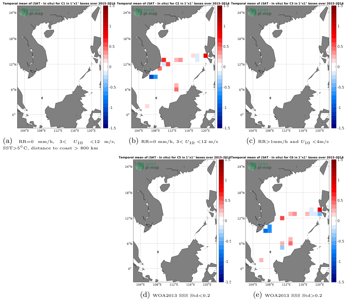
Figure 12: Temporal mean gridded over spatial boxes of size 1^\circ \times 1^\circ of \Delta SSS (SMAP-L2-RSS-V3-70KM - TSG-SAMOS) for 5 different subdatasets corresponding to: RR=0 mm/h, 3 < U_{10} < 12 m/s, SST > 5^\circ C , distance to coast > 800 km (a), RR=0 mm/h, 3 < U_{10} < 12 m/s (b), RR > 1 mm/h and U_{10} < 4 m/s (c), WOA2013 SSS Std < 0.2 (d), WOA2013 SSS Std > 0.2 (e).
