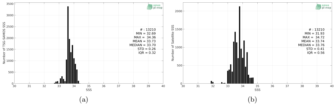
Figure 2: Histograms of SSS from TSG-SAMOS (a) and SMAP-L2-RSS-V3-70KM (b) considering all match-up pairs per bins of 0.1 over the South China Sea Pi-MEP region and for the full satellite product period.
