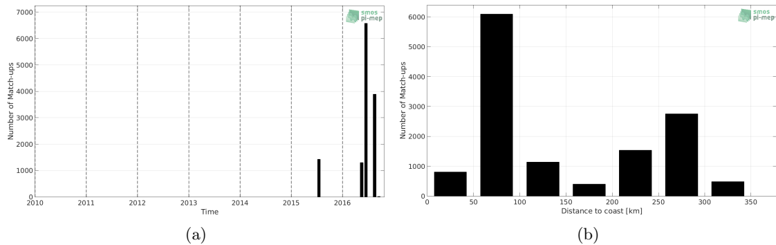
Figure 1: Number of match-ups between TSG-SAMOS and SMAP-L2-RSS-V3-70KM SSS as a function of time (a) and as function of the distance to coast (b) over the South China Sea Pi-MEP region and for the full satellite product period.
