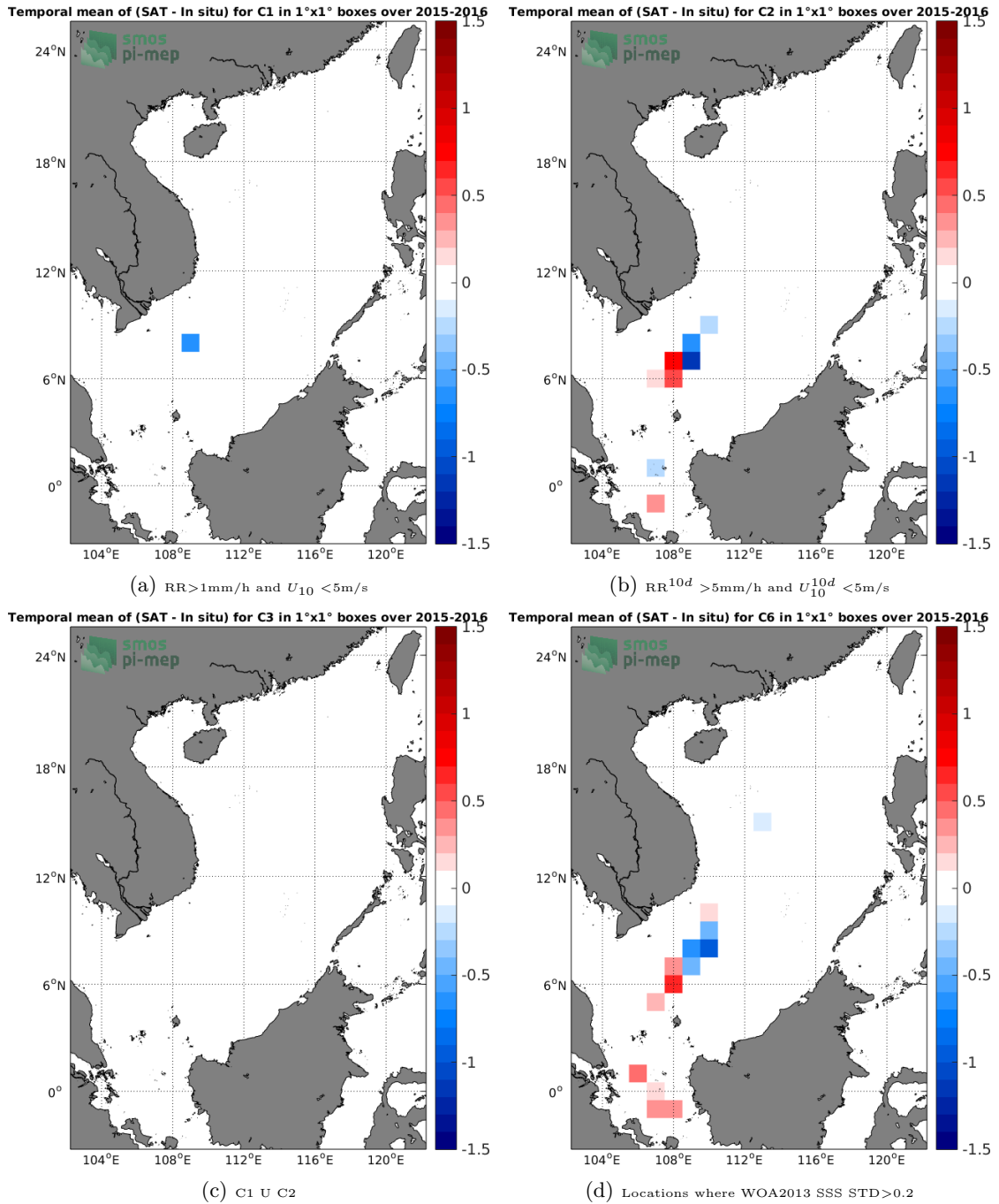
Figure 12: Temporal mean gridded over spatial boxes of size 1°x1° of \Delta\text{SSS} (SMAP-L2-RSS-V3-70KM - TSG-LEGOS-DM) for 4 different subdatasets corresponding to: RR > 1\text{mm/h} and U_{10} < 5\text{m/s} (a), RR^{10d} > 5\text{mm/h} and U_{10}^{10d} < 5\text{m/s} (b), C1 U C2 (c), Locations where WOA2013 SSS STD > 0.2 (d).
