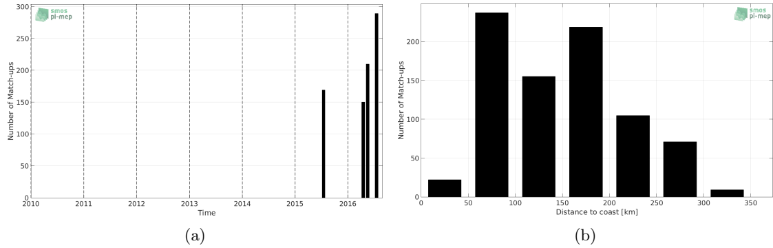
Figure 1: Number of match-ups between TSG-LEGOS-DM and SMAP-L2-RSS-V3-70KM SSS as a function of time (a) and as function of the distance to coast (b) over the South China Sea Pi-MEP region and for the full satellite product period.
