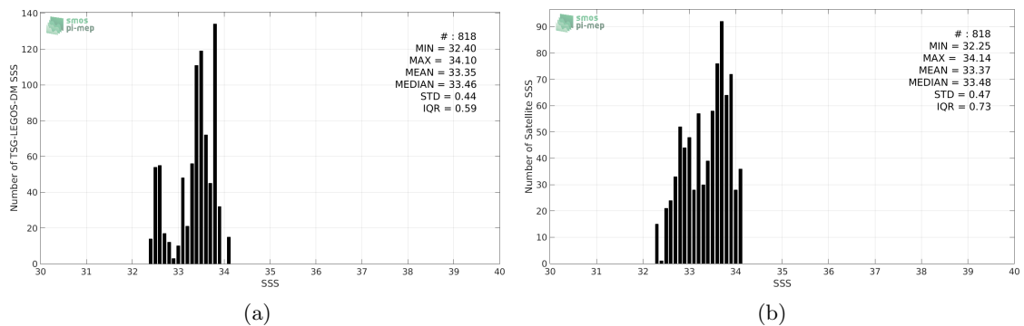
Figure 2: Histograms of SSS from TSG-LEGOS-DM (a) and SMAP-L2-RSS-V3-70KM (b) considering all match-up pairs per bins of 0.1 over the South China Sea Pi-MEP region and for the full satellite product period.
