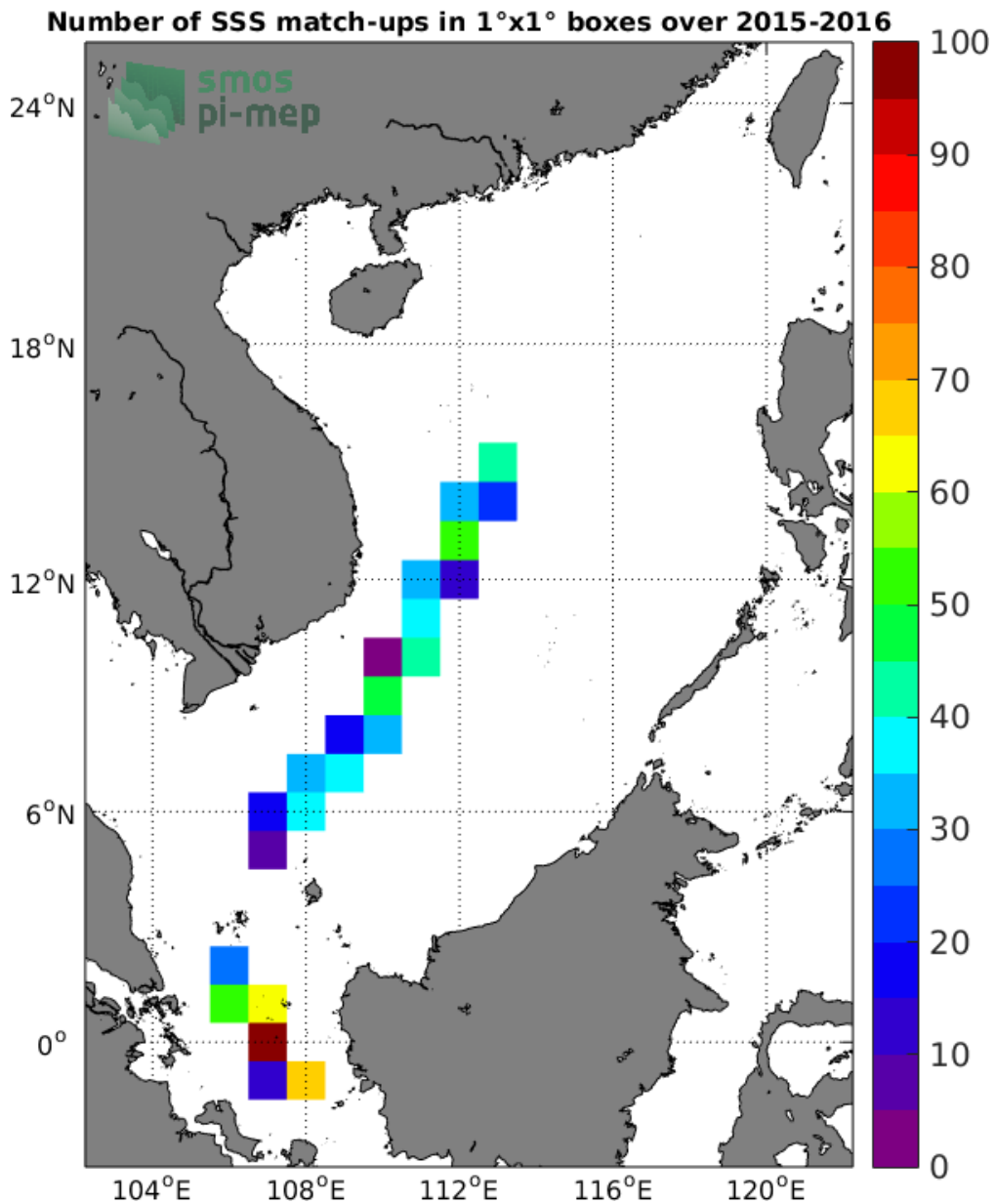
Figure 4: Number of SSS match-ups between TSG-LEGOS-DM SSS and the SMAP-L2-RSS-V3-70KM SSS product for the South China Sea Pi-MEP region over 1°x1° boxes and for the full satellite product period.
