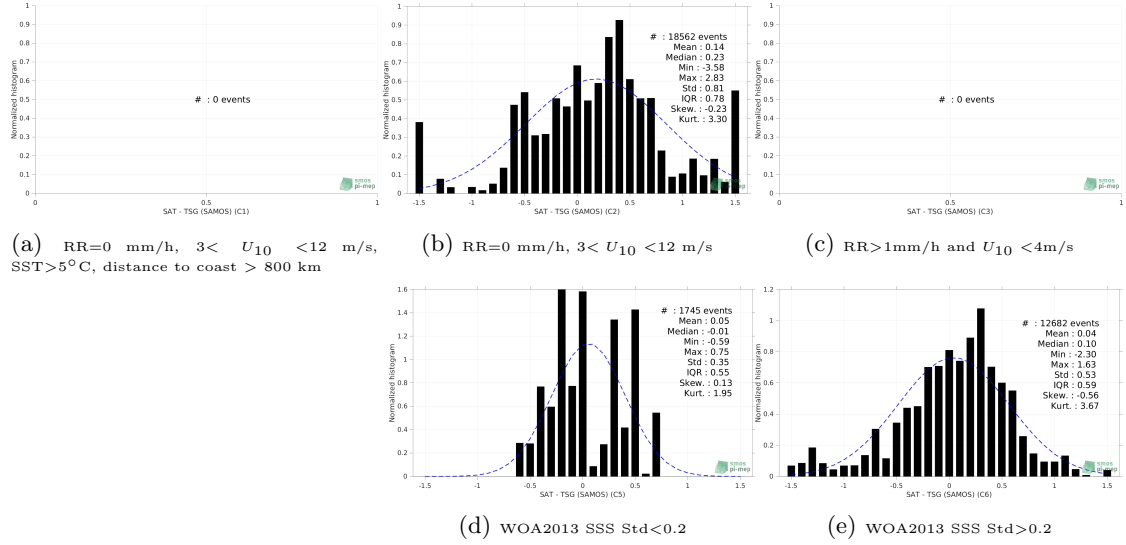
Figure 13: Normalized histogram of \Delta SSS (SMAP SSS L2 v5.0 (JPL) - TSG (SAMOS)) for 5 different subdatasets corresponding to: RR=0 mm/h, 3 < U_{10} < 12 m/s, SST > 5°C, distance to coast > 800 km (a), RR=0 mm/h, 3 < U_{10} < 12 m/s (b), RR > 1mm/h and U_{10} < 4 m/s (c), WOA2013 SSS Std < 0.2 (d), WOA2013 SSS Std > 0.2 (e).
