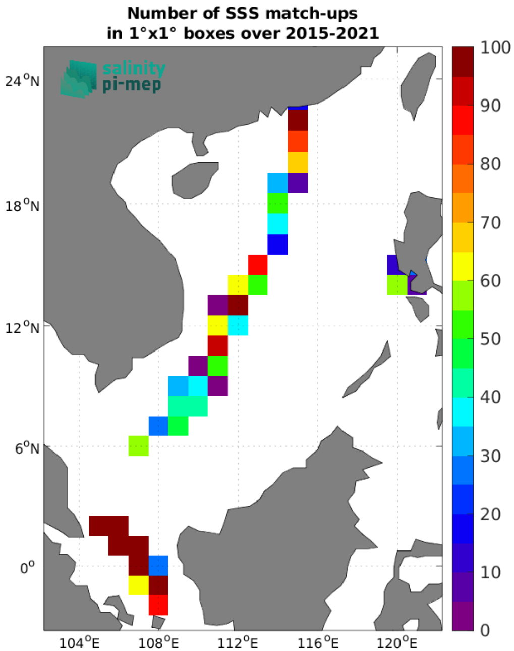
Figure 5: Number of SSS match-ups between TSG (LEGOS-DM) SSS and the SMAP SSS L2 v5.0 (JPL) SSS product for the South China Sea Pi-MEP region over 1°x1° boxes and for the full satellite product period.
