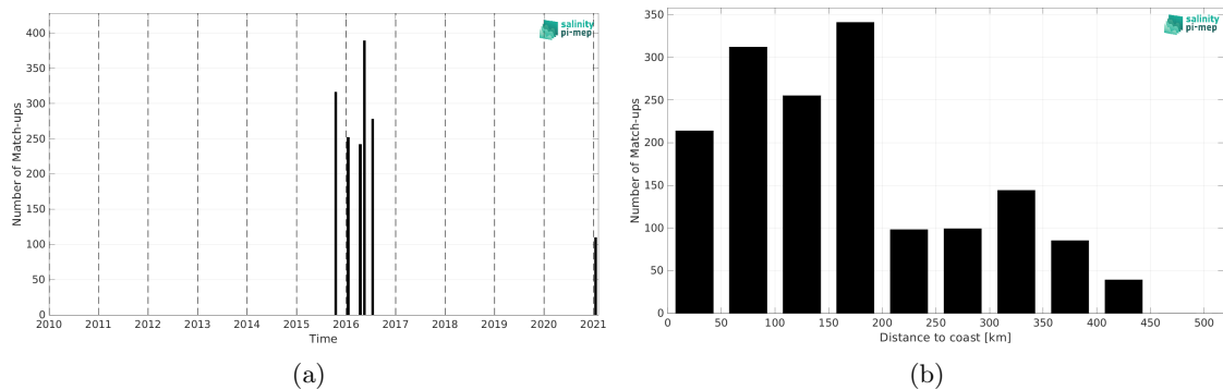
Figure 2: Number of match-ups between TSG (LEGOS-DM) and SMAP SSS L2 v5.0 (JPL) SSS as a function of time (a) and as function of the distance to coast (b) over the South China Sea Pi-MEP region and for the full satellite product period.
