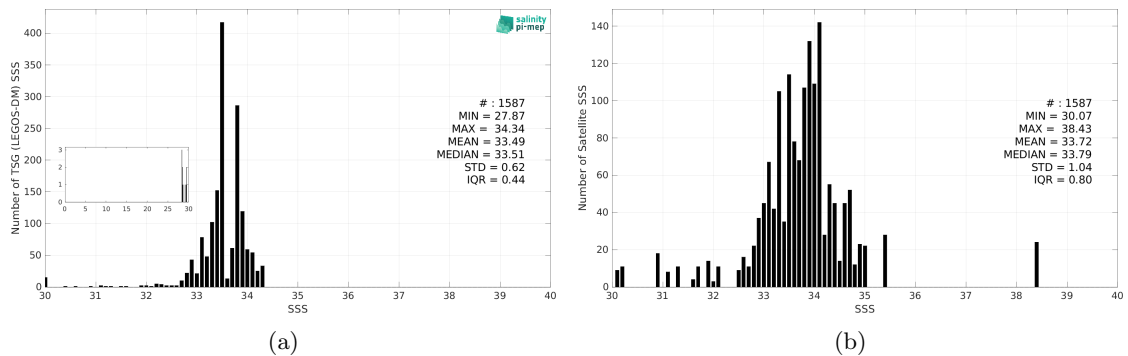
Figure 3: Histograms of SSS from TSG (LEGOS-DM) (a) and SMAP SSS L2 v5.0 (JPL) (b) considering all match-up pairs per bins of 0.1 over the South China Sea Pi-MEP region and for the full satellite product period.
