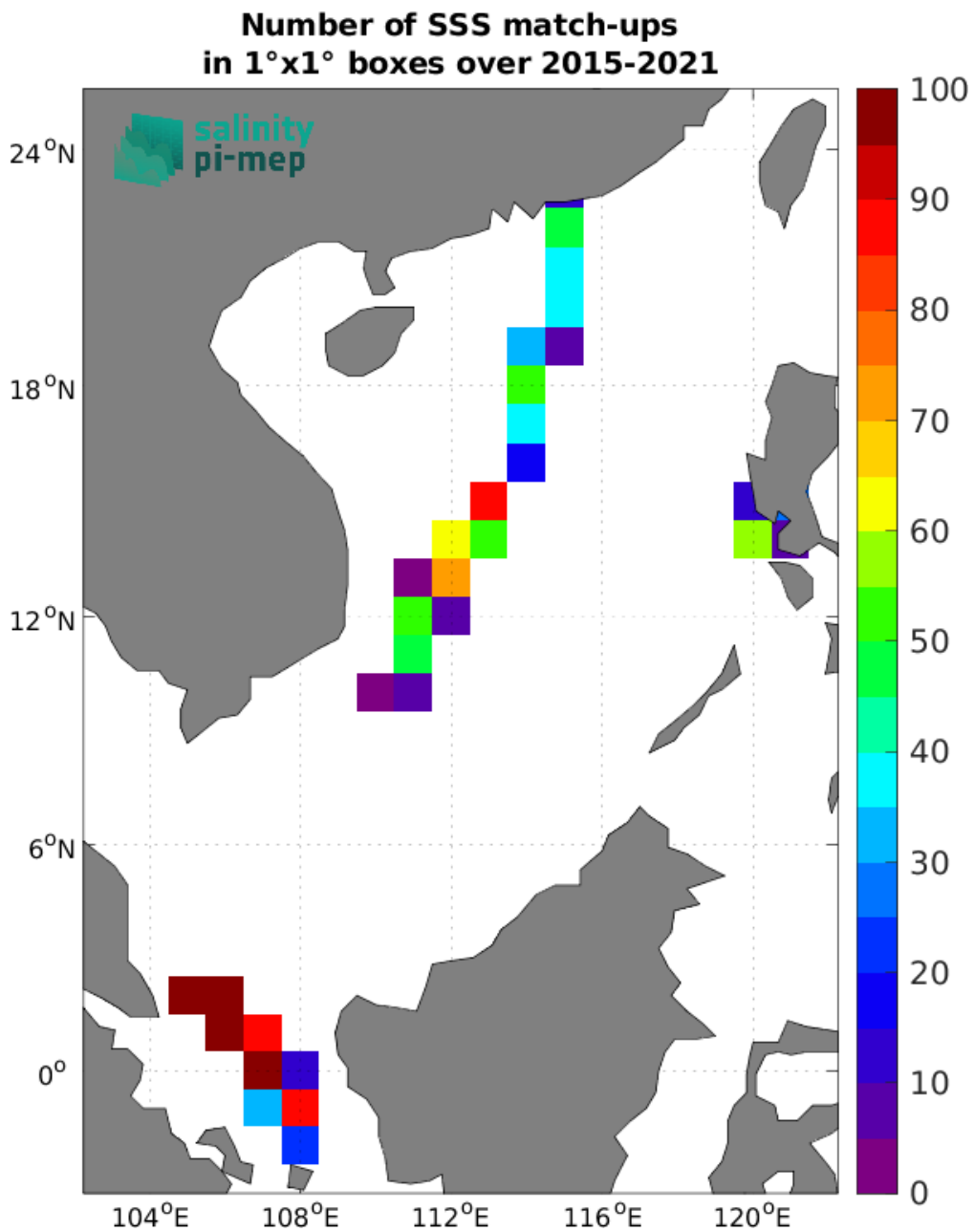
Figure 5: Number of SSS match-ups between TSG (LEGOS-DM) SSS and the SMAP SSS L2 v5.0 (JPL) SSS product for the South China Sea Pi-MEP region over 1^\circ \times 1^\circ boxes and for the full satellite product period.
