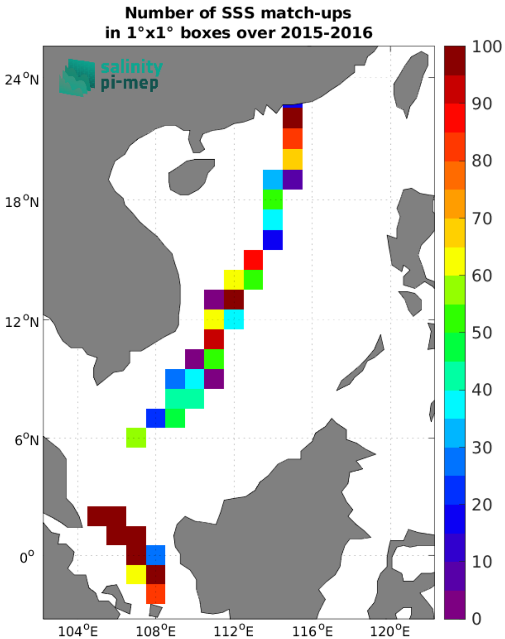
Figure 4: Number of SSS match-ups between TSG (LEGOS-DM) SSS and the SMAP SSS L2 v5.0 (JPL) SSS product for the South China Sea Pi-MEP region over 1^{\circ} \times 1^{\circ} boxes and for the full satellite product period.
