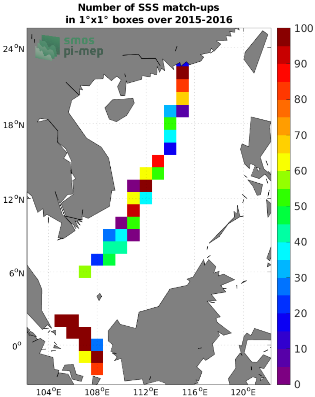
Figure 4: Number of SSS match-ups between TSG (LEGOS-DM) SSS and the SMAP SSS L2 v5.0 (JPL) SSS product for the South China Sea Pi-MEP region over 1^\circ \times 1^\circ boxes and for the full satellite product period.
