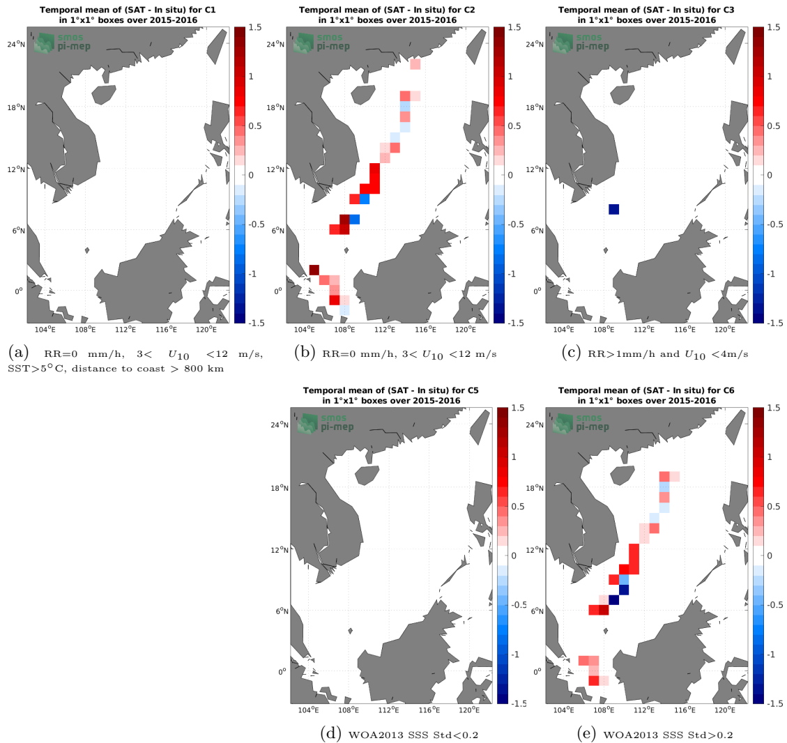
Figure 12: Temporal mean gridded over spatial boxes of size 1^\circ \times 1^\circ of \Delta SSS (SMAP SSS L2 v5.0 (JPL) - TSG (LEGOS-DM)) for 5 different subdatasets corresponding to:RR=0 mm/h, 3 < U_{10} < 12 m/s, SST>5°C, distance to coast > 800 km (a), RR=0 mm/h, 3 < U_{10} < 12 m/s (b), RR>1mm/h and U_{10} < 4 m/s (c), WOA2013 SSS Std<0.2 (d), WOA2013 SSS Std>0.2 (e).
